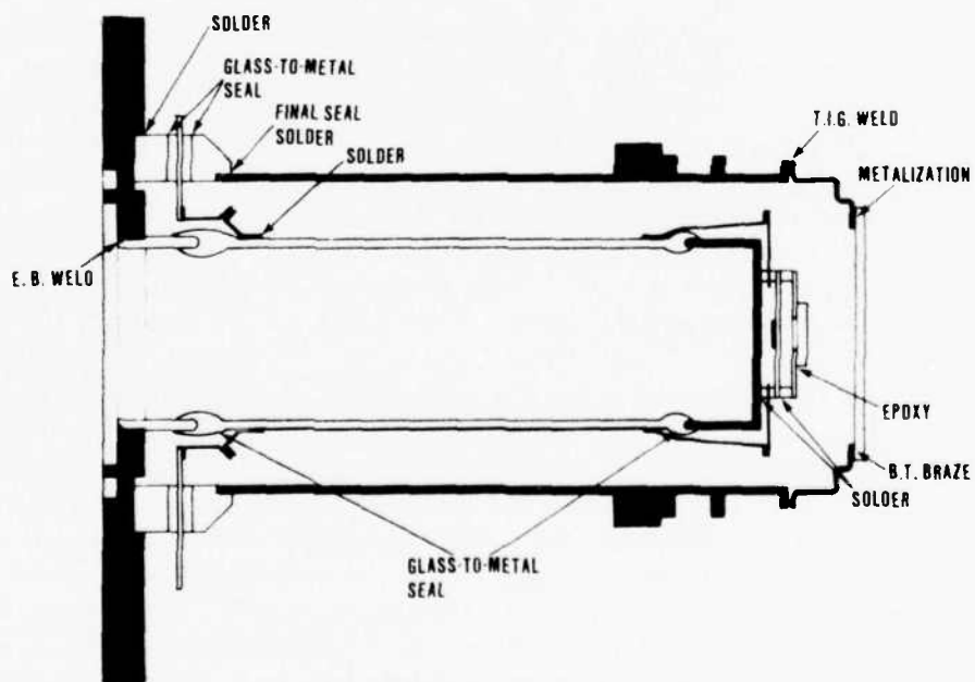
Fig. 35. Dewar fabrication.
