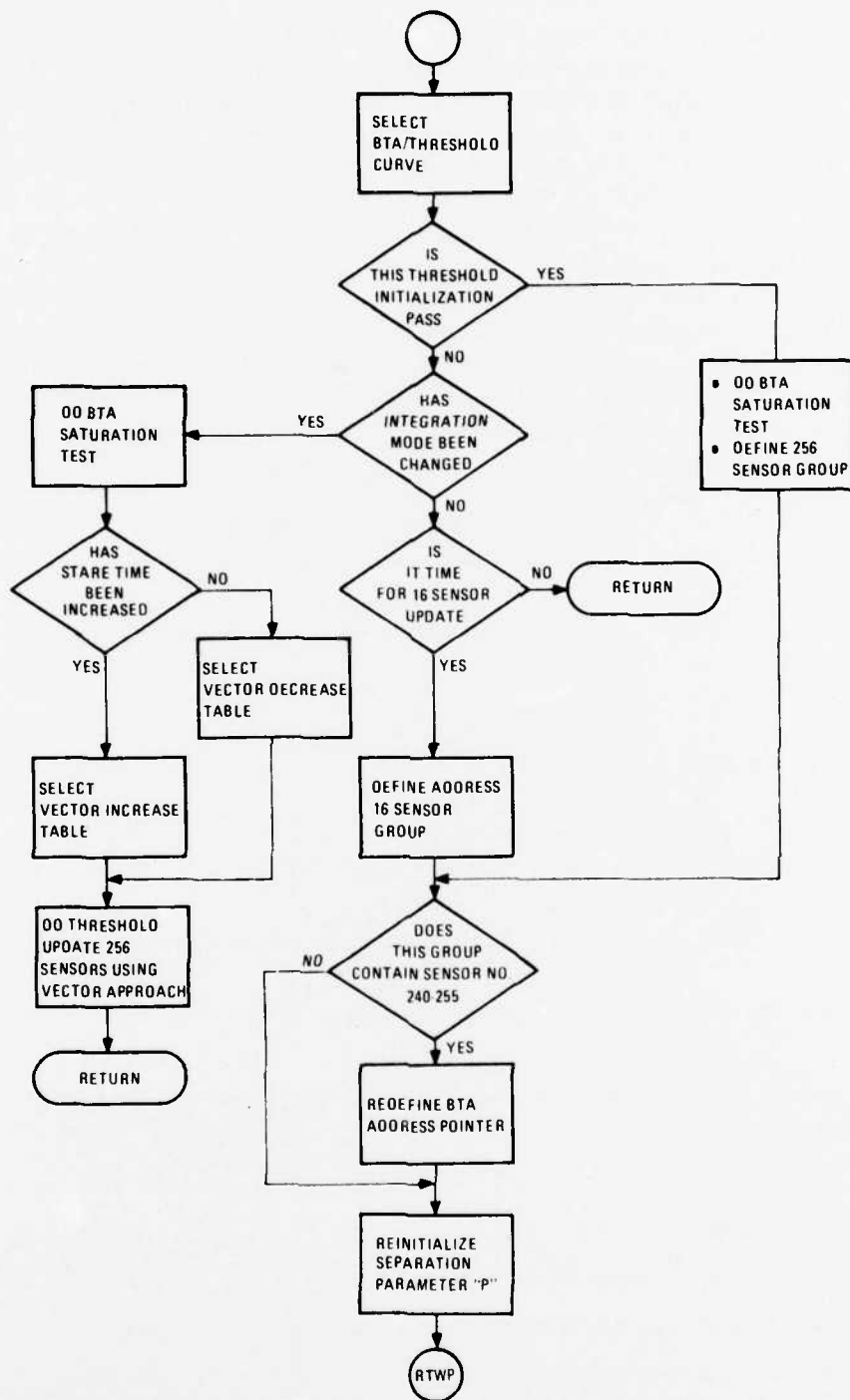
Fig. 42. Threshold routine.
