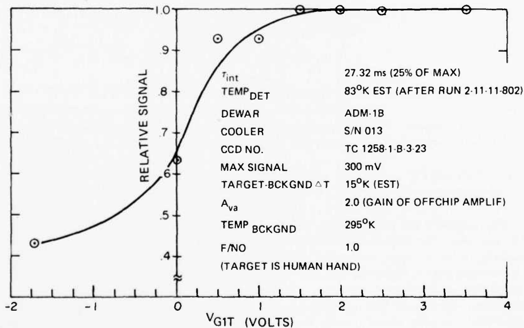
Fig. 17. Relative signal response vs. V_{G1T} at 25% integration.
