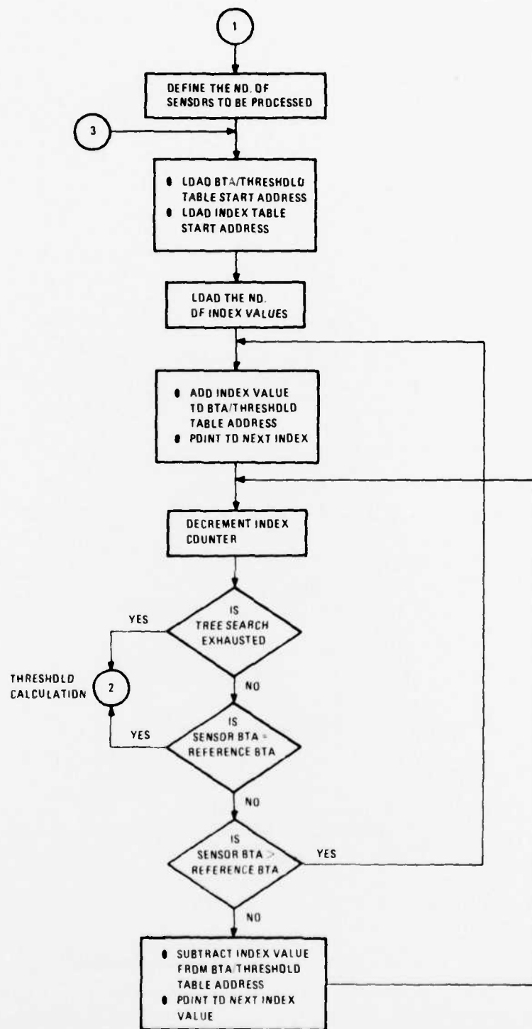
Fig. 41. Binary tree search approach (sheet 1 of 2).
