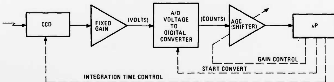
Fig. 40. System configuration with automatic level control.
