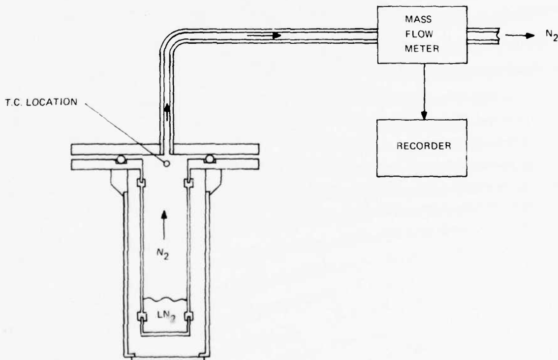
Fig. 36. Arrangement used in liquid nitrogen boiloff test to determine dewar heat load.
