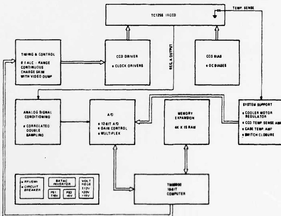
Fig. 2. Sensor Unit electronics block diagram (ADM-1).
