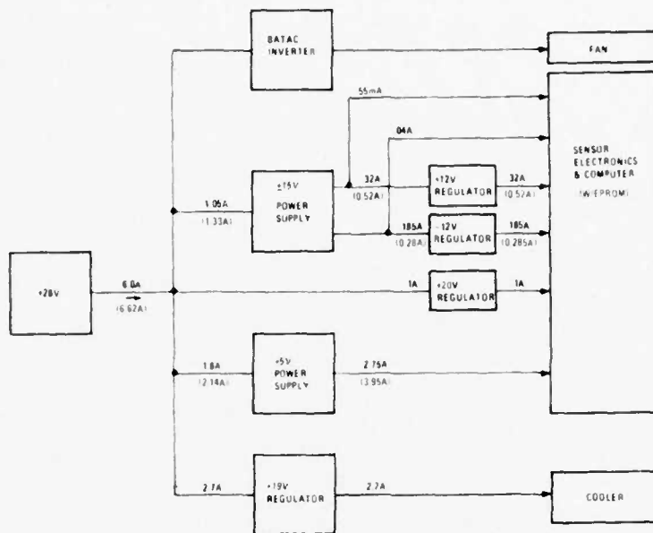
Fig. 8. Modified power flow diagram (parentheses enclose values of current with EPROM expansion board).
