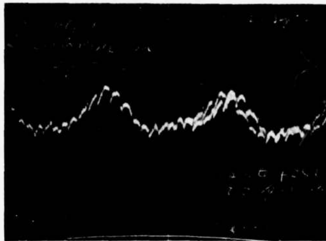
Fig. 13. Cooler compressor-induced noise at the input to the A/D converter prior to separating the input power lines in the ADM-1 sensor unit.
