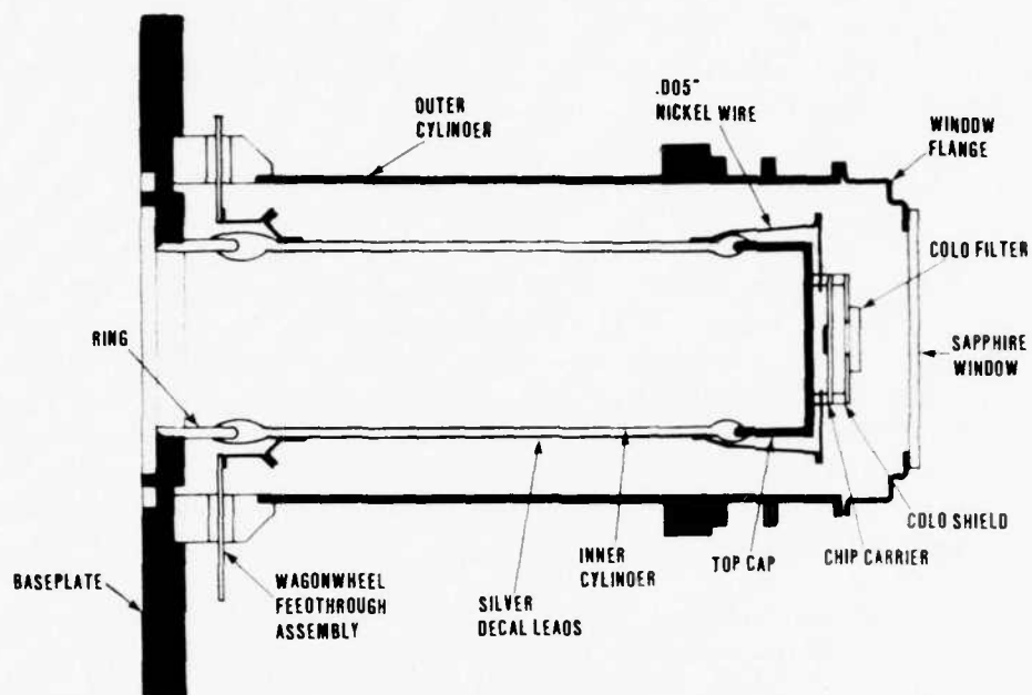
Fig. 34. Dewar components.
