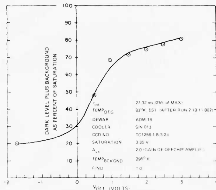
Fig. 15. Dark level plus background vs. V_{G1T} at 25% integration.
