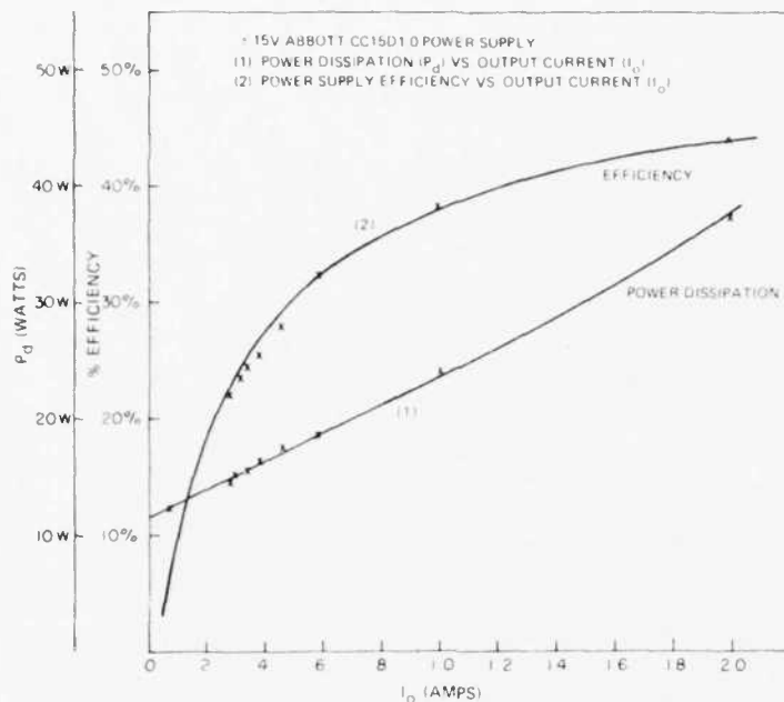
Fig. 10. Power dissipation vs. output current ( I_o ) of Abbott Transistor Labs Model CC15D1.0 power supply ( \pm 15 -V, 1.0 A each output).
