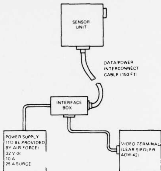
Fig. 1. Arrangement of the ADM-1 system major assemblies.
