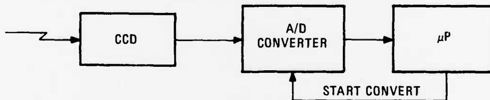
Fig. 39. Basic system configuration.
