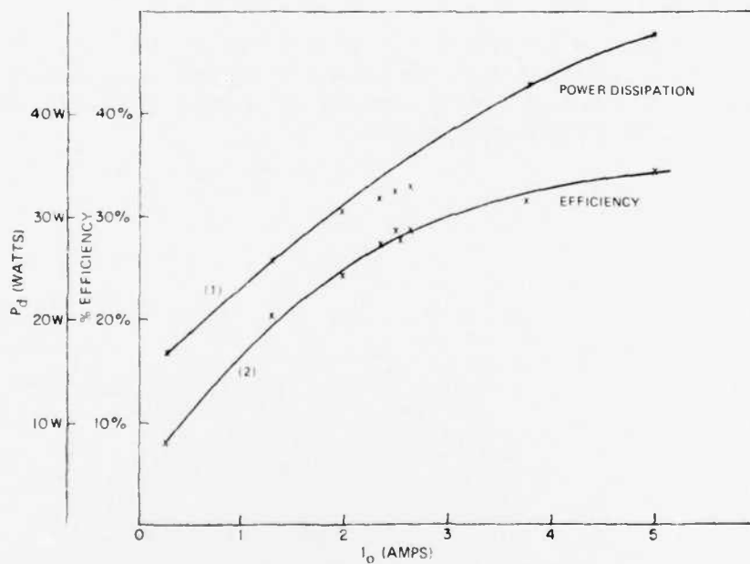
Fig. 9. Power dissipation vs. output current ( I_o ) of Abbott Transistor Labs Model SD 5.0 power supply (5-V dc, 5-A supply).
