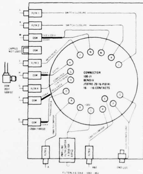
Fig. 4. Wiring arrangement of RFI/EMI enclosure.
