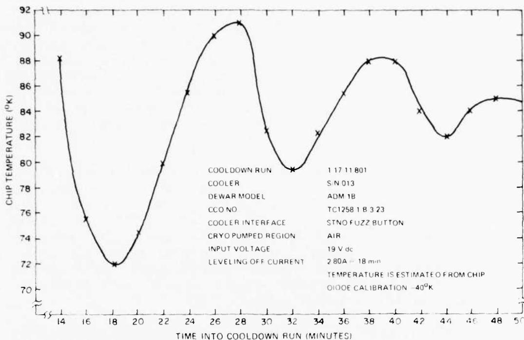
Fig. 26. Variation of chip temperature with cooldown time (run 1-17-11-801).
