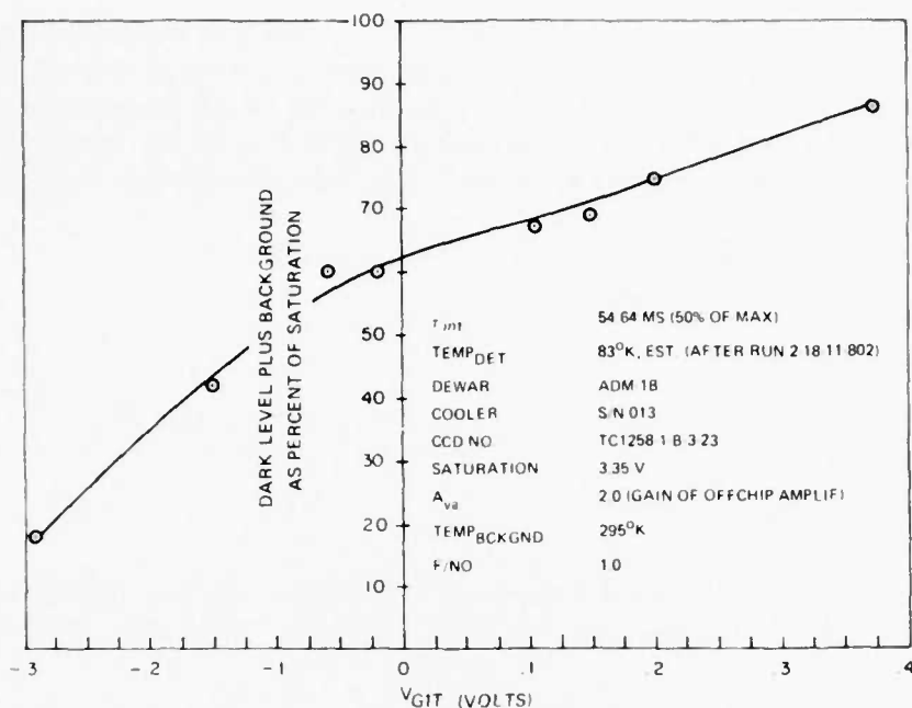
Fig. 16. Dark level plus background vs. V_{G1T} at 50% integration.
