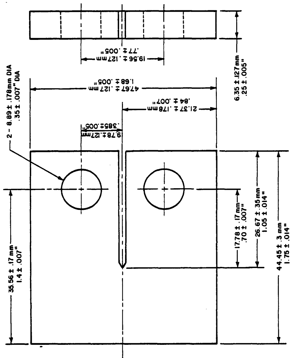
Figure 4. Dimensions of CT specimens for crack propagation tests.
