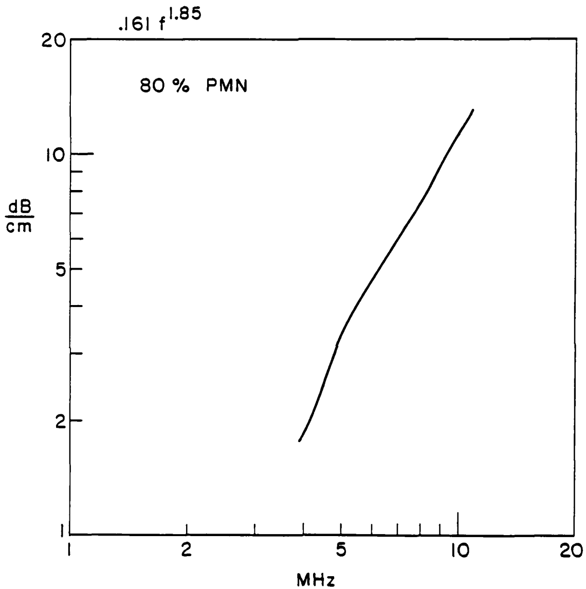
Fig. 7--Acoustic attenuation vs. frequency in Pb_3(MgNb_2)O_7 electrostrictive ceramic. The data closely fits the curve .161 f^{1.85} .
