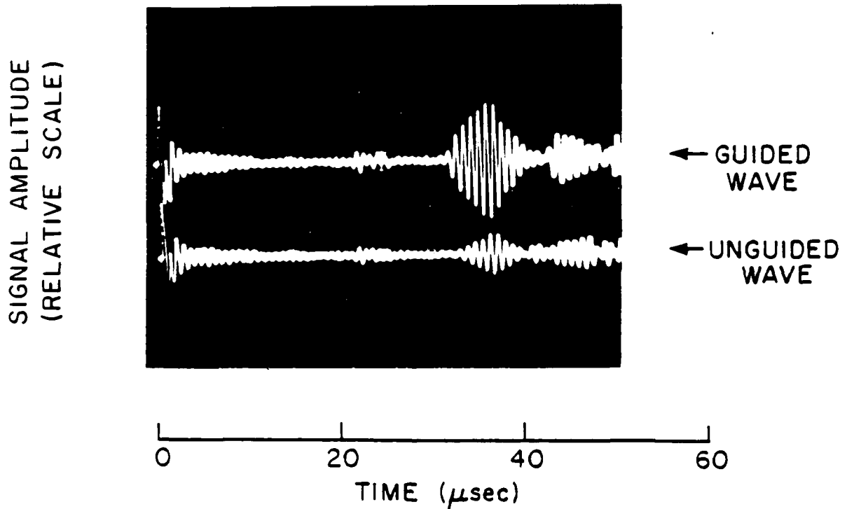
Fig. 1--Top: Improved experimental set-up for domain wall wave transmission experiments. Bottom: Pulse transmission measurements demonstrating wave guidance in this structure ( f = 1.15 MHz).
