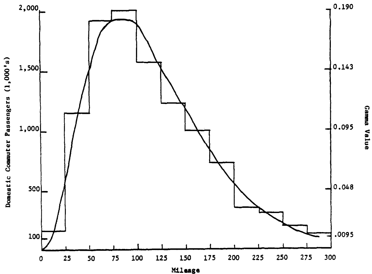
Figure 1 Distribution of commuter passengers by mileage, 1979, and gamma distribution approximation.
