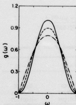
FIG. 1. Beta spectrum with \nu = 3 and estimates: — exact spectrum; --- N = 10 ; ... N = 20 .
