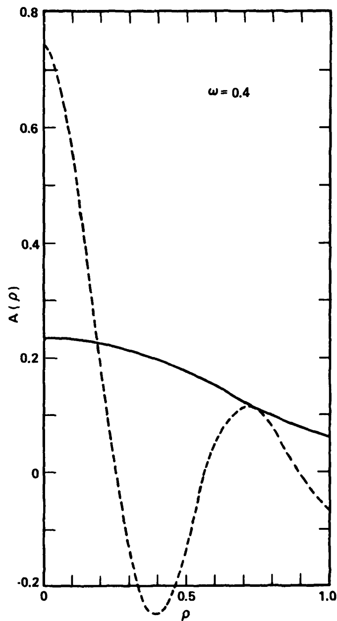
Fig. 2. Pupil functions that achieve the upper bound (—) and lower bound (---) at \omega = .4 .
