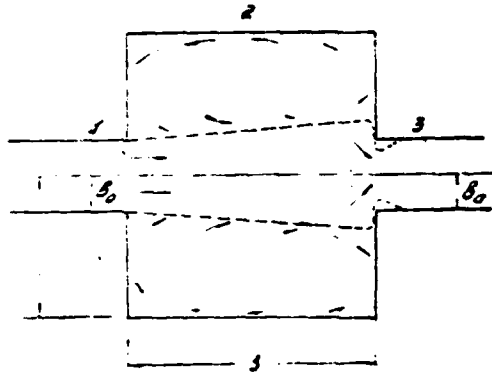
Fig. 4.2. The aerodynamic configuration of flow in the cell of labyrinth.
