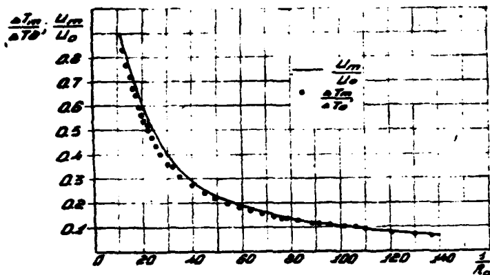
Fig. 30. Comparison of the loss of a change in the velocity and excess temperature along the axis of circular jet according to experiments of Syrkin.
