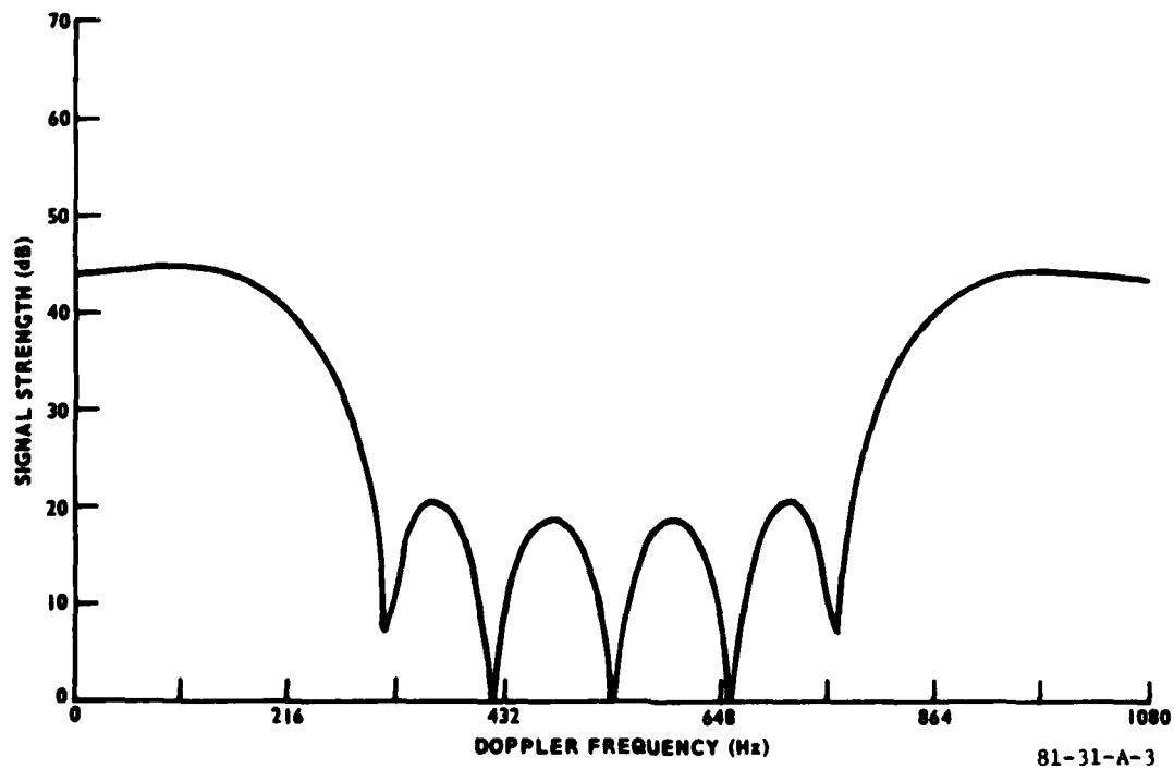
FIGURE A-3. MTD II COMPUTED DOPPLER FILTER RESPONSE (ZERO FILTER)
