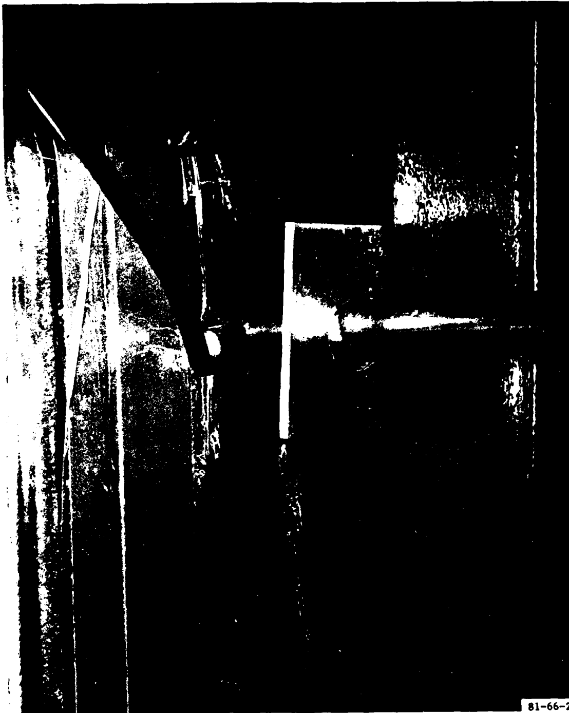
FIGURE 2. CLOSEUP OF IMPACT AREA SHOWING HOLE IN KIMCODE™ SAFETY RIMBAND, COOLANT TUBE, AND CENTER PUNCH
