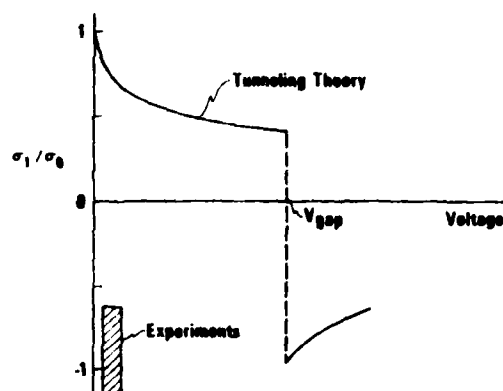
FIG. 2. Schematic diagram illustrating the dependence of \sigma_1/\sigma_0 upon voltage (solid curve), according to tunneling theory. The shaded rectangle indicates the locations of experimental determinations of \sigma_1/\sigma_0 for tunnel, microbridge, and point contact junctions. A recent experiment (Ref. 15) carried out on tunnel junctions at several temperatures near the critical temperature, showing both signs for \sigma_1/\sigma_0 , but opposite to that expected from tunneling theory, is not shown.
