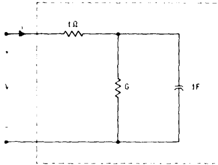
Fig. 5. The value of the shunt resistor is R = (1/G) \Omega . The 1-port is of course strongly passive provided G > 0 .
