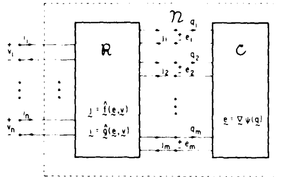
Fig. 7. Every voltage-controlled state representation has a realization of this form in which \mathcal{C} is passive. If \mathcal{R} and \mathcal{C} are both passive it is called a passive realization.
