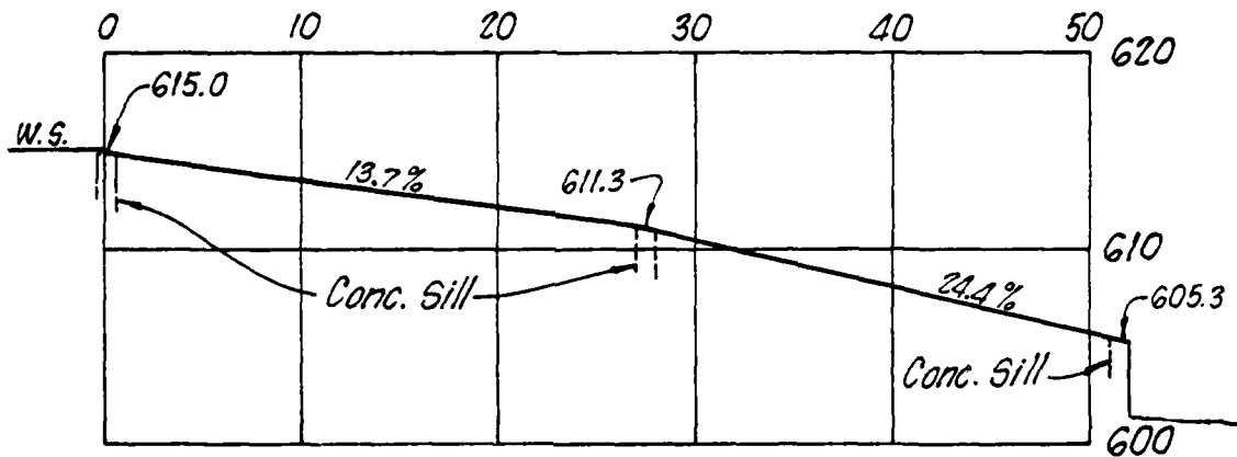
SPILLWAY PROFILE
