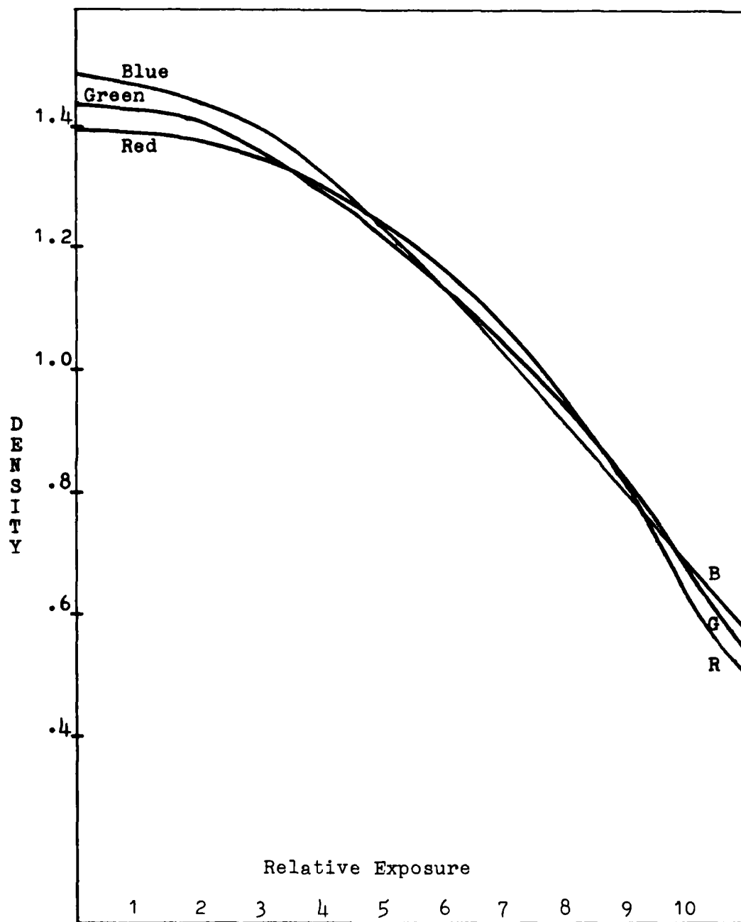
Fig. 5-1. Neutral Characteristic Curves
