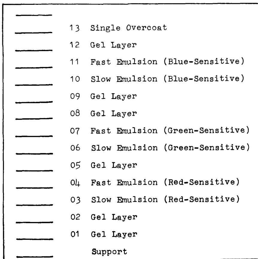
Fig. 2-2. Kodak Ektachrome 160 Film Structure 4
