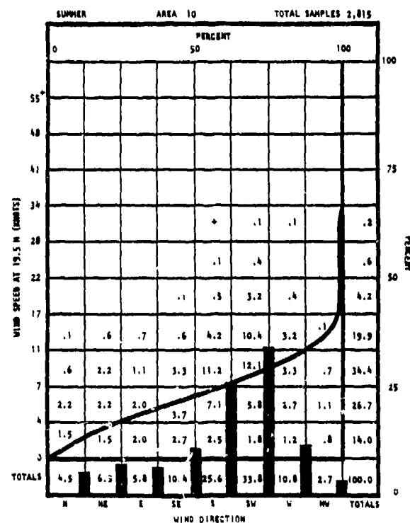
Figure A-10-4-4 Wind Speed by Wind Direction
