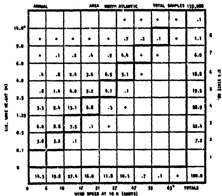
Figure A-6 Significant Wave Height by Wind Speed (WMO Sea State Chart)
