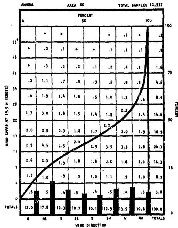
Figure A-00-1-4 Wind Speed by Wind Direction
