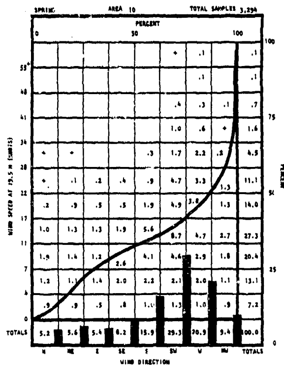
Figure A-10-3-4 Wind Speed by Wind Direction
