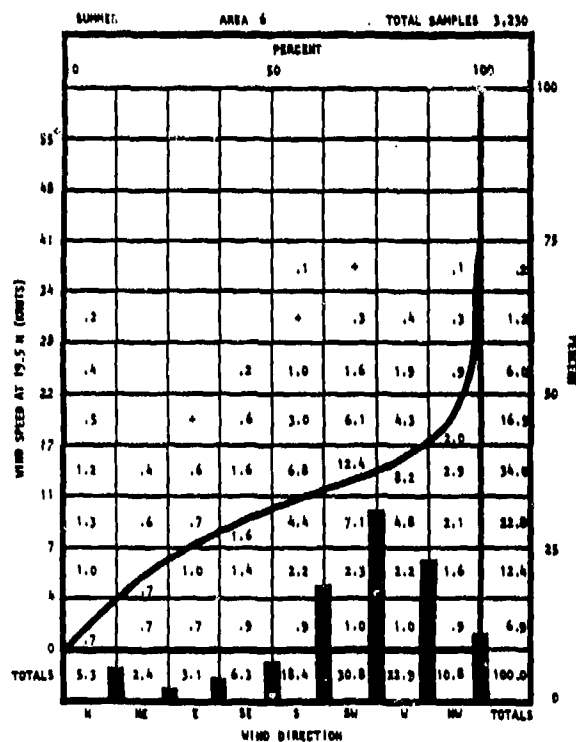
Figure A-6-4-4 Wind Speed by Wind Direction
