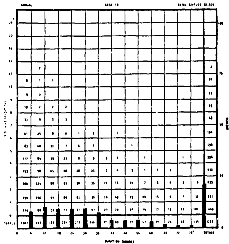
Figure A-10-1-6 Persistence of Significant Wave Height
