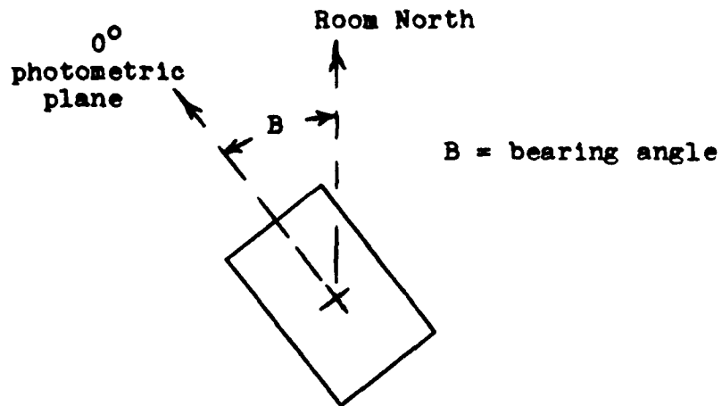
Figure 28: Definition of luminaire bearing angle. View is from above luminaire.
