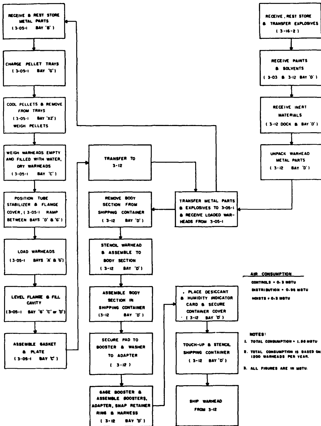
Figure 8. Yearly air consumption--GM, HE warhead M17A1
