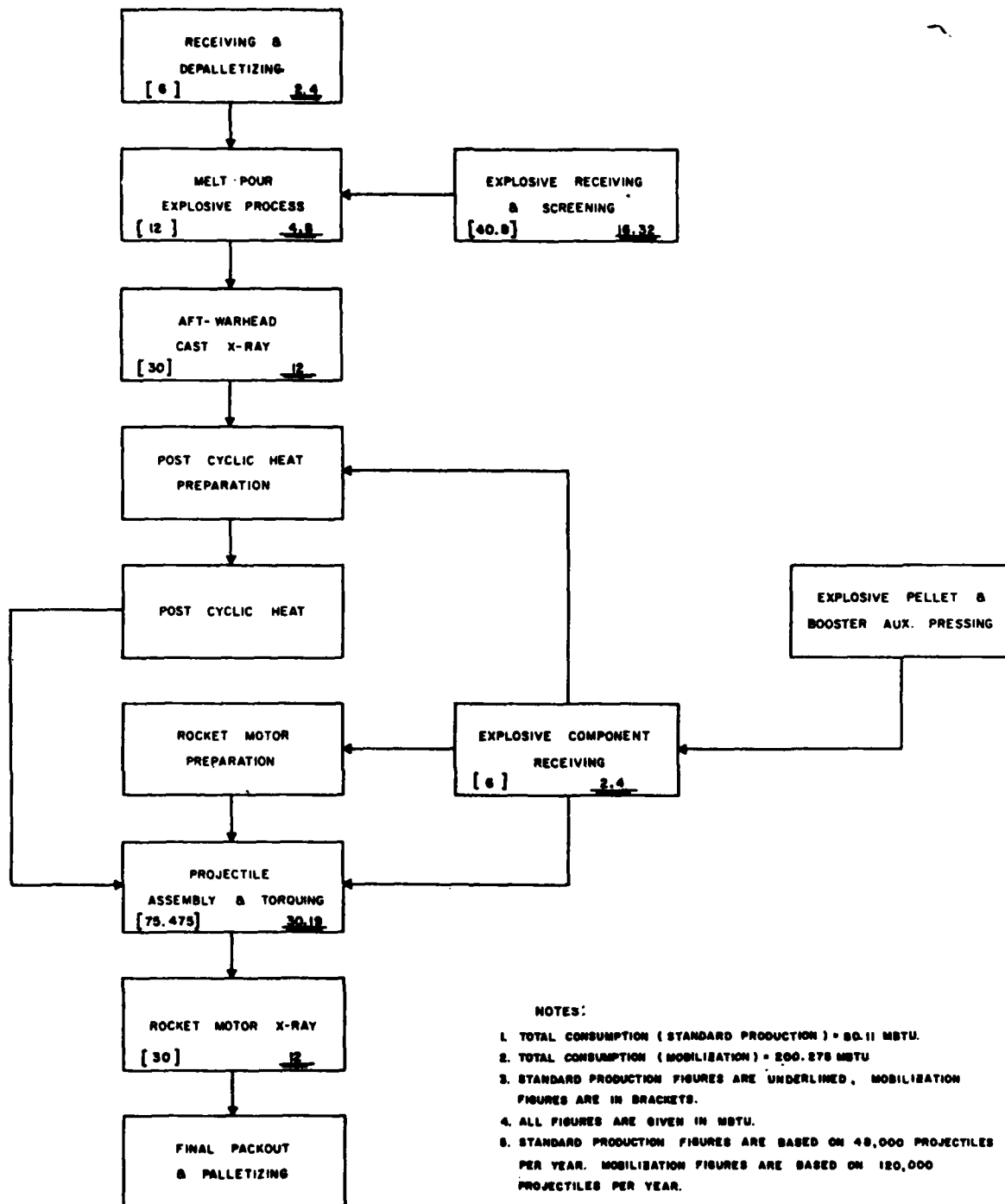
Figure 12. Yearly air consumption--8-inch HE projectile M650E5
