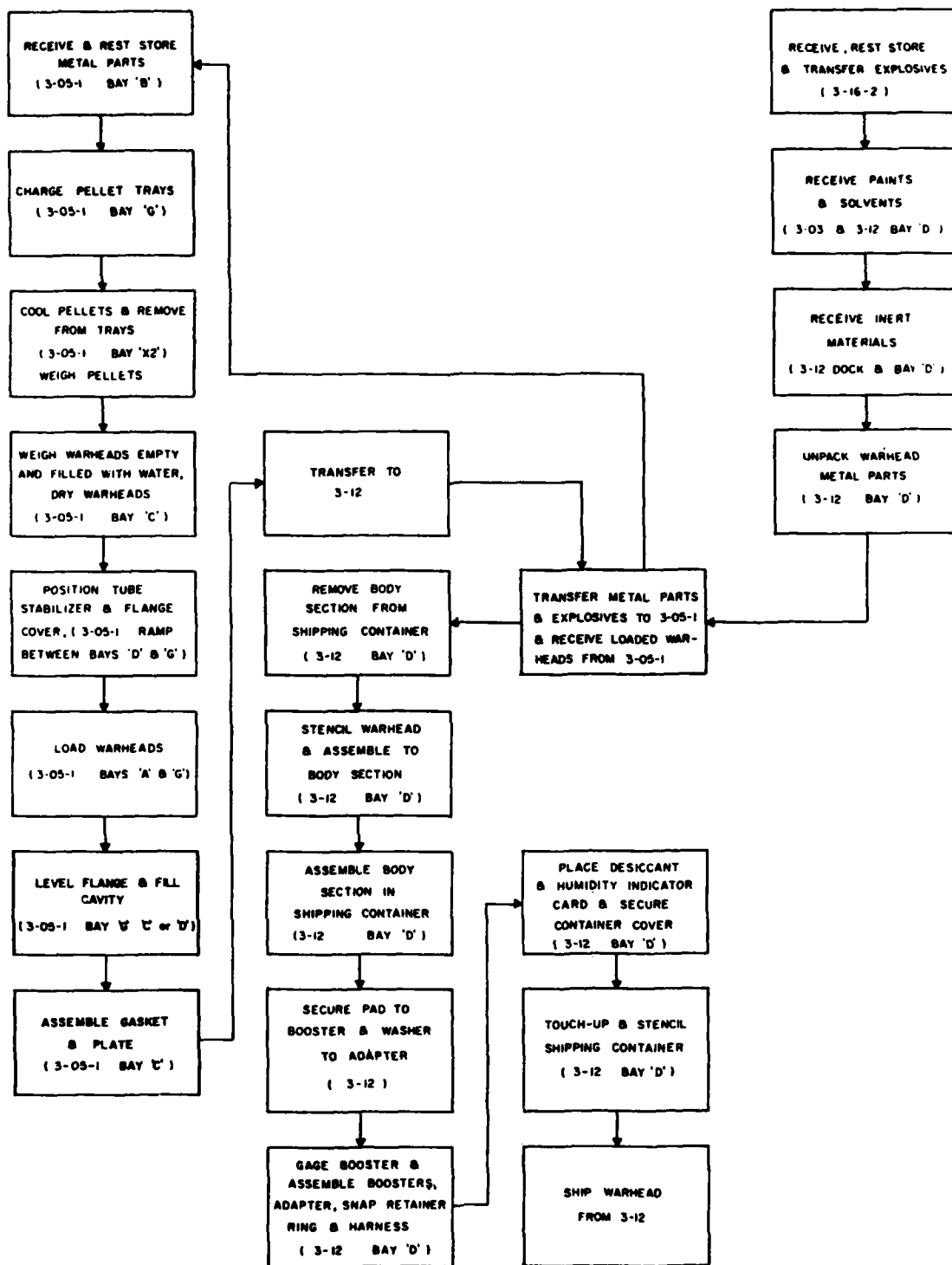
Figure 5. Process description--GM, HE warhead M17A1
