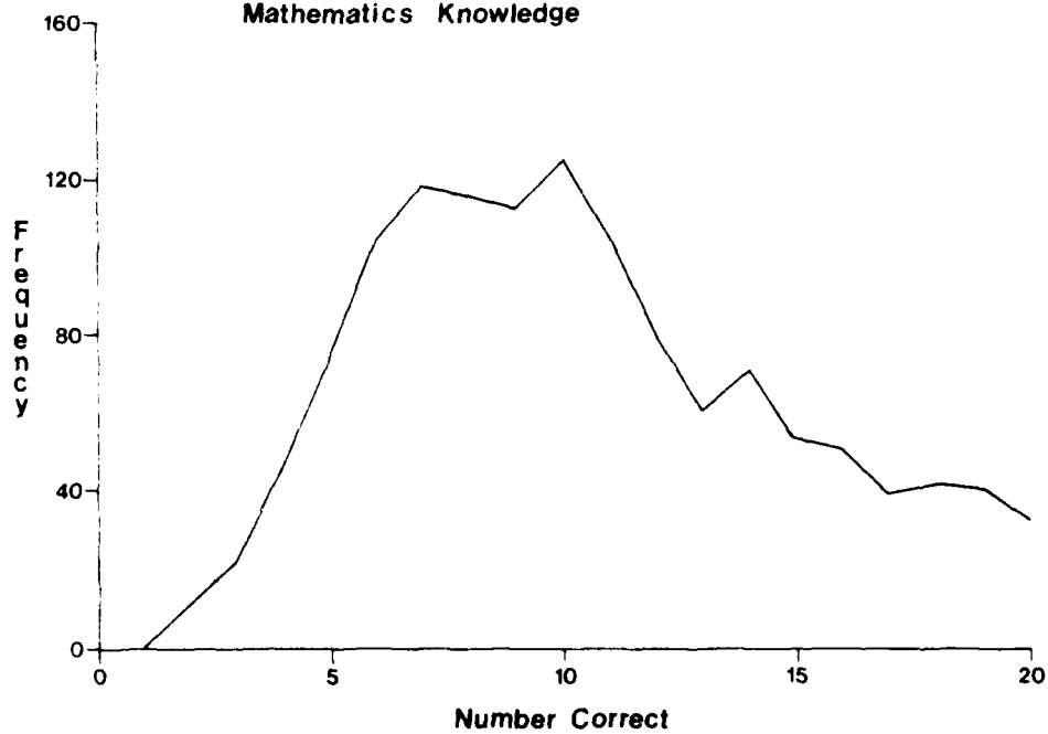
Figure 5. Raw Score Frequency Distribution Mathematics Knowledge
