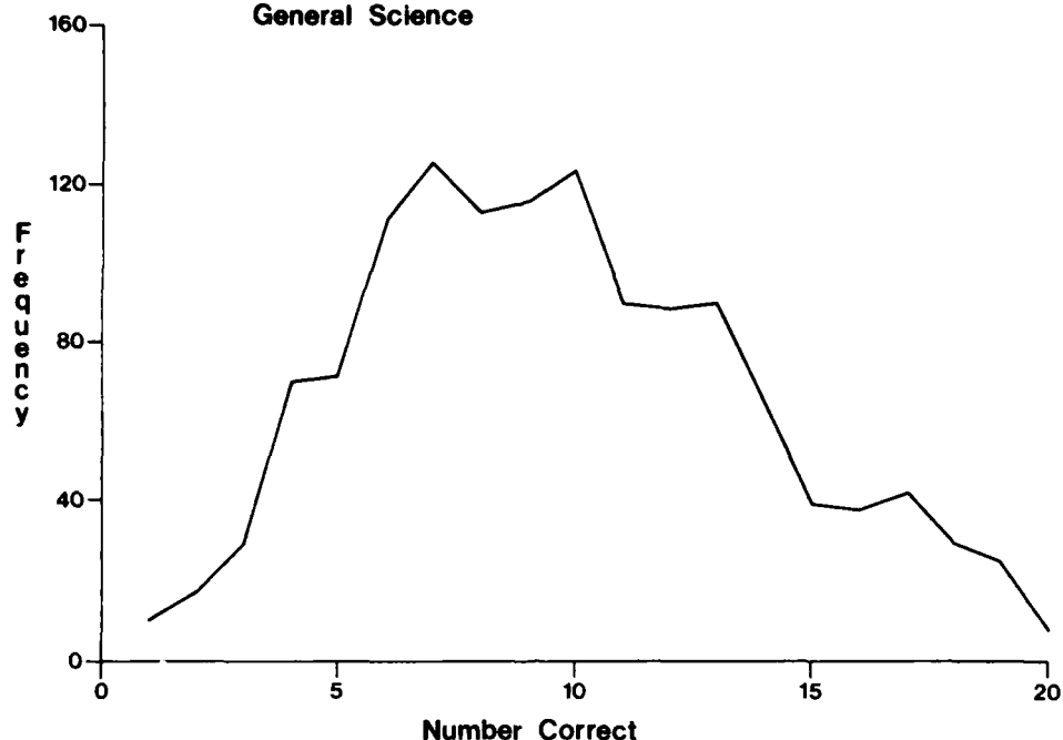
Figure 8. Raw Score Frequency Distribution General Science
