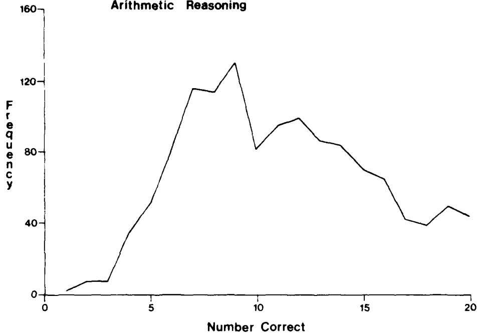
Figure 4. Raw Score Frequency Distribution Arithmetic Reasoning
