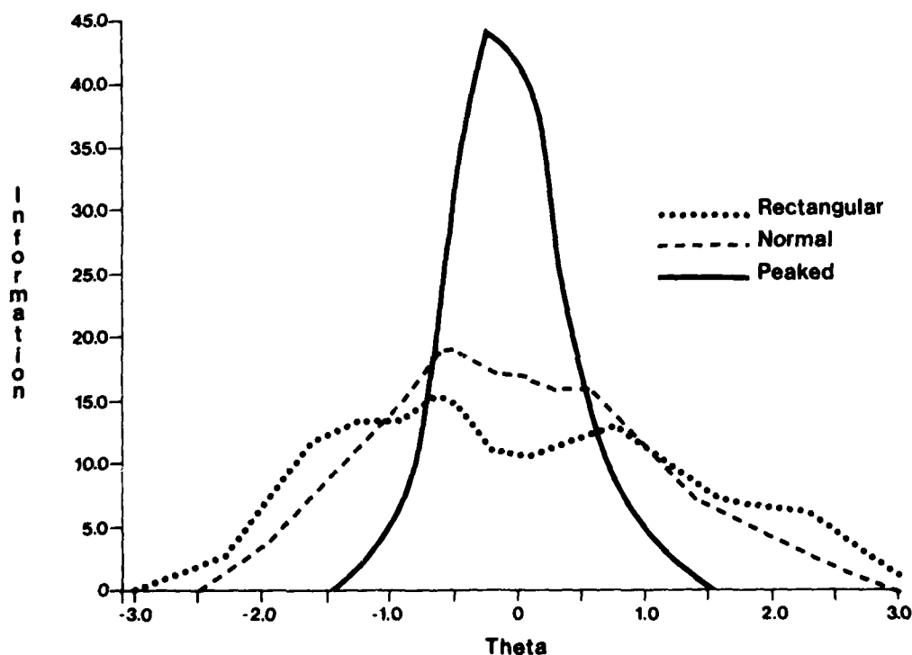
Figure 9. True Information Curves, Using True Item Parameters, for Each of Three Anchor Tests
