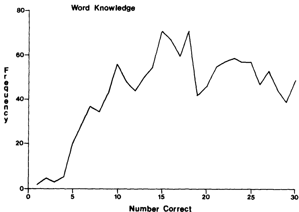
Figure 3. Raw Score Frequency Distribution
