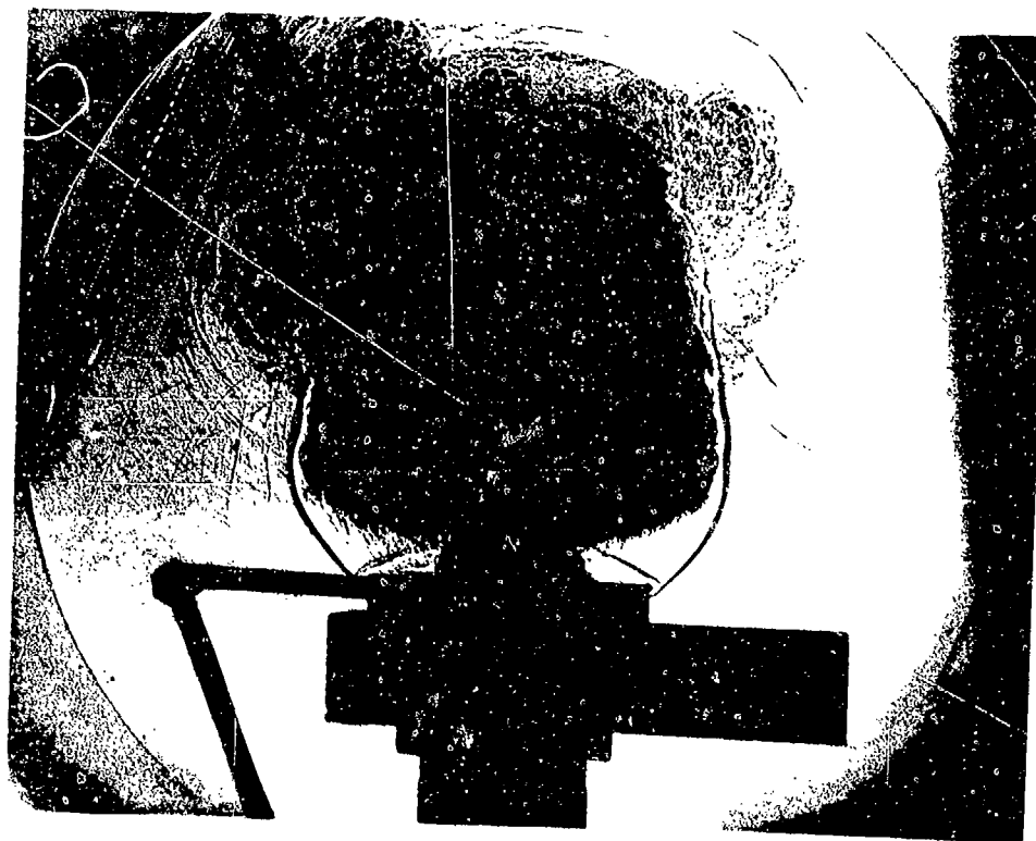
b. Ambient Gun Tube Figure 15. Spark Shadowgraphs Comparing Ambient and Evacuated Gun Tube Precursor/Propellant Gas Interactions, V_p = 1050 \text{ m/s}
