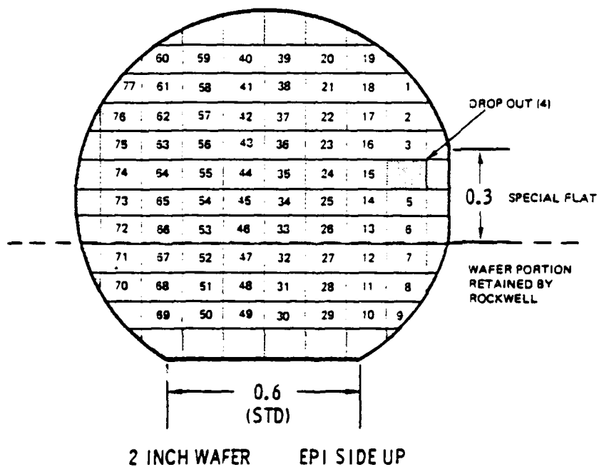
Figure 12. Die Identification
