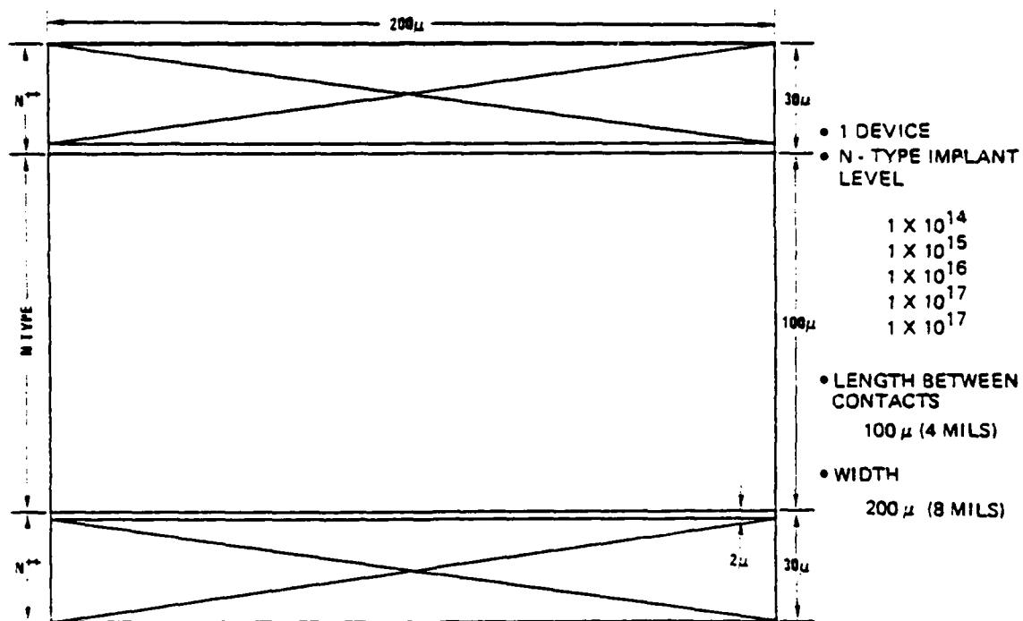
Figure 2. Doping Level Test Structure
