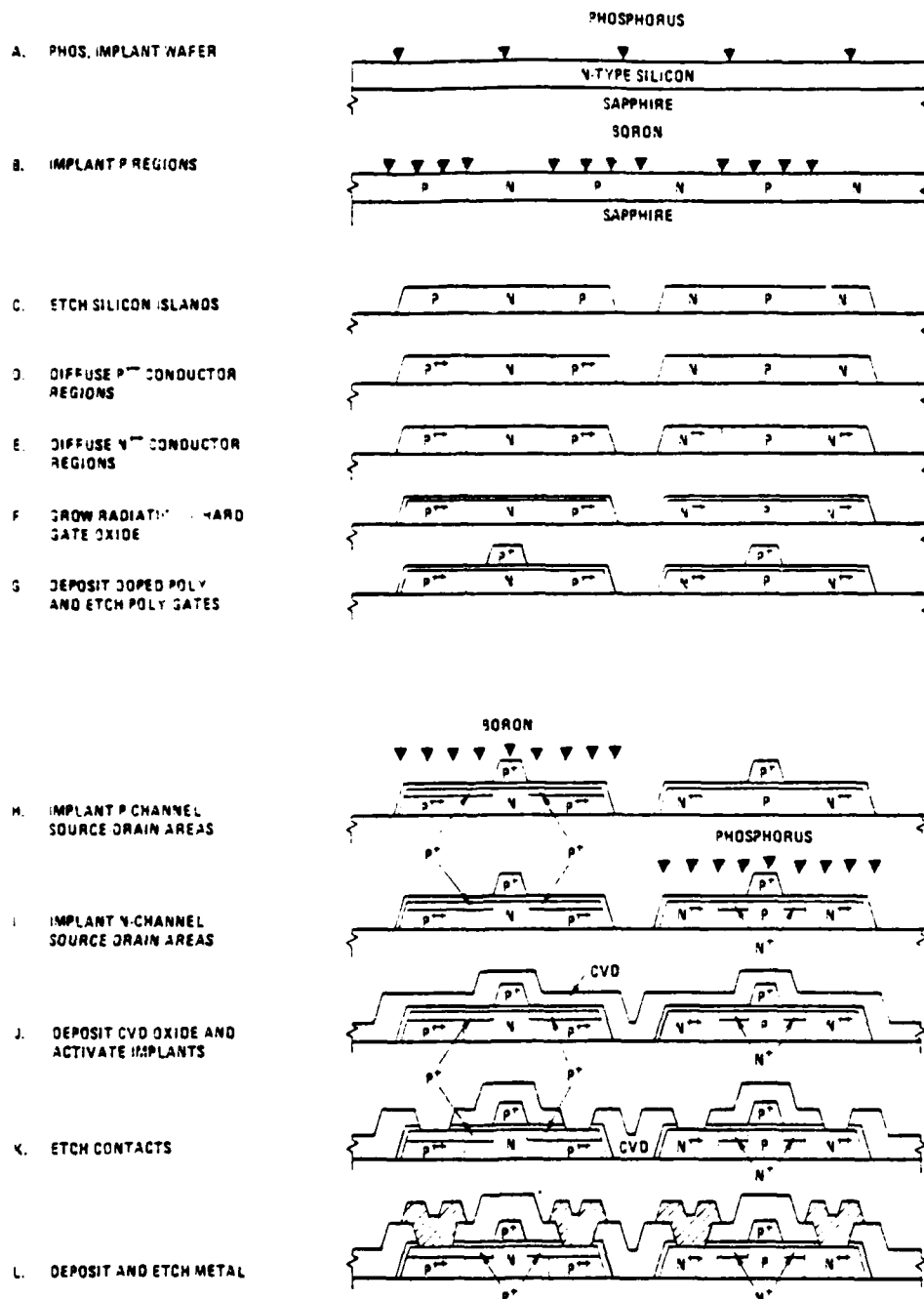
Figure 13. Si-Gate CMOS/SOS Process
