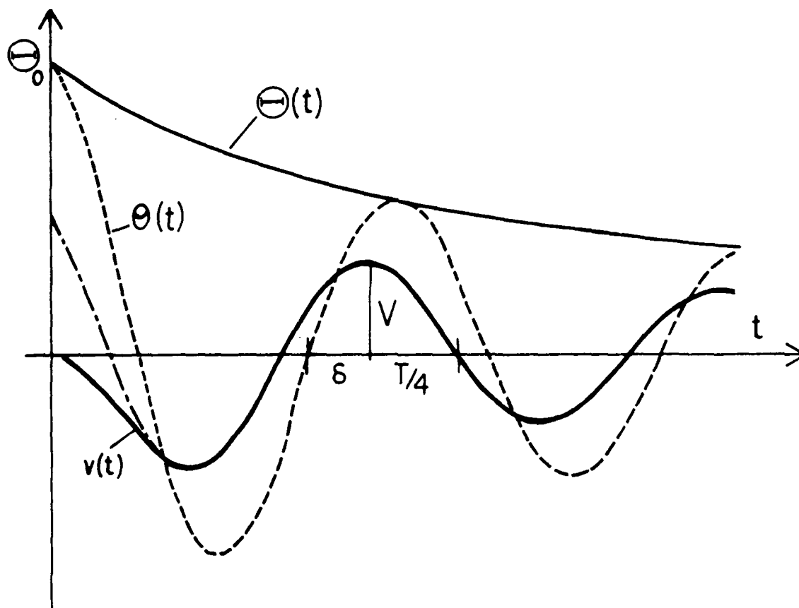
Figure 2: Idealised time series \theta(t) , \ominus(t) and v(t) . The real velocity is u(t) = L \frac{d\theta}{dt} \approx L\omega\ominus \sin \omega t .
