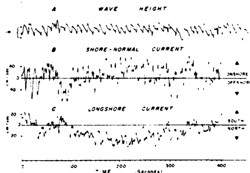
Figure 4 Sample time series of surf-zone pressure sensor and current meters
