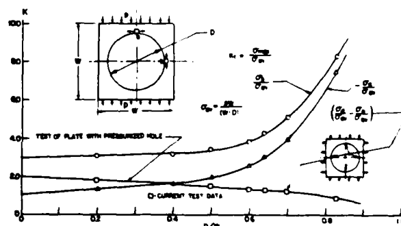
Fig. 5 Stress-concentration factors for a round hole in a square plate subjected to a uniaxial uniform pressure and computations for the biaxial case
