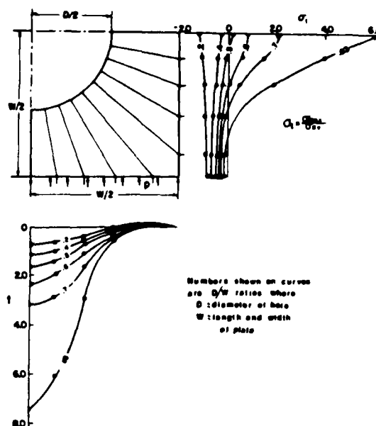
Fig. 4 Stress distributions on outer boundary of a square plate with a round hole subjected to uniform pressure applied to two opposite sides of the plate (average stress on the net section used for comparison)
