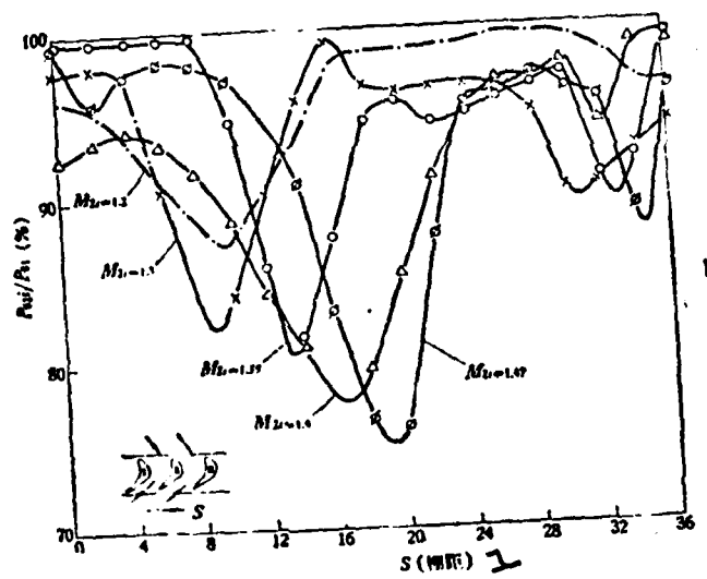
Figure 5. Experimental Curves for Transonic Turbine Blade Cascade Performance.
