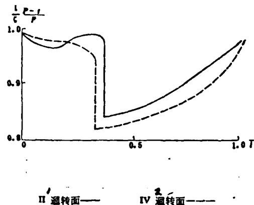
Figure 7. The distribution of the surface of revolution \frac{1}{5} \frac{P-t}{P} along the center line of the passageway involved.
