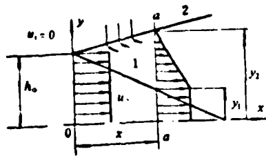
Figure 1. A simplified diagram of a free planer jet flow
