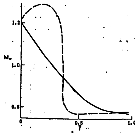
S_{2c} - - - - Normal Calculation of the S_2 Flow ———
