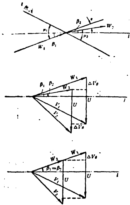
Figure 1. The oblique shock wave \beta_2 = \beta_1 - \epsilon and the velocity triangle for the gas flow both in front of and behind the wave Key: 1--shock wave
