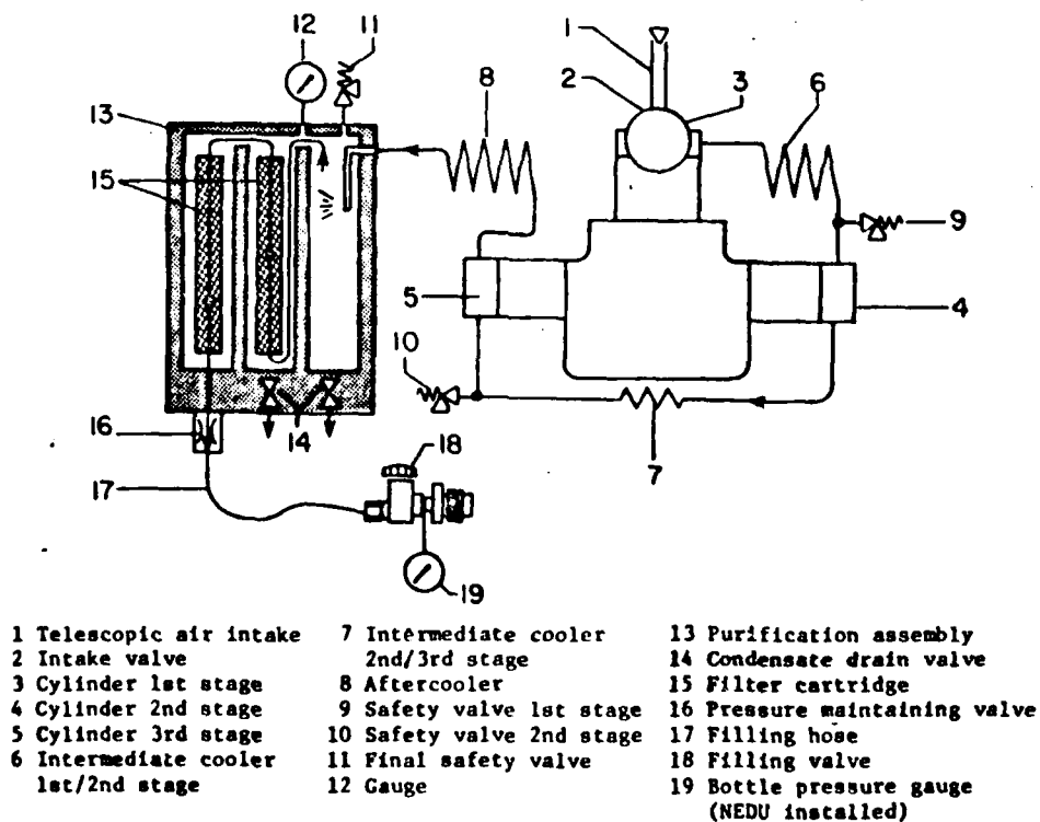
Figure 3. Compressor Schematic
