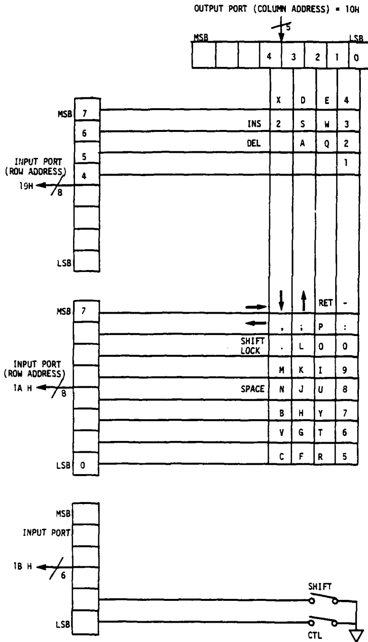
FIGURE 3-2. KEYBOARD MATRIX/MICROPROCESSOR INTERFACE CONFIGURATION
