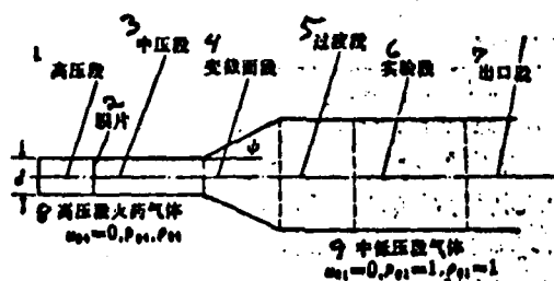
Figure 1. Diagram of the shock tube Key: 1--high pressure section; 2--film; 3--medium pressure section; 4--section with variable cross-sectional area; 5--transitional section; 6--experimental section; 7--exit section; 8--explosive gas in high pressure section; 9--gas in medium and low pressure sections
