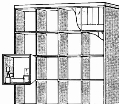
c. Box-Wall Principle
