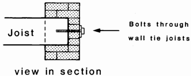
Joists inserted into walls to support floors
