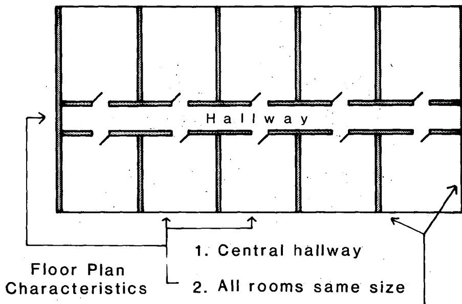
Floor Plan View (above ground floor)
