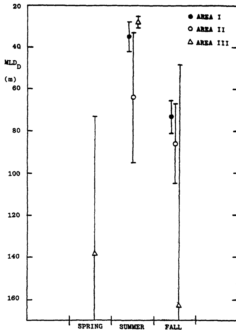
Figure 4.3 Dependence of MLD on area and season for density criterion. Mean MLD D and 95% confidence interval.
