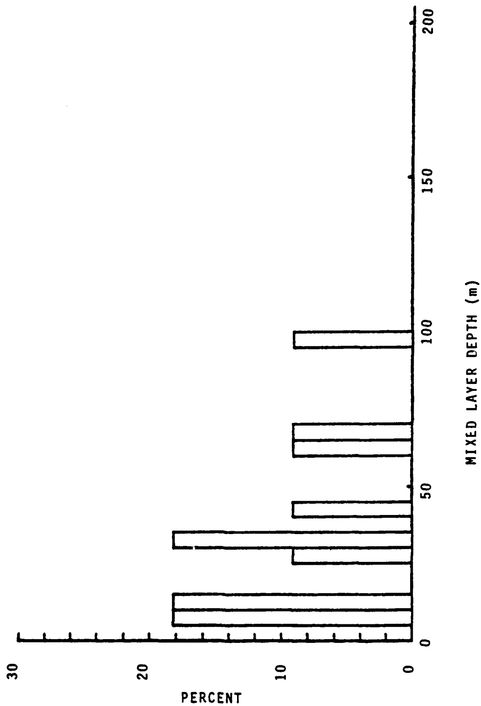
Figure 3.40 Histogram of MLD N for Fall, Area III (11 Stations)
