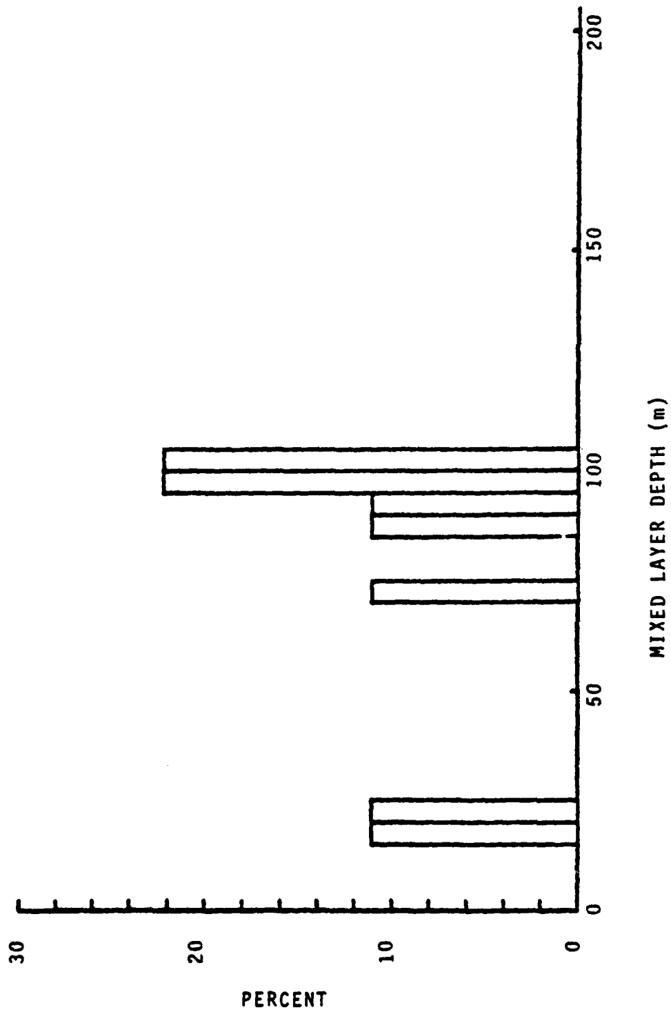
Figure 3.6 Histogram of MLD T for Fall, Area II (9 Stations)
