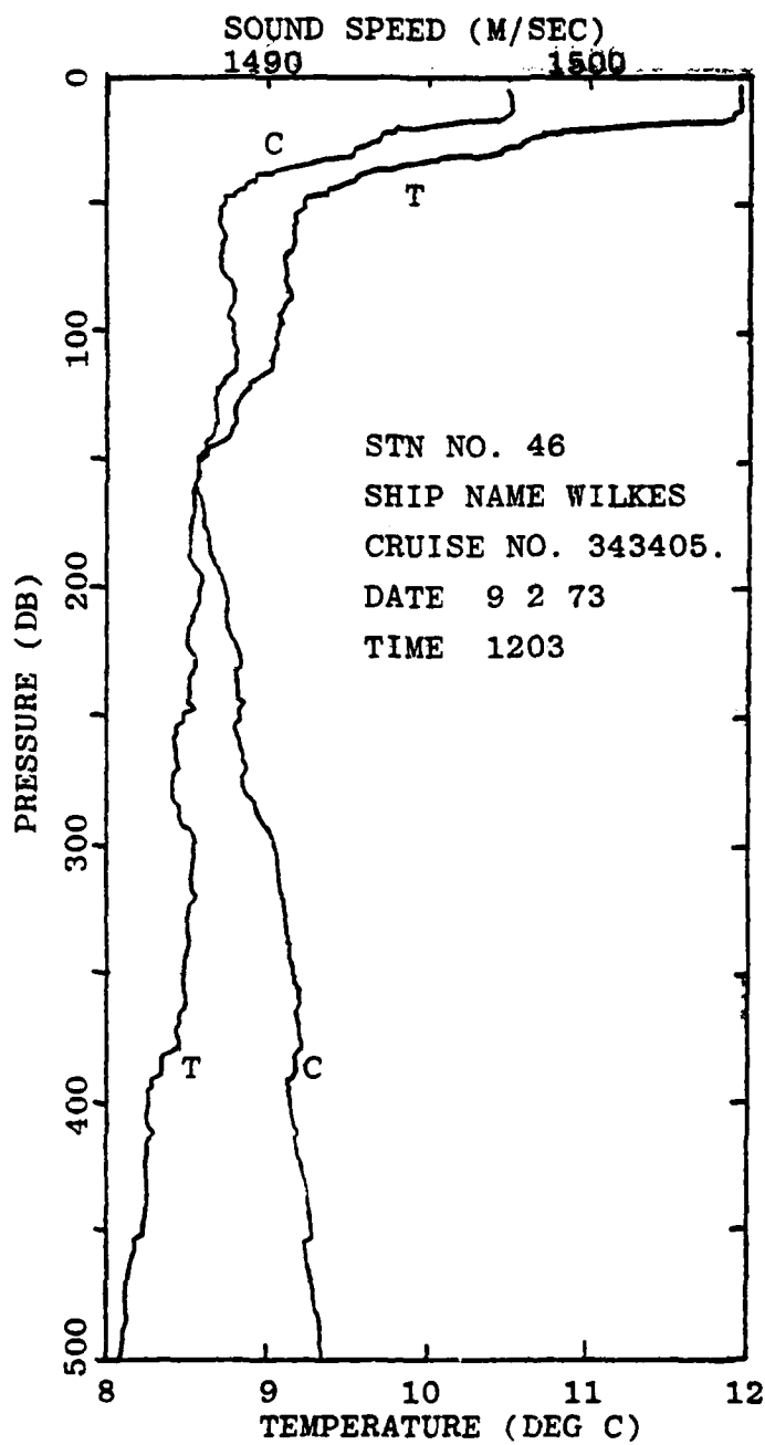
Figure 2.2 Sound speed (C) and temperature (T) profiles at a sample SVSTD station before smoothing.
