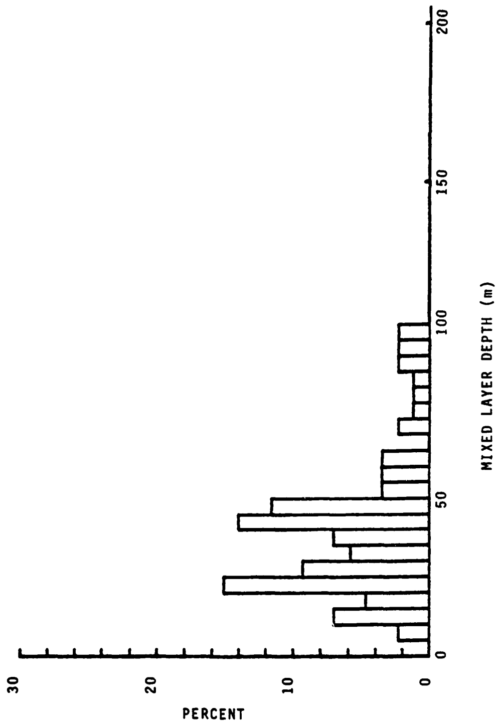
Figure 3.10 Histogram of MLD T for All Seasons, Area II (86 Stations)
