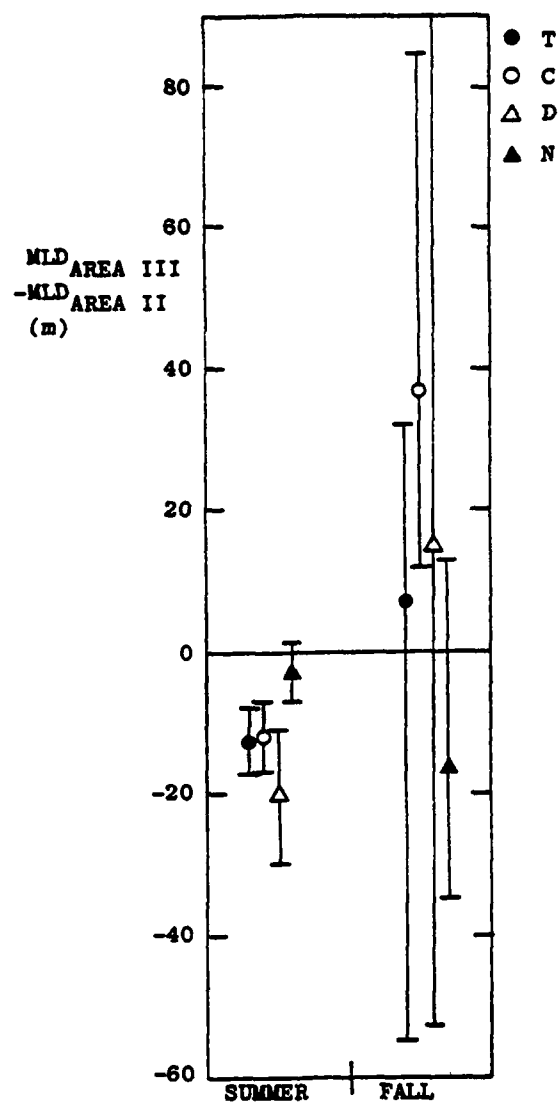
Figure 4.10 c) Area III - Area II.
