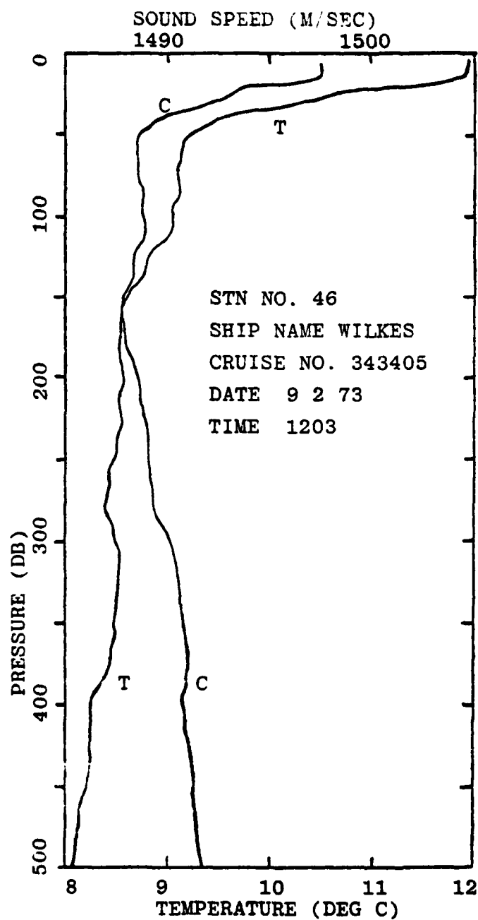
Figure 2.4 Sound speed (C) and temperature (T) profiles at a sample SVSTD station after smoothing.
