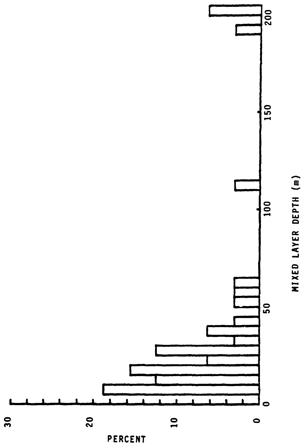
Figure 3.30 Histogram of MLD D for Spring, Area III (32 Stations)
