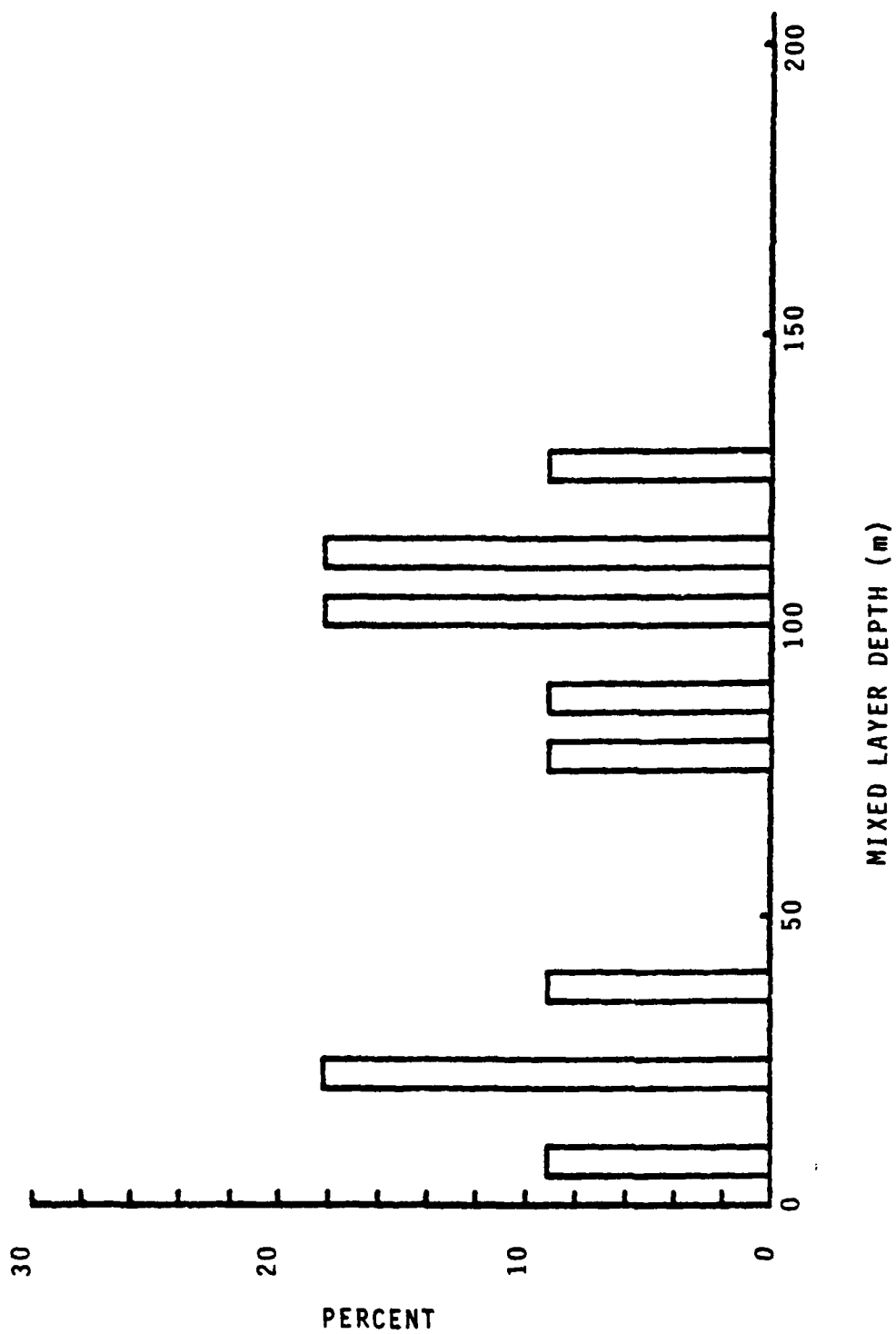
Figure 3.7 Histogram of MLD T for Fall, Area III (11 Stations)
