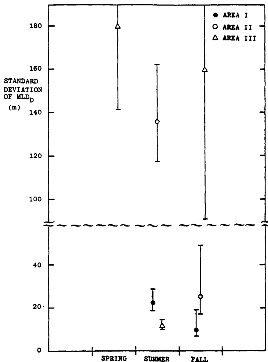
Figure 4.7 Dependence of MLD standard deviation and 95% confidence interval on area and season for the density criterion. Note break in vertical axis.
