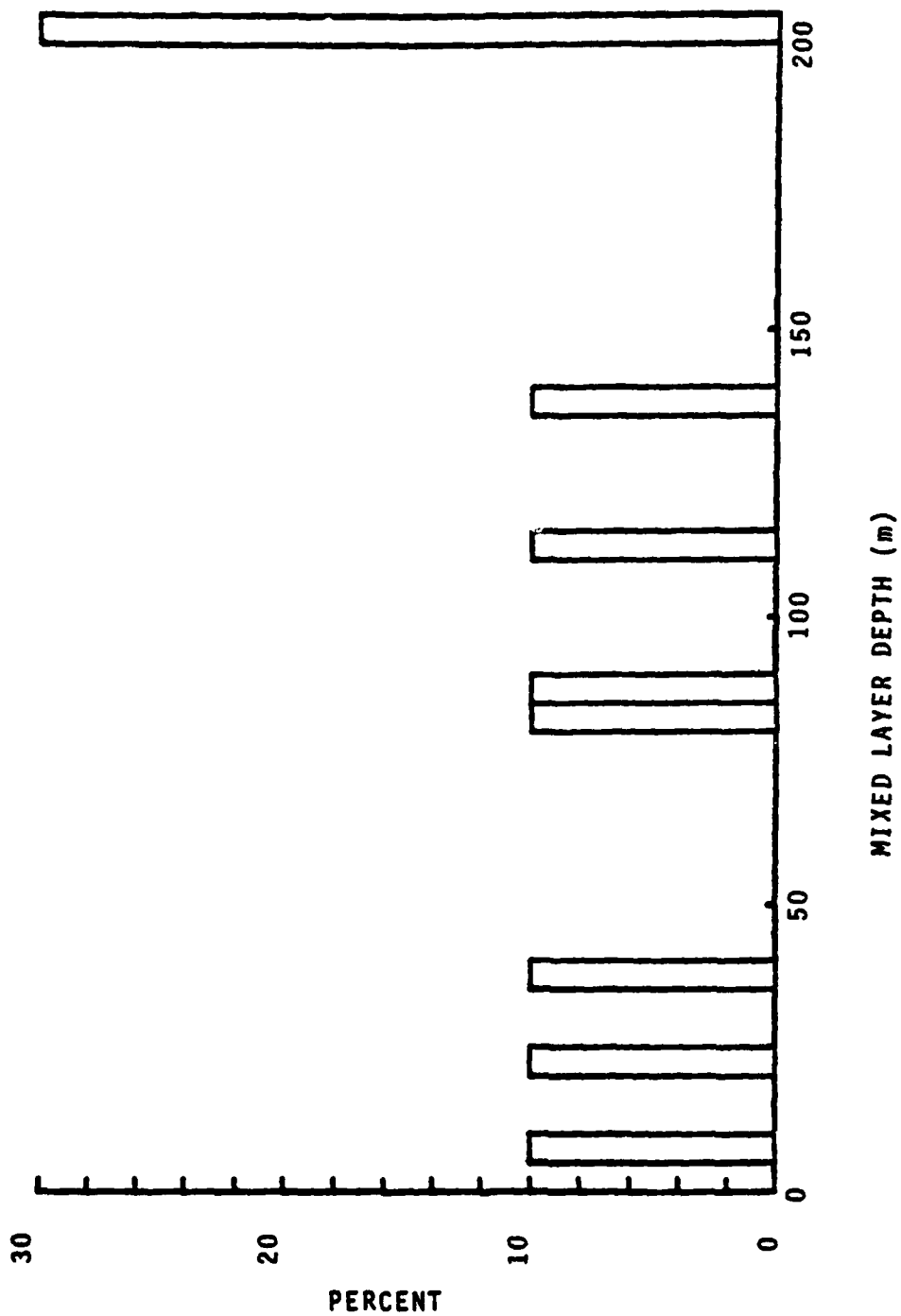
Figure 3.18 Histogram of MLD c for Fall, Area III (10 Stations)
