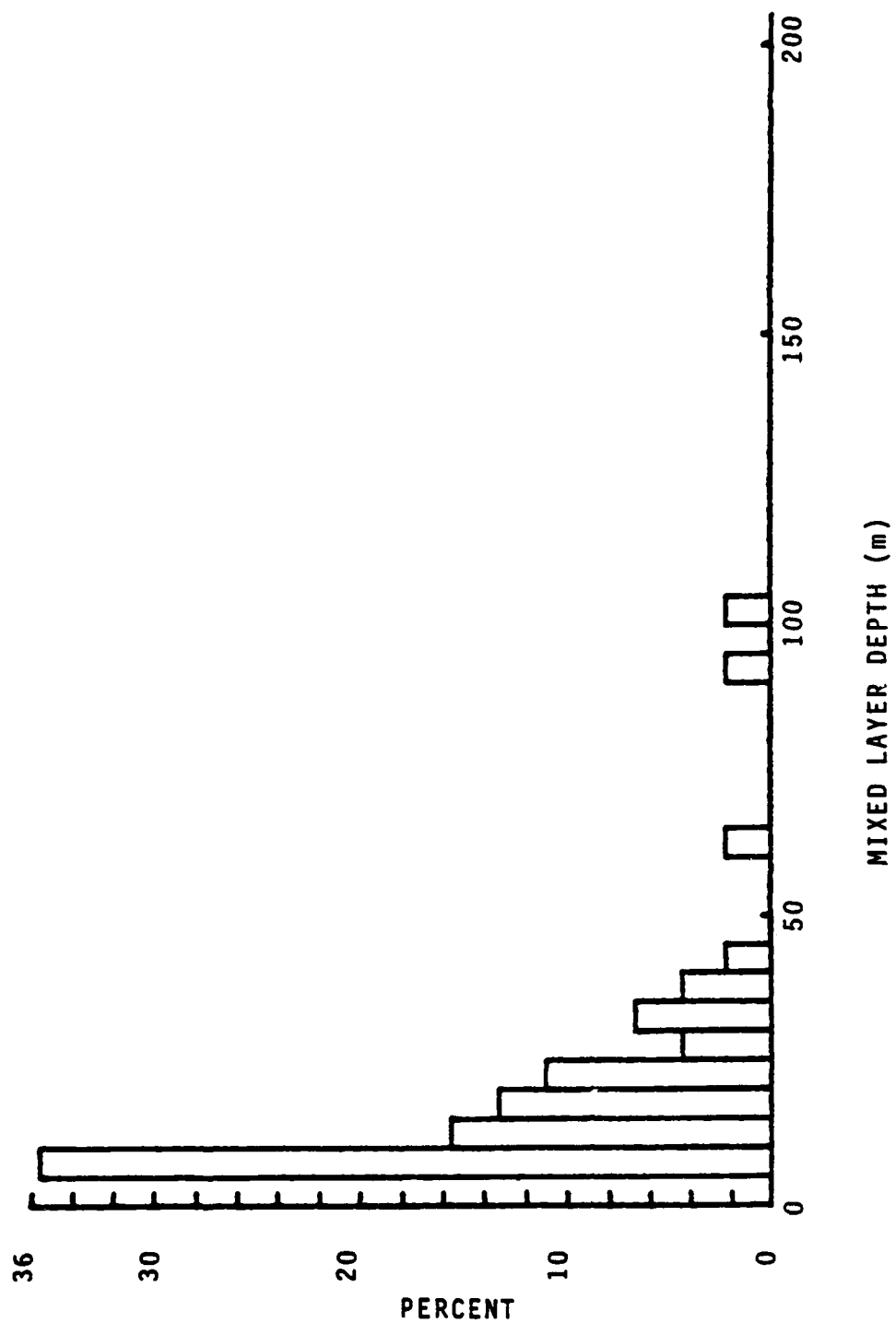
Figure 3.24 Histogram of MLD 9 for Summer, Area I (45 Stations)
