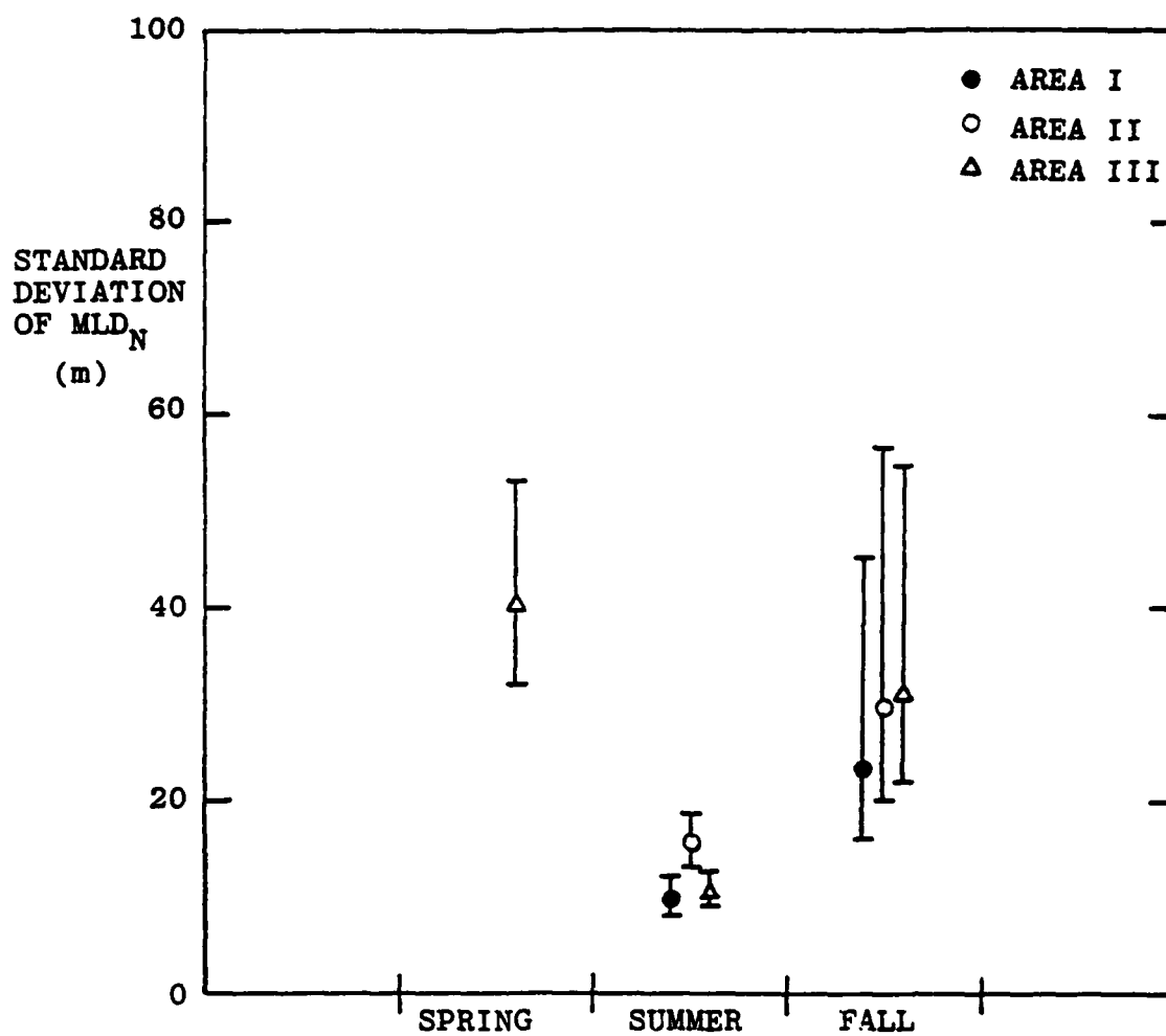
Figure 4.8 Dependence of MLD standard deviation on area and season for the stability criterion. MLD standard deviation and 95% confidence interval on the standard deviation.
