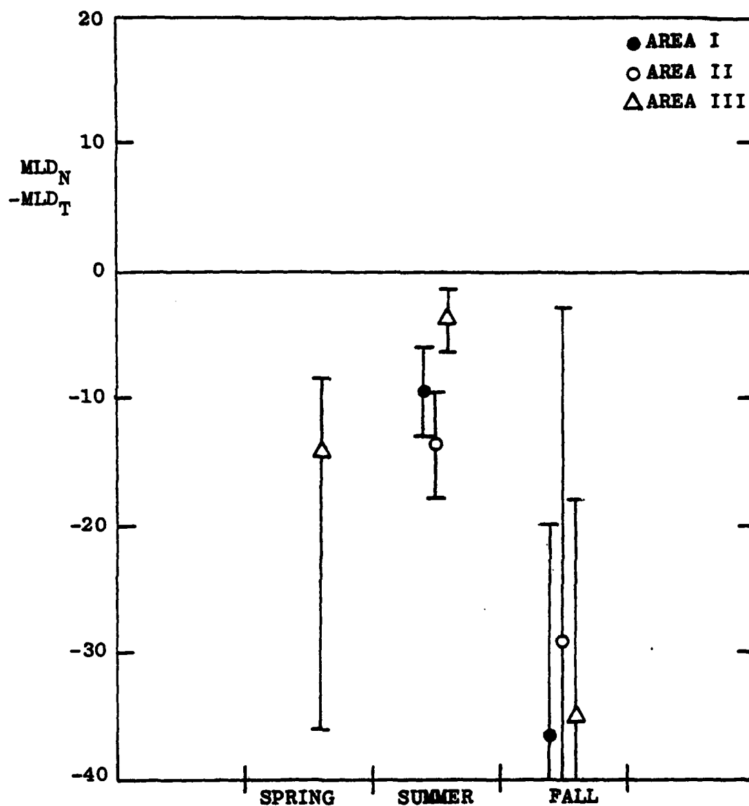
Figure 4.11 c) Difference between stability and temperature criteria as a function of area and season. Mean MLD difference and 95% confidence interval.
