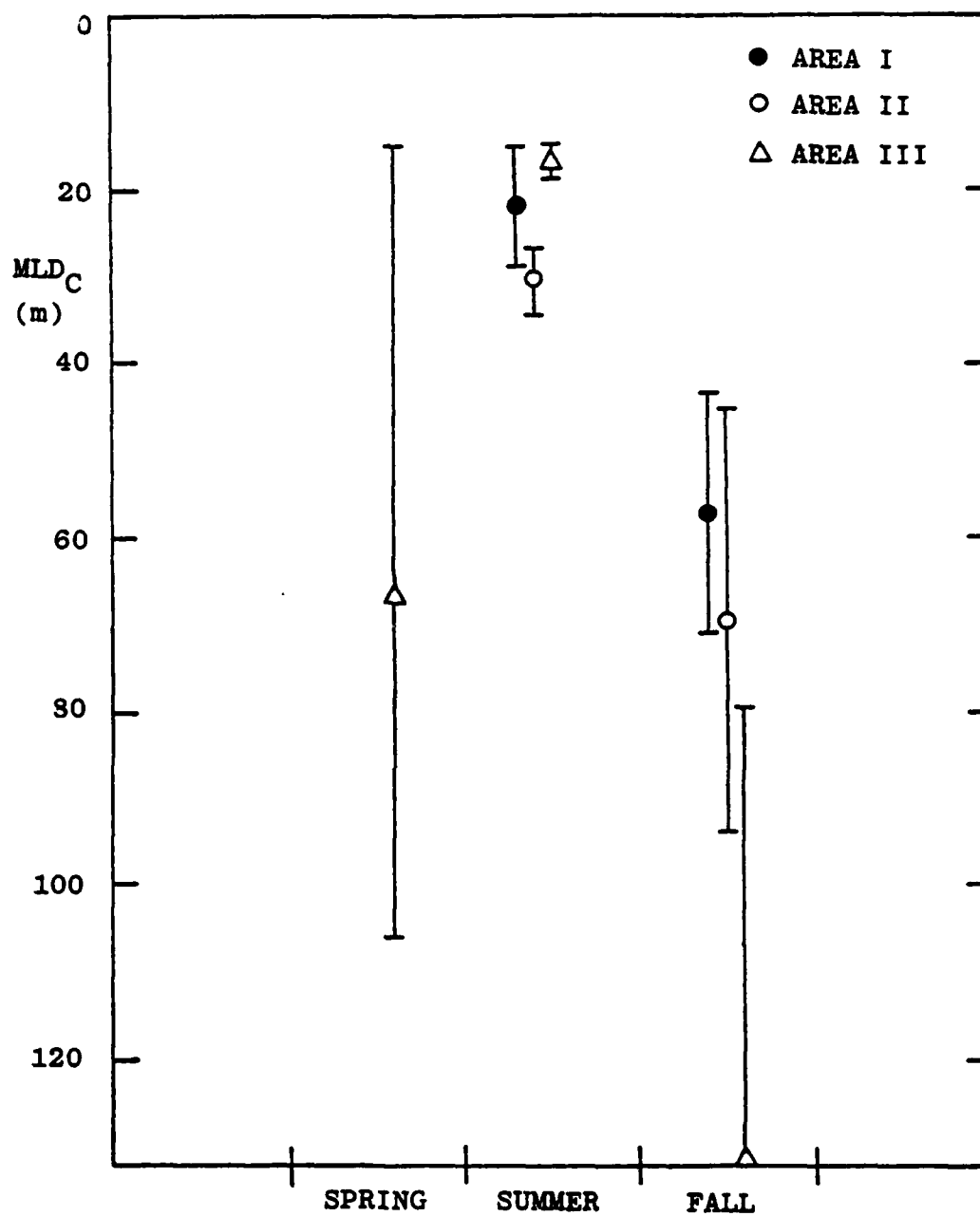
Figure 4.2 Dependence of MLD on area and season for sound speed criterion. Mean MLD C and 95% confidence interval about mean.
