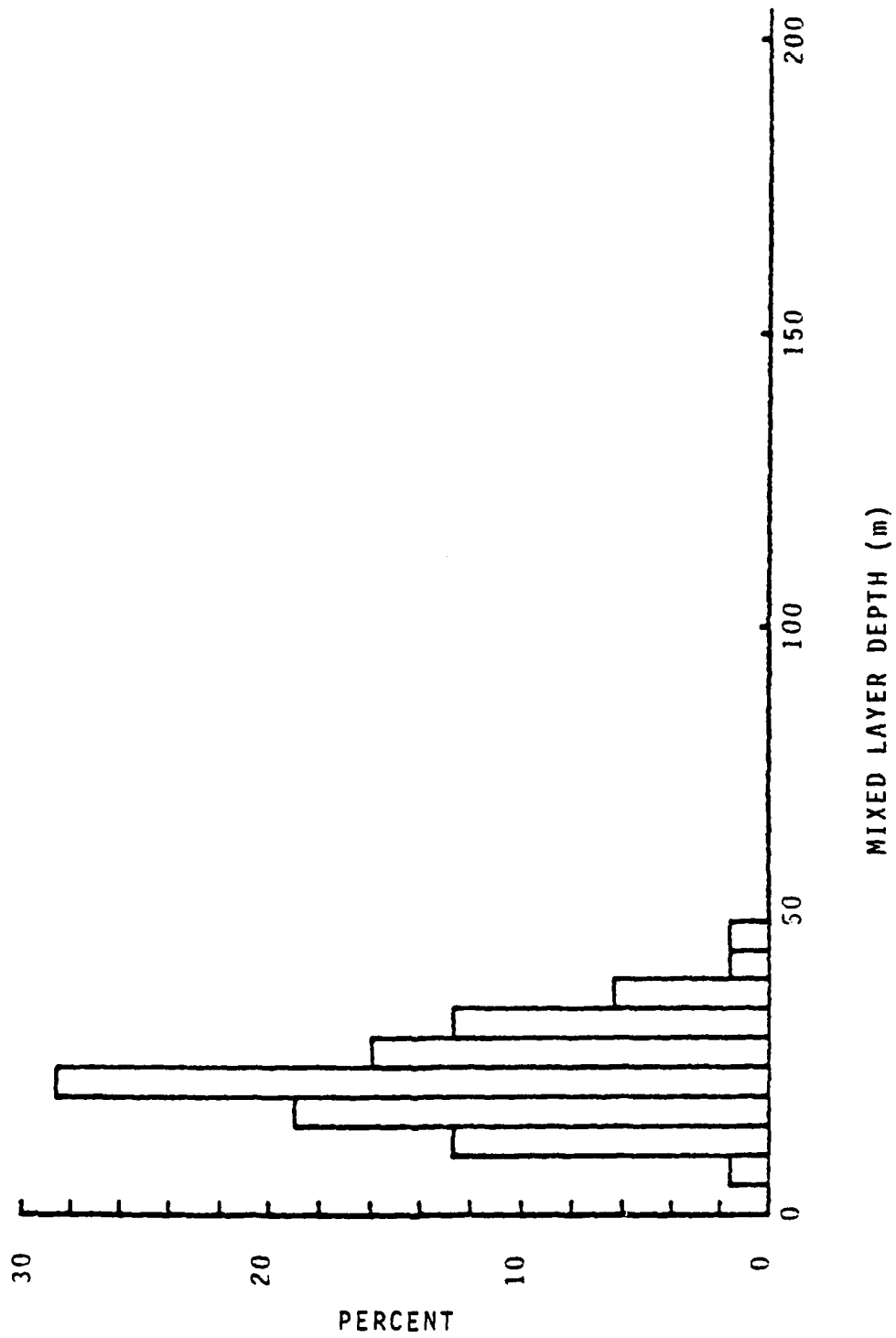
Figure 3.4 Histogram of MLD T for Summer, Area III (63 Stations)
