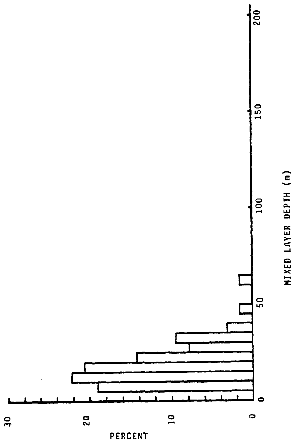
Figure 3.37 Histogram of MLD N for Summer, Area III (63 Stations)
