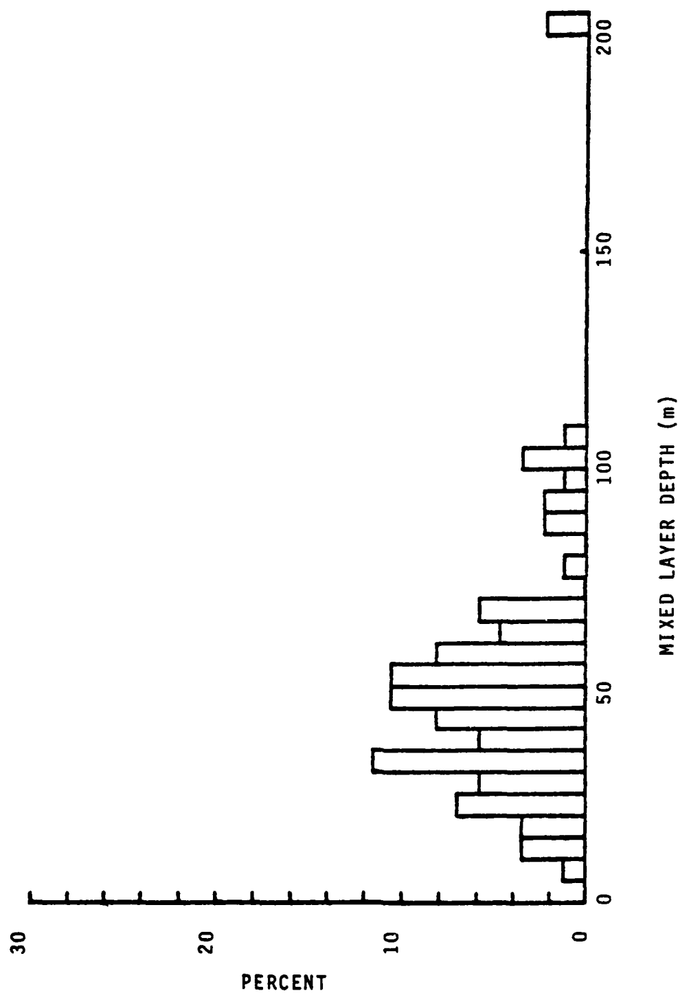
Figure 3.21 Histogram of MLD_c for All Seasons, Area II (86 Stations)
