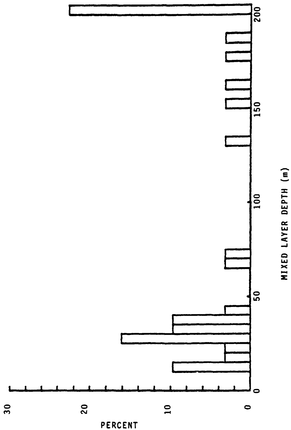
Figure 3.19 Histogram of MLD c for Spring, Area III (31 Stations)
