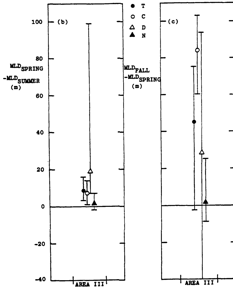
Figure 4.9 b) spring-summer. c) fall-spring. Note change of scale and large uncertainties of comparisons involving spring.
