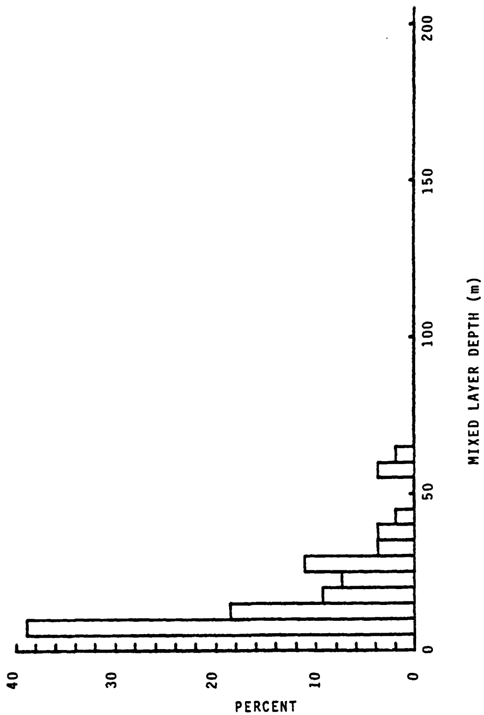
Figure 3.42 Histogram of MLD N for All Seasons, Area I (54 Stations)
