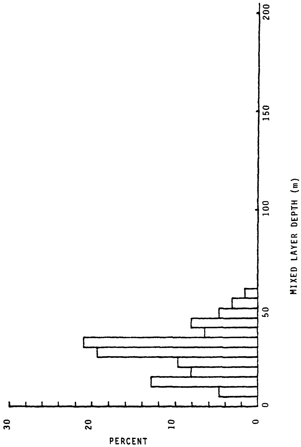
Figure 3.15 Histogram of MLD c for Summer, Area III (62 Stations)
