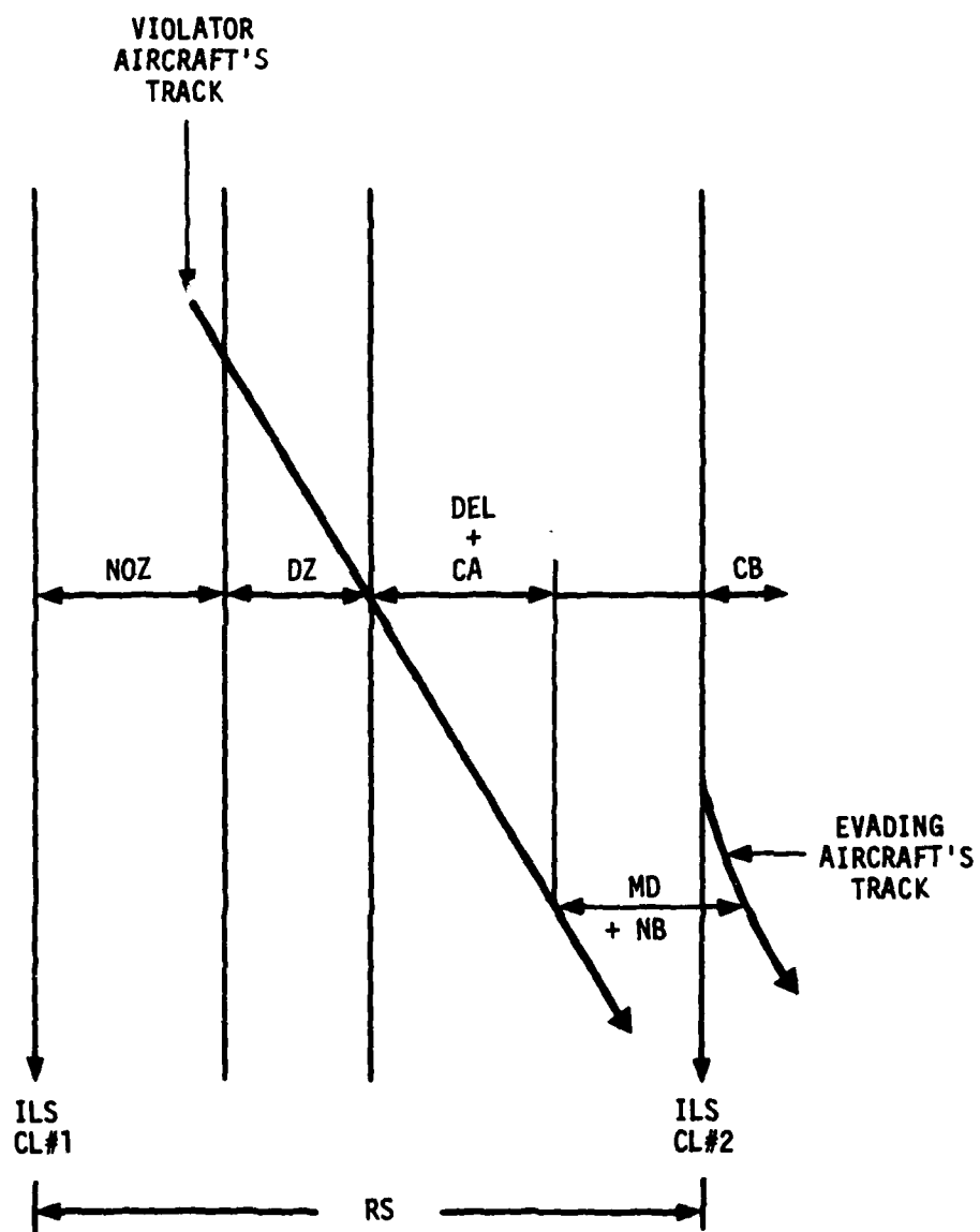
FIGURE B-5 SPACING BETWEEN AIRCRAFT (NOMENCLATURE)
