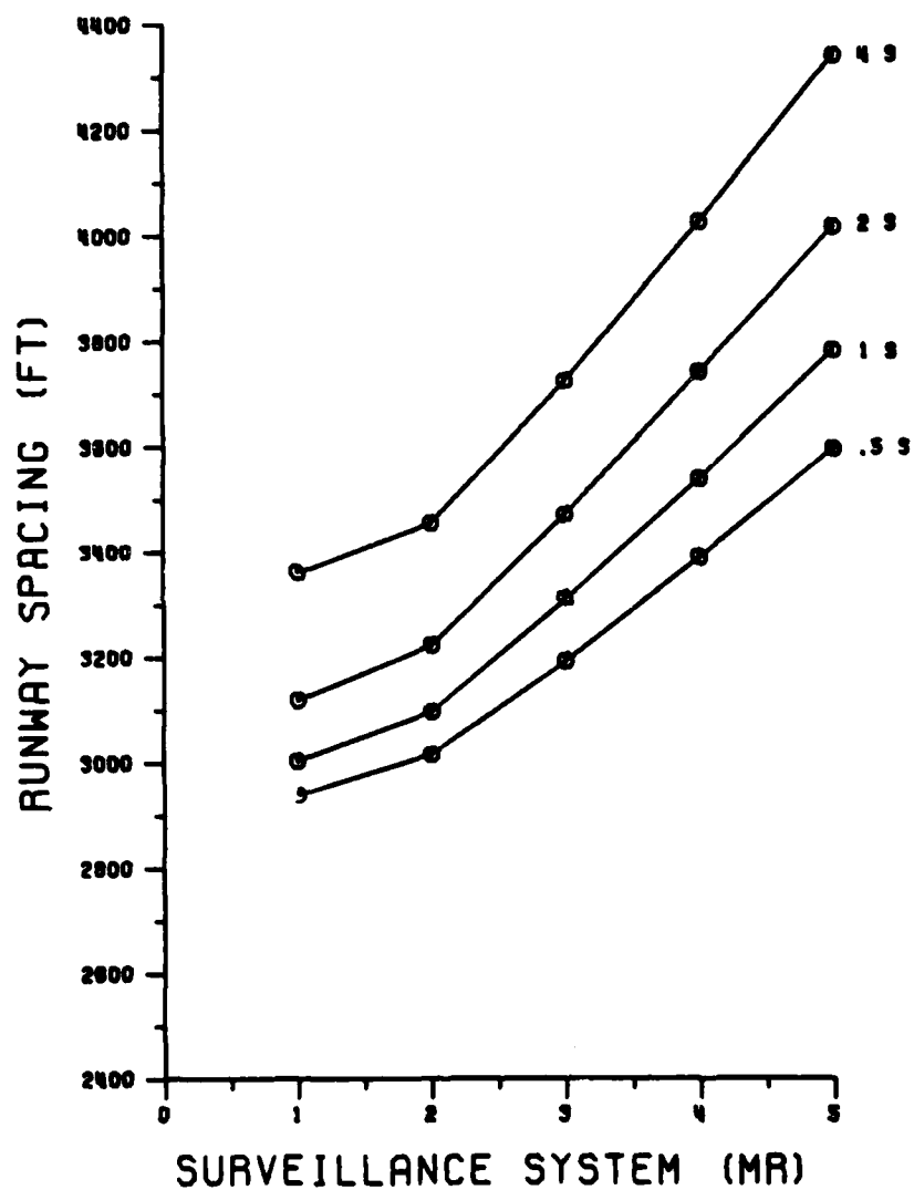
FIGURE C-1 RUNWAY SPACING—CASE #1
