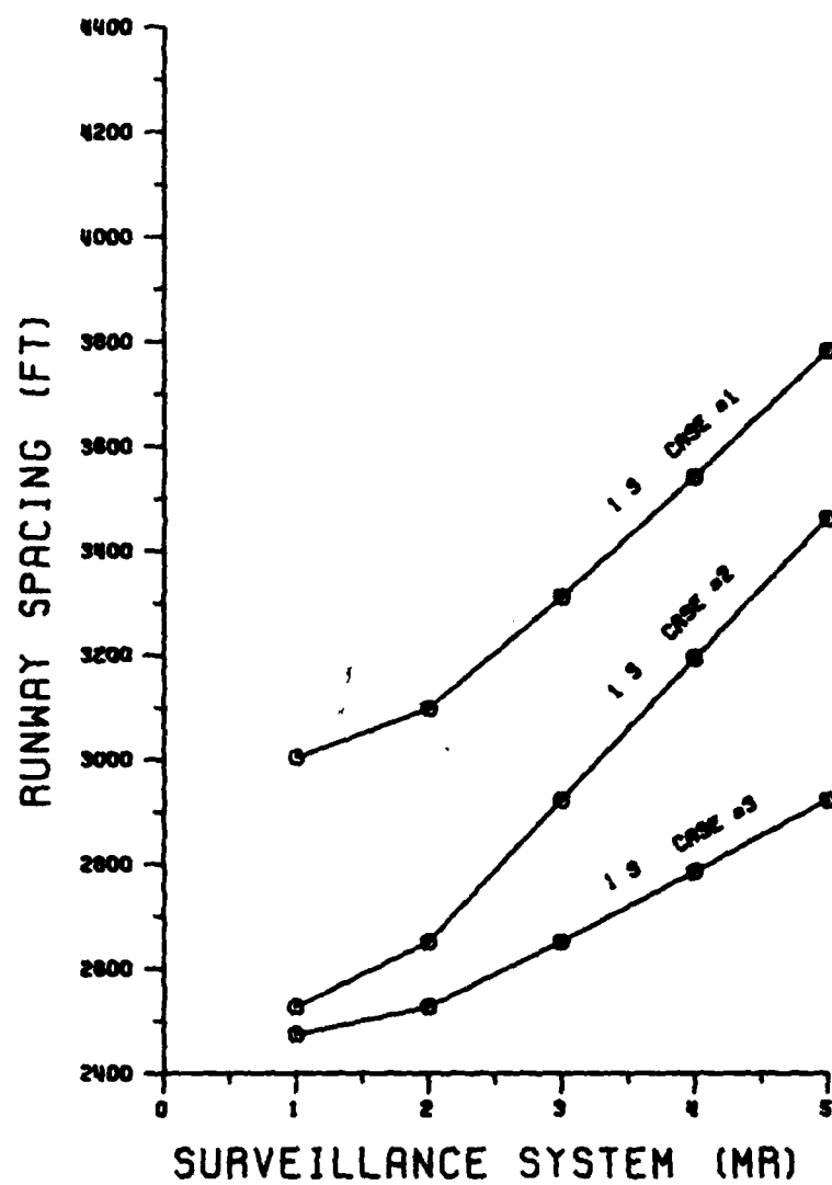
FIGURE 3-3 RUNWAY SPACING—1 s UPDATE
