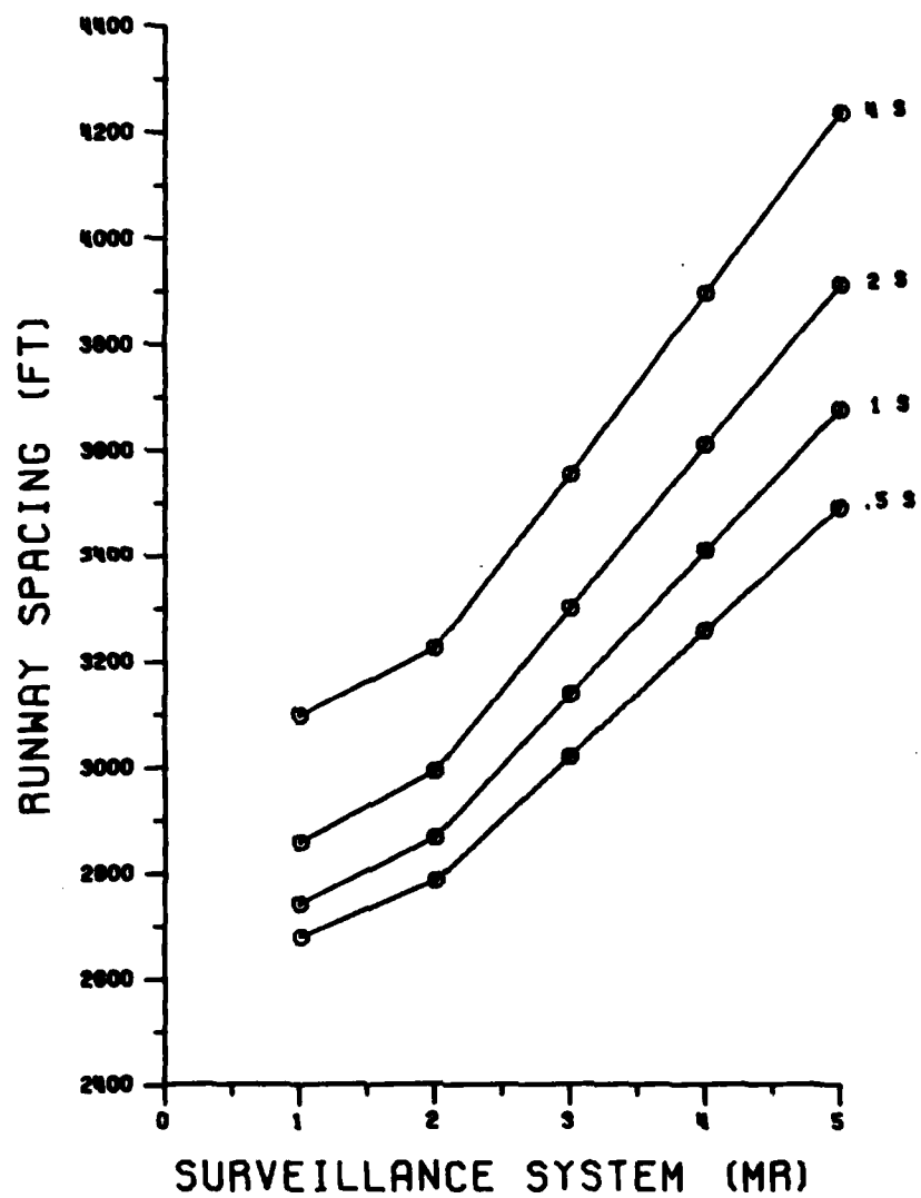
FIGURE C-5 RUNWAY SPACING—CASE #5
