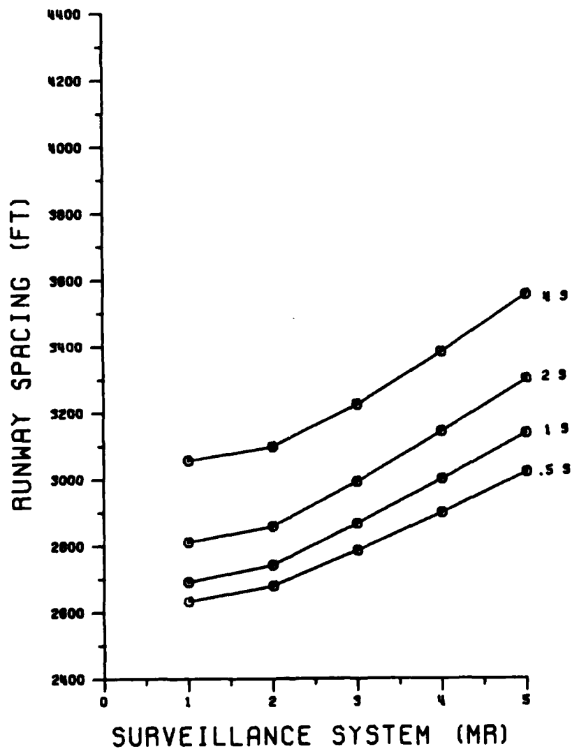
FIGURE C-8 RUNWAY SPACING—CASE #6
