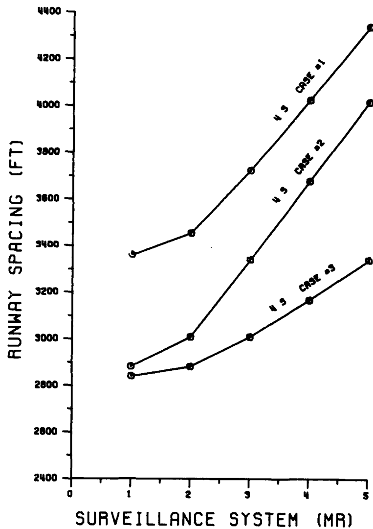
FIGURE 3-4 RUNWAY SPACING—4 s UPDATE
