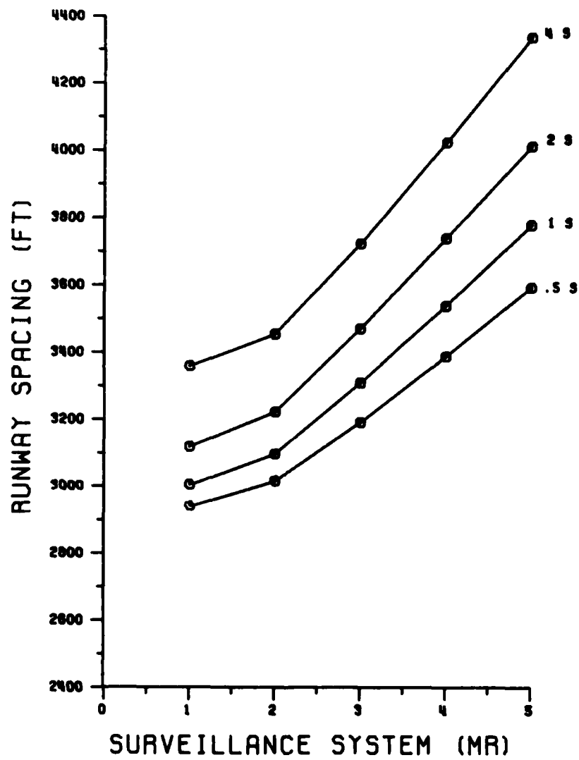
FIGURE 3-2 RUNWAY SPACING—BASELINE
