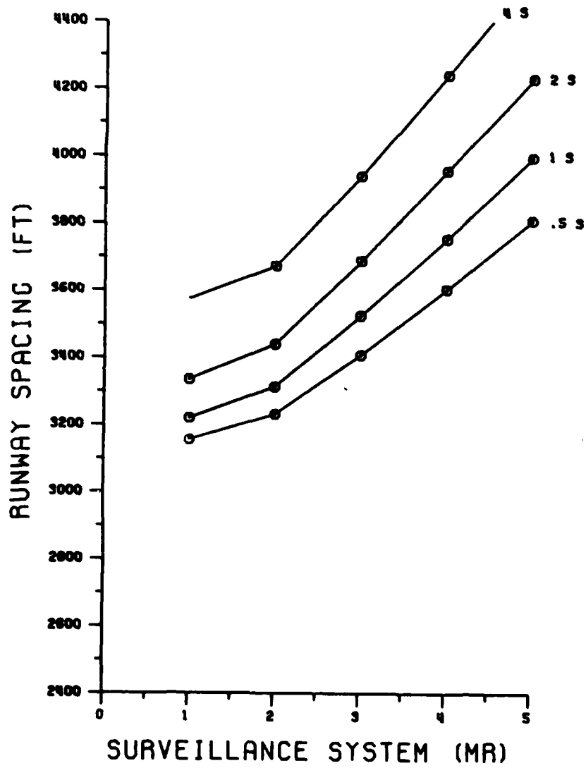
FIGURE C-4 RUNWAY SPACING—CASE #4
