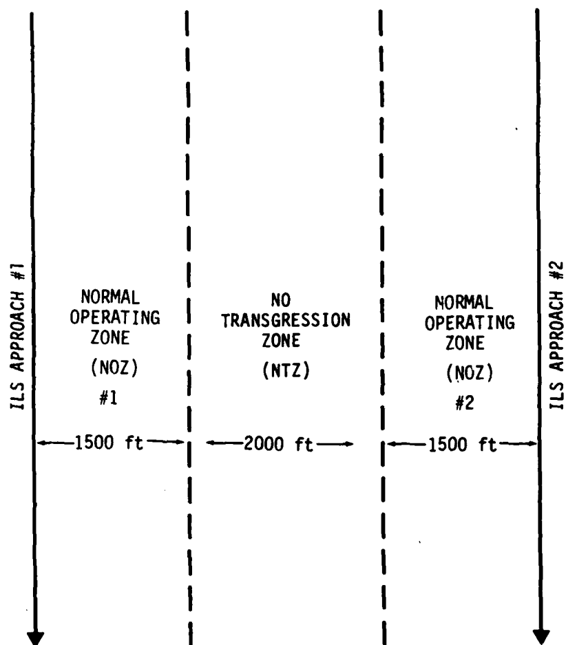
FIGURE 2-2 PARALLEL RUNWAY MONITORING ZONES
