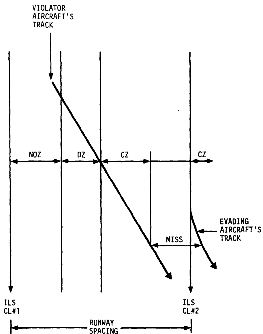
FIGURE B-4 SPACING BETWEEN AIRCRAFT
