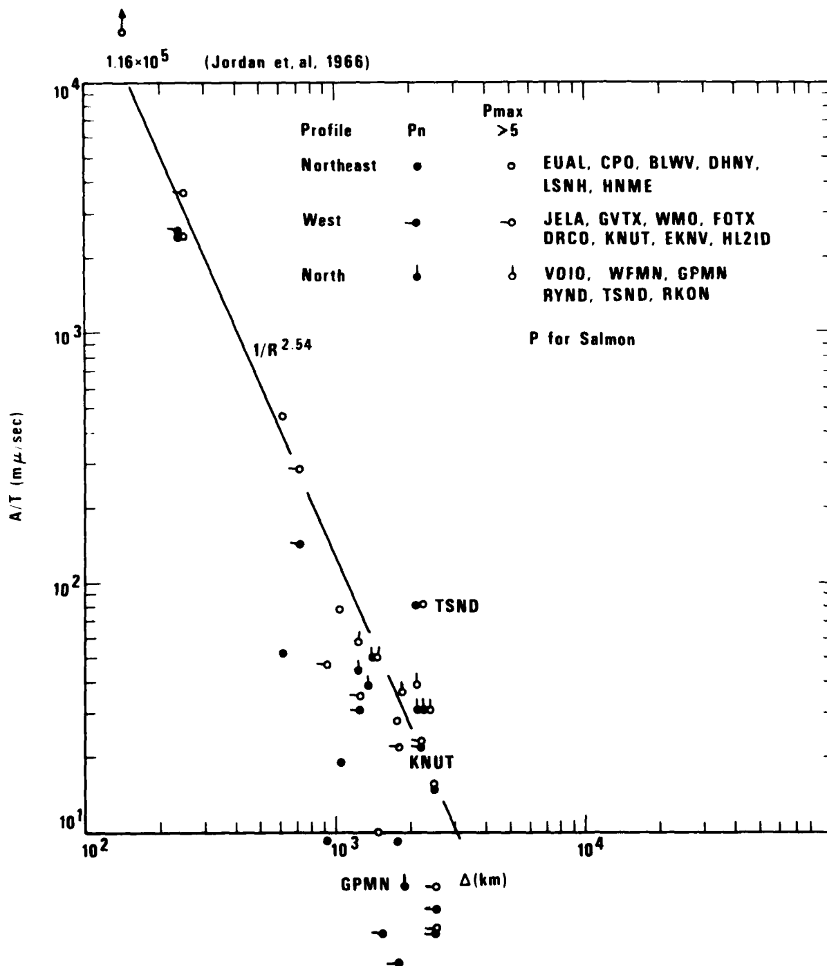
Figure 20. Amplitude-distance relations for the P and P max (phase velocity greater than 5 km/sec) phase from SALMON. A least-squares slope of -2.54 has been fitted to the P max data of the Northeast and North profiles. Note that most of the data along the Western profile fall well below the line.
