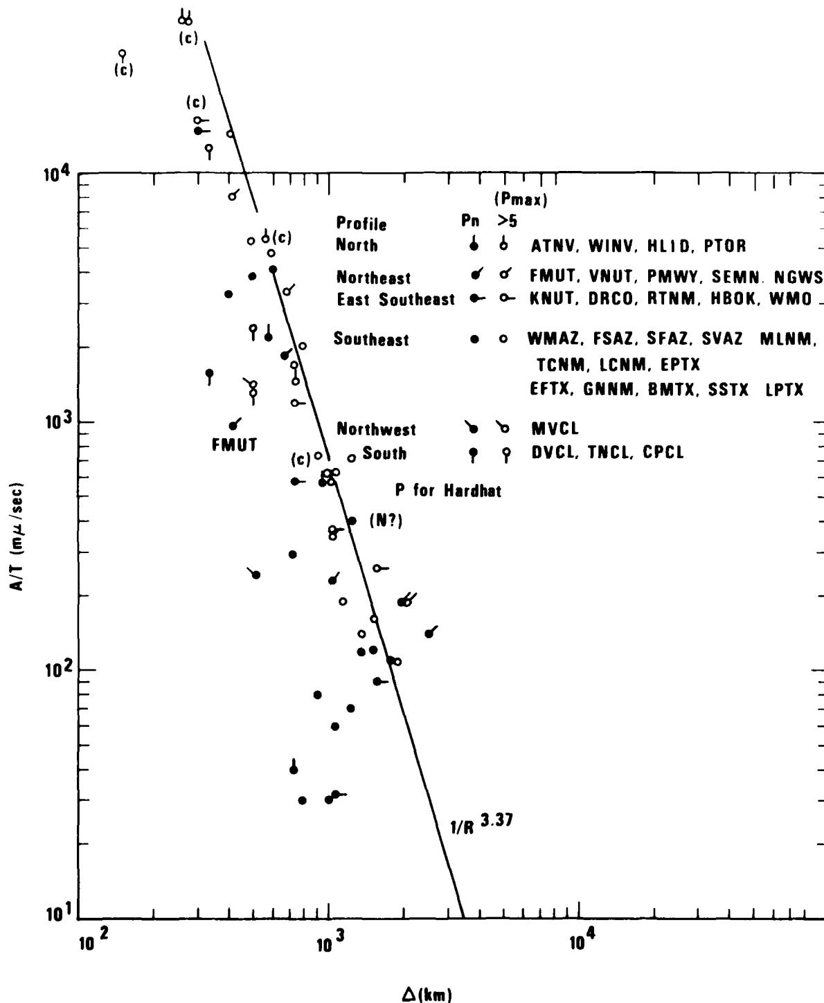
Figure 22. Amplitude-distance relations for the P and P max (phase velocity greater than 5 km/sec) phase from HARDHAT. A least-squares slope of -3.37 has been fitted to the P max data. Note that the P data is much more erratic. The notation (c) indicates that the data were clipped and that the true value, therefore, lies above the plotted point. (N?) indicates that the measurement may be noise.
