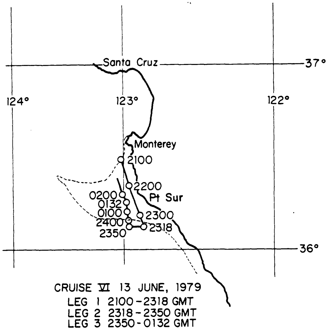
Figure 4. Track of the June '79 Cruise and outline of the upwelling feature based on satellite IR imagery.
