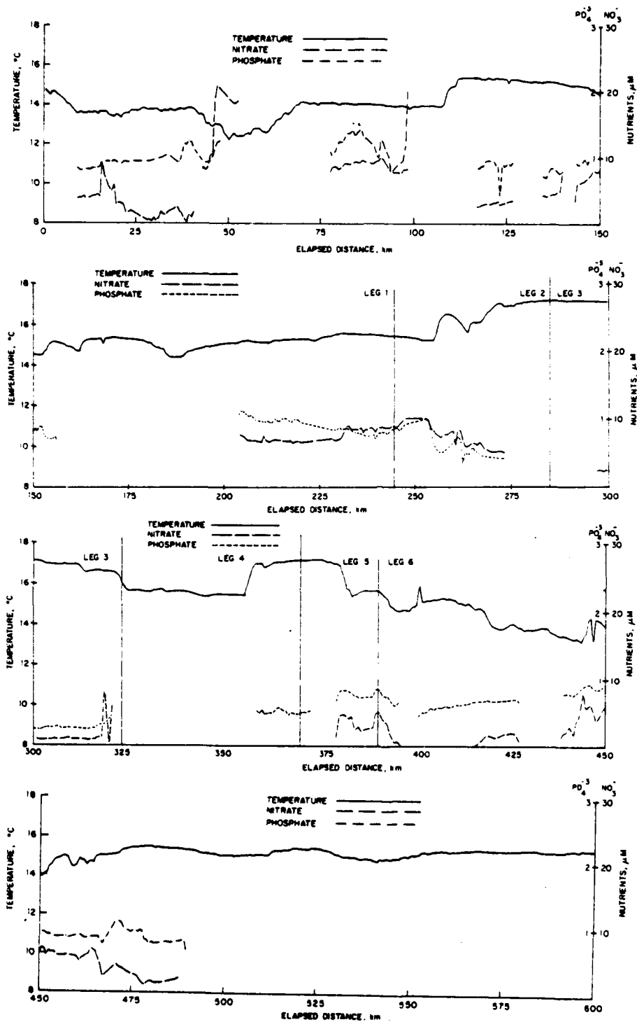
Figure 7. Nitrate, phosphate, and sea surface temperature versus elapsed distance along the track of the August '79 Cruise.
