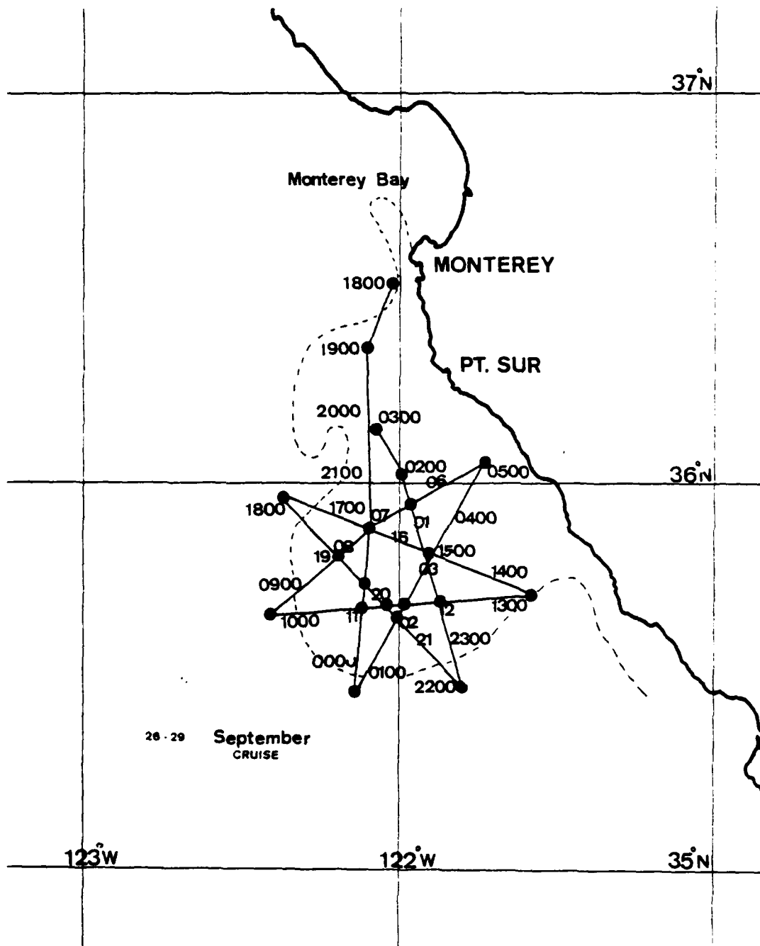
Figure 9. Track of the September '79 Cruise and outline of the upwelling feature based on satellite IR imagery.
