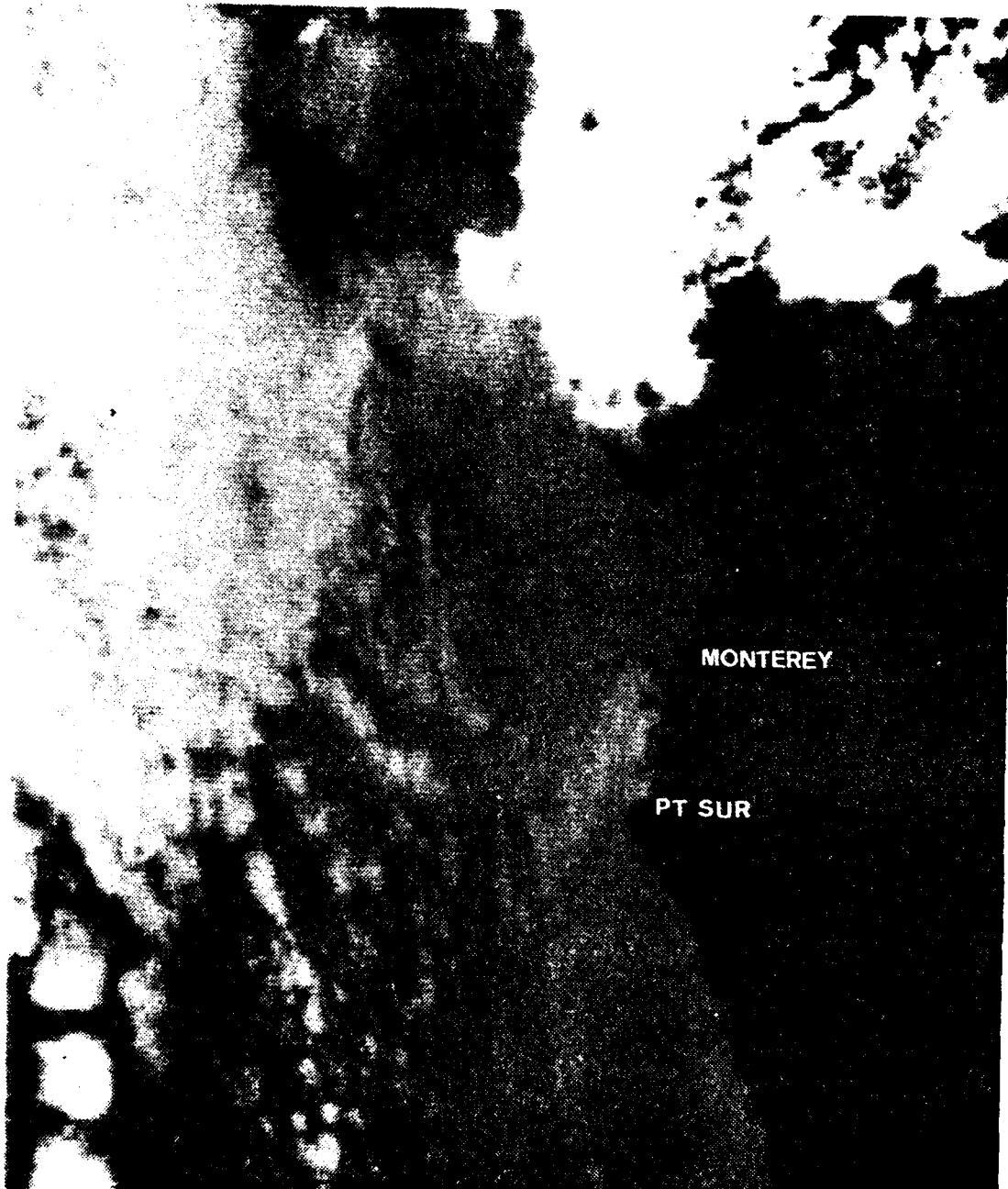
Plate 5. TIROS-N Satellite IR Image of the California Coast, 29 April 1979.
