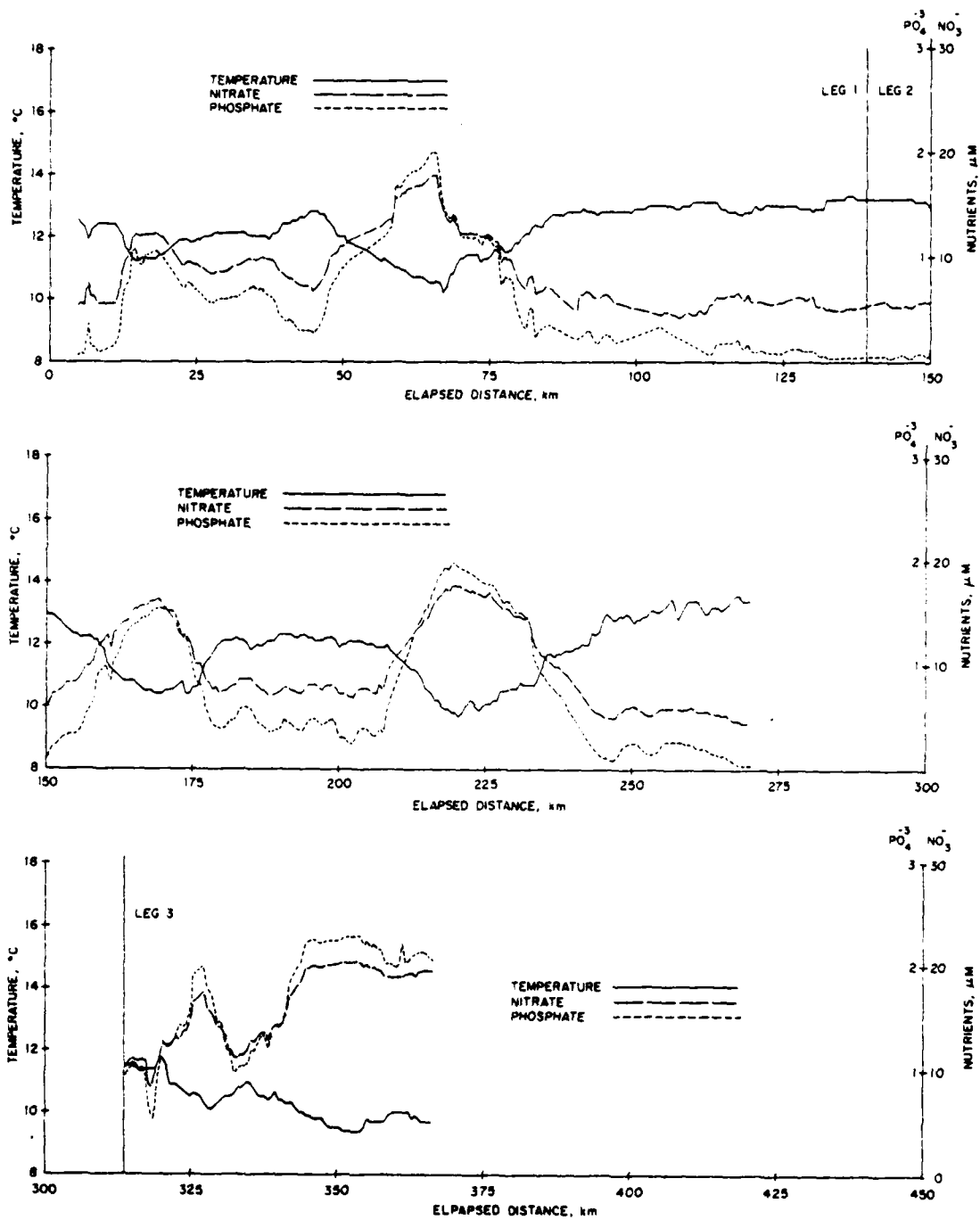
Figure 2. Nitrate, phosphate, and sea surface temperature versus elapsed distance along the track of the April '79 Cruise.
