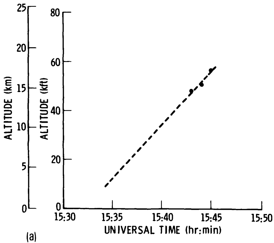
(a) Figure 8(a). Altitude of the leading edge of the northward surge as a function of time. The plotted points, though not well determined, do indicate the general altitude range. The dotted line is a simple linear extrapolation backward in time.
