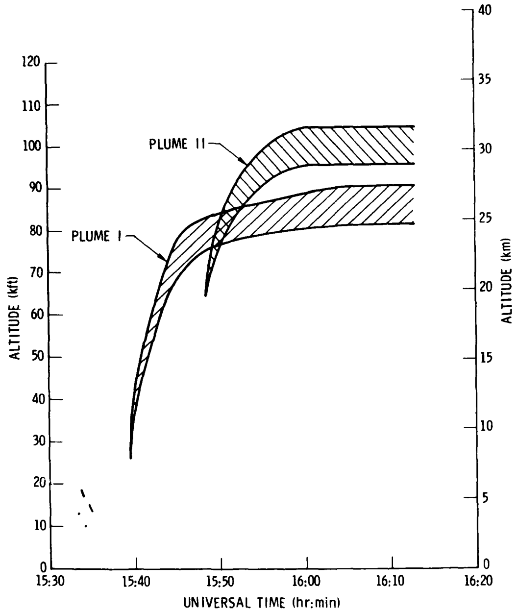
Figure 3. Peak altitude of the ash plumes based on triangulation.
