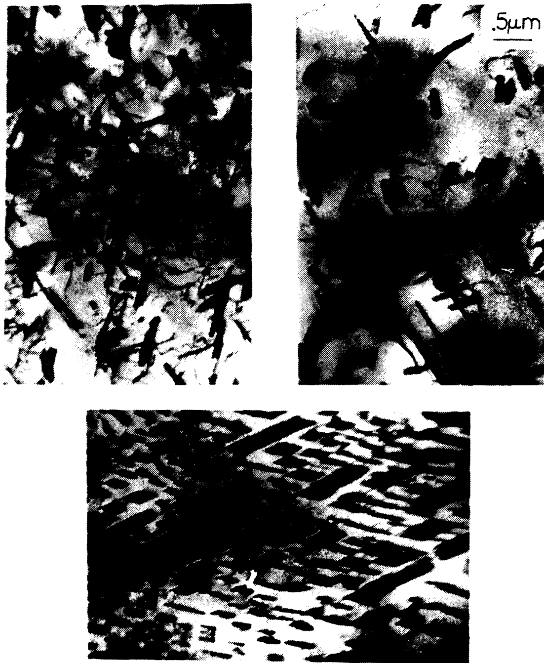
Figure 35. MIL65 - TEM Photo of Thin Foil
