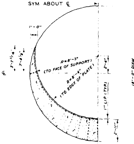
HALF SECTION UPSTREAM PLATE
