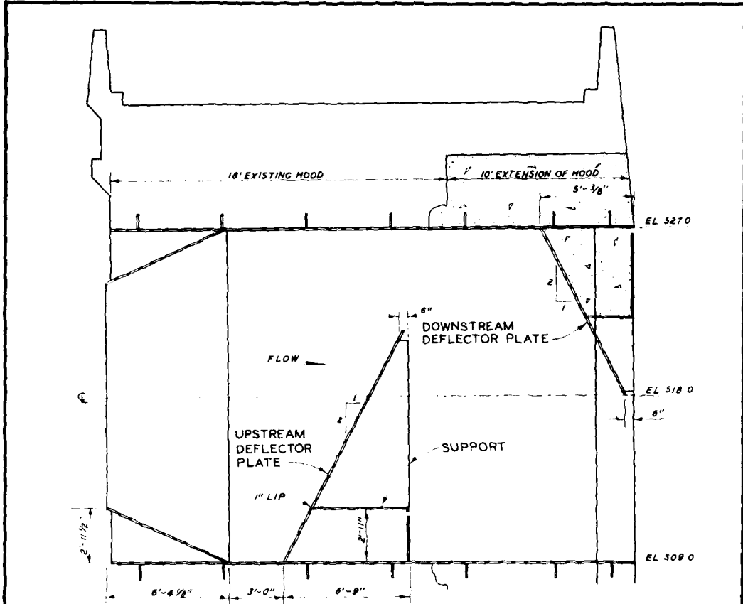
SECTION THROUGH CENTER OF HOOD
