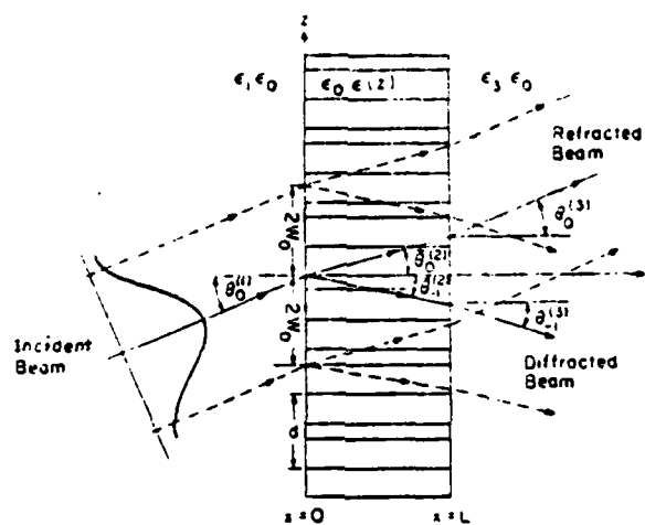
Figure 3. Bragg Diffraction Geometry (after Ref. 12)
