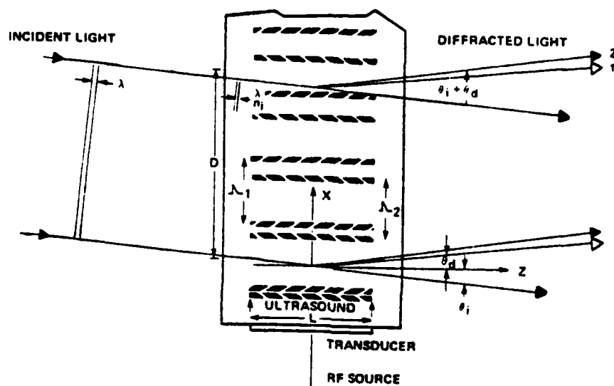
Figure 4. Bragg Cell Operation
