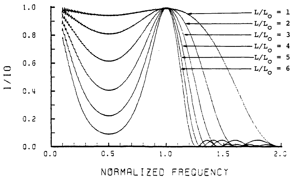
Figure 17. AOSA Implemented Diffraction Efficiency Bandshape
