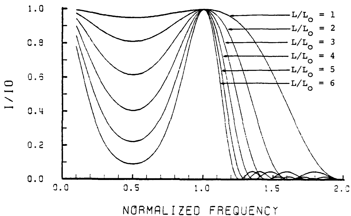
Figure 14. Diffraction Efficiency Bandshape (after Ref. 2)
