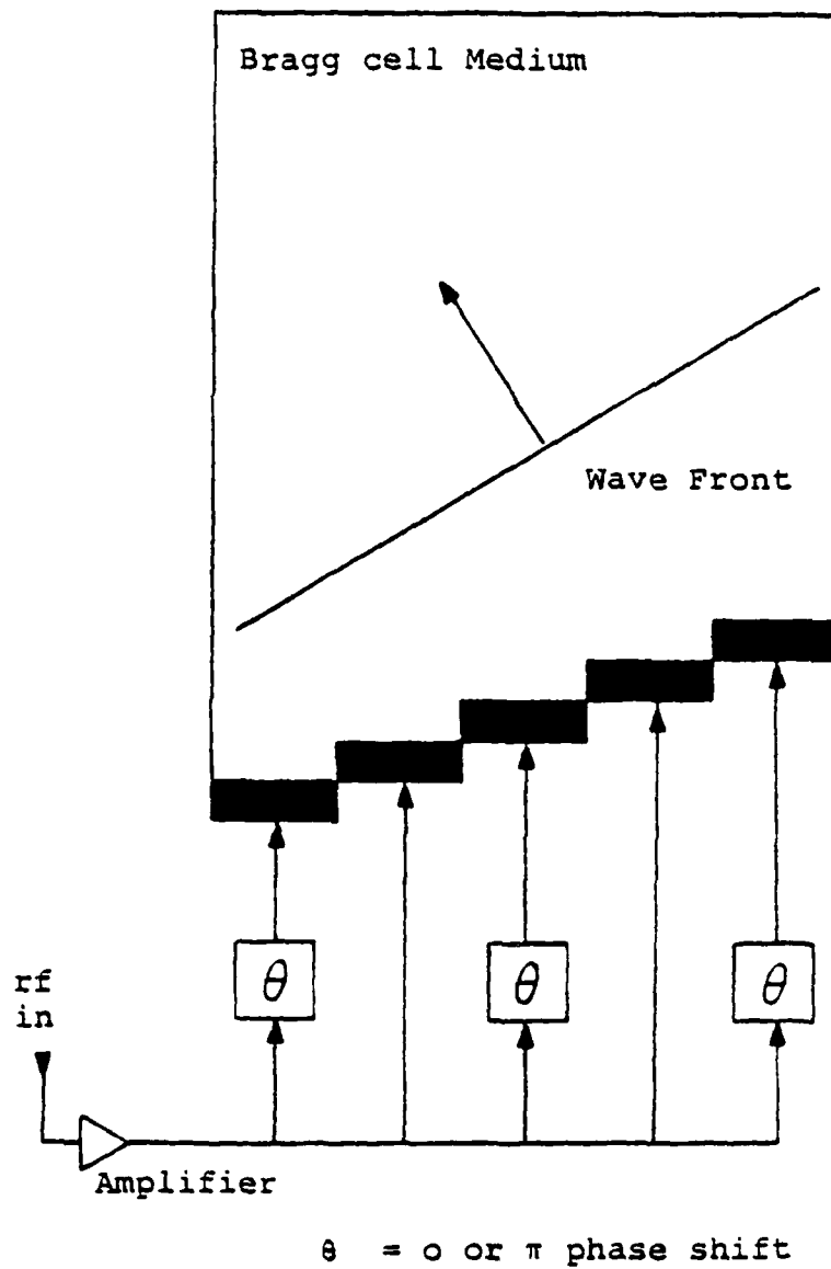
Figure 15. First-order Stepped Array Transducer
