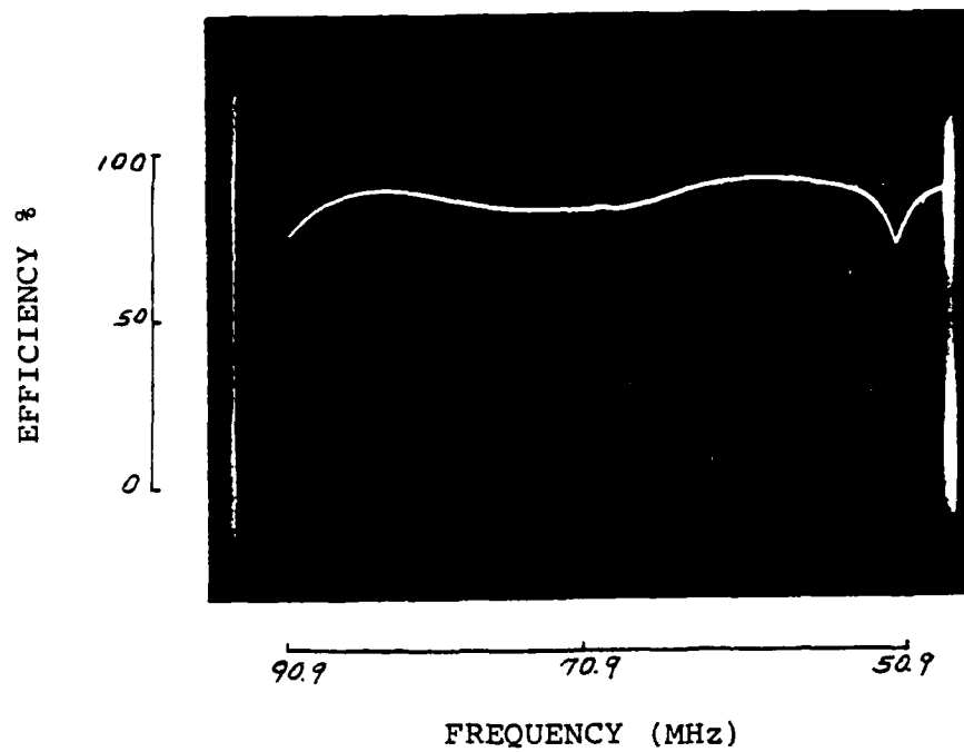
Figure 16. AOD-70 Bragg Deflector Efficiency Curve
