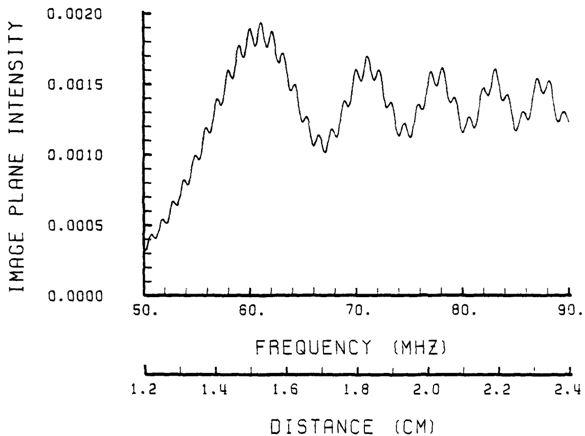
Figure 30. Image Plane Intensity Profile (Magnitude) Produced by a Linear Chirp with \Delta f_m = 80 MHz, f_o = 50 MHz, t = 2 \mu sec with an Incident Plane Wave o and a Stepped Array Transducer
