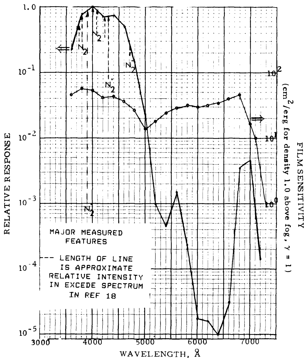
Figure 13. Relative spectral response of the monochrome (EK 2475 film) photometric camera with 5.7 mm f/1.8 lens. The sharp falloff above 4600 \text{\AA} results from the attenuation by its 1\frac{1}{2} mm thick BG-12 Schott filter. Response at wavelengths below 3900 \text{\AA} is limited by lens absorption and at wavelengths beyond 7000 \text{\AA} by the falloff of the film's sensitivity (circles).
