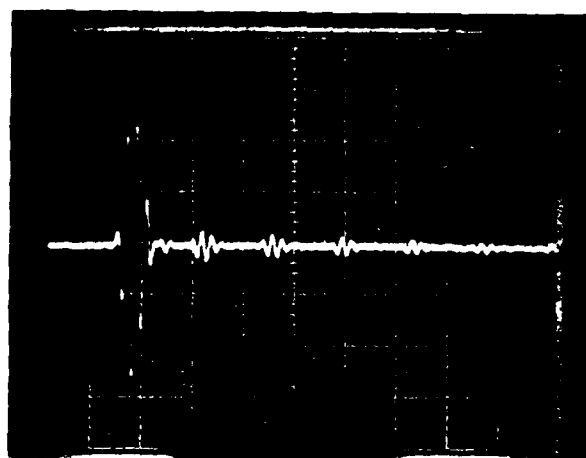
Figure 4. Echoes From .128" Thick Copper Plate, Laid on the Bottom of the Plastic Pan. Sweep Rate 1 \mu\text{s}/\text{cm} .
