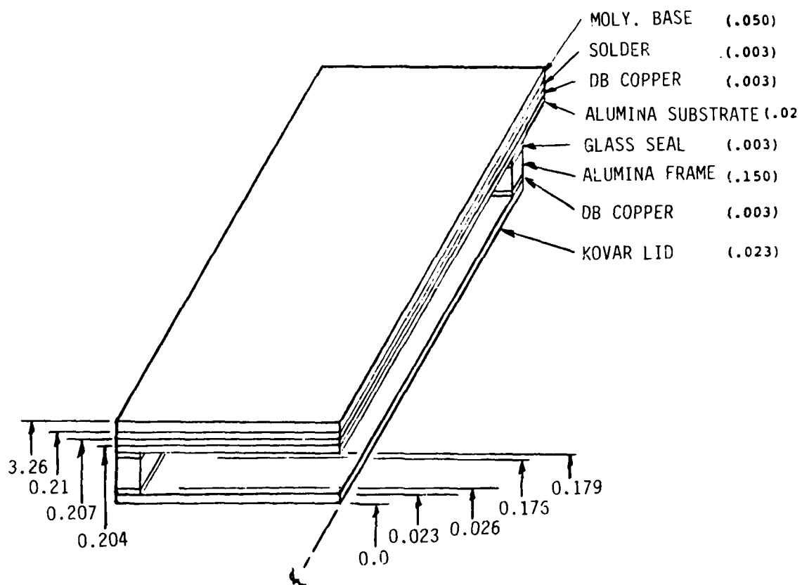
Figure 10. Section of 100W RF P.A. Module
