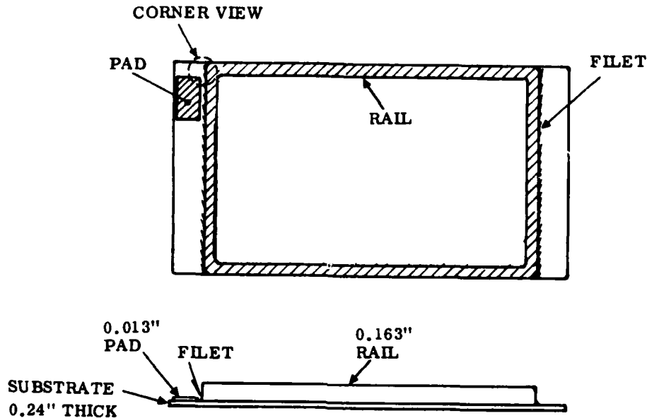
Figure 1. Circuit Assembly Dimensions
