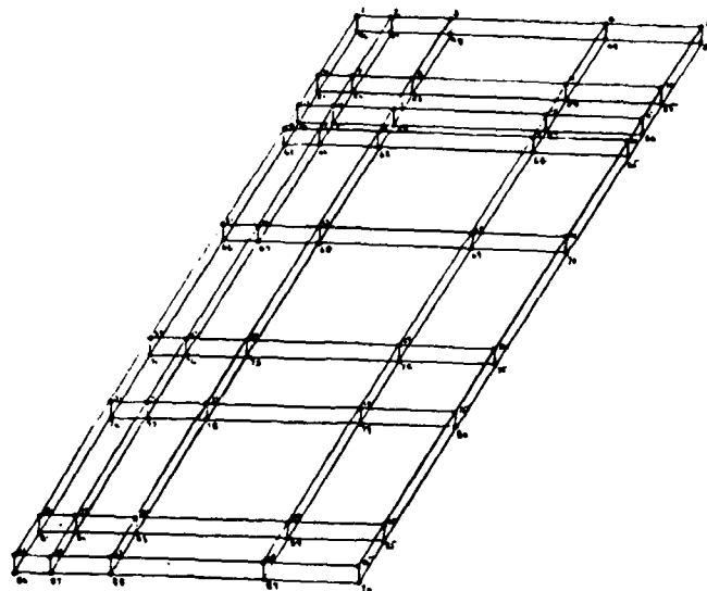
Figure 11. Finite Element Model (Moly Base)
