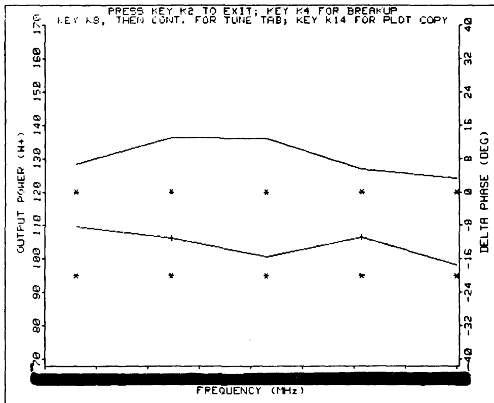
Figure 34. Typical Mach Plot of f/Output Power Vs Delta Phase
