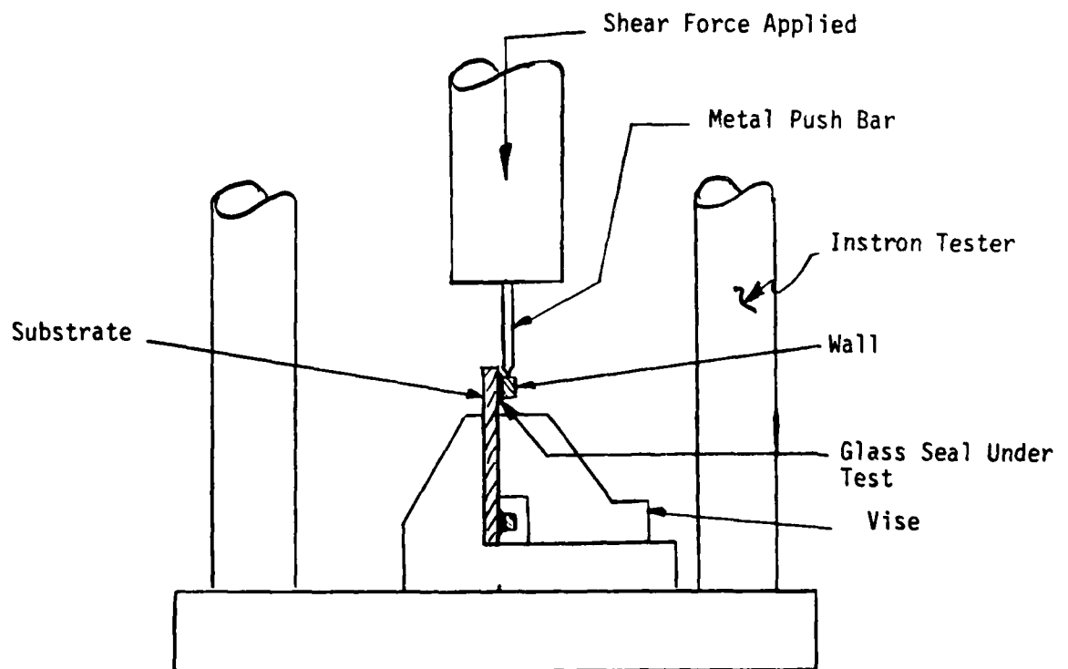
Figure 8. Test Set-Up
