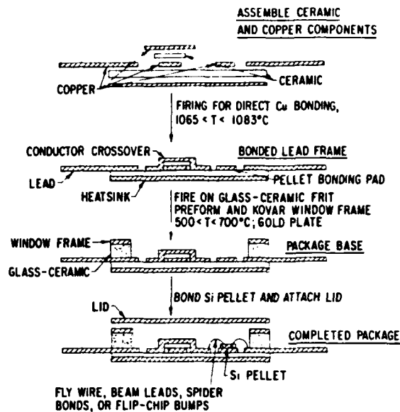
Fig. 5 Process steps to fabricate electronic package by direct bonding process.
