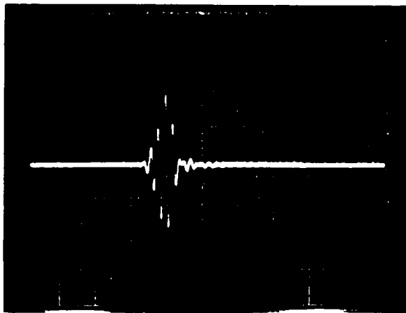
Figure 10. Echo From .0135" Dimpled Projection on Brass Shim. 1 \mu s/cm . Delay has not been Altered from Test of Figure 9.
