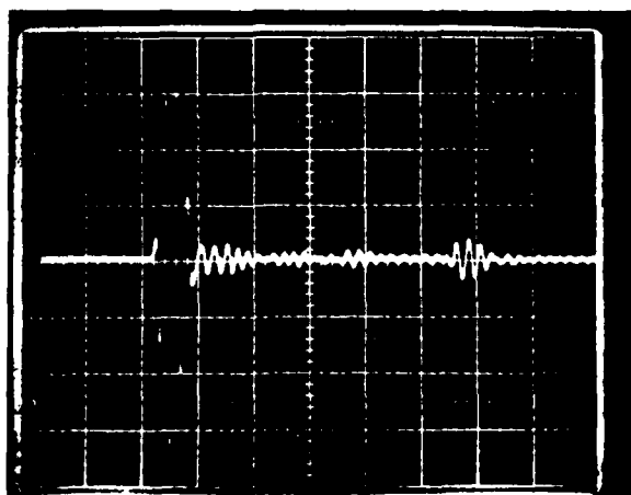
Figure 14. Echoes From Ceramic Rail of Circuit Board, (2.2 cm), Lying on Cu Plate (7.6 cm). Sweep Rate 1 \mu\text{s}/\text{cm} .
