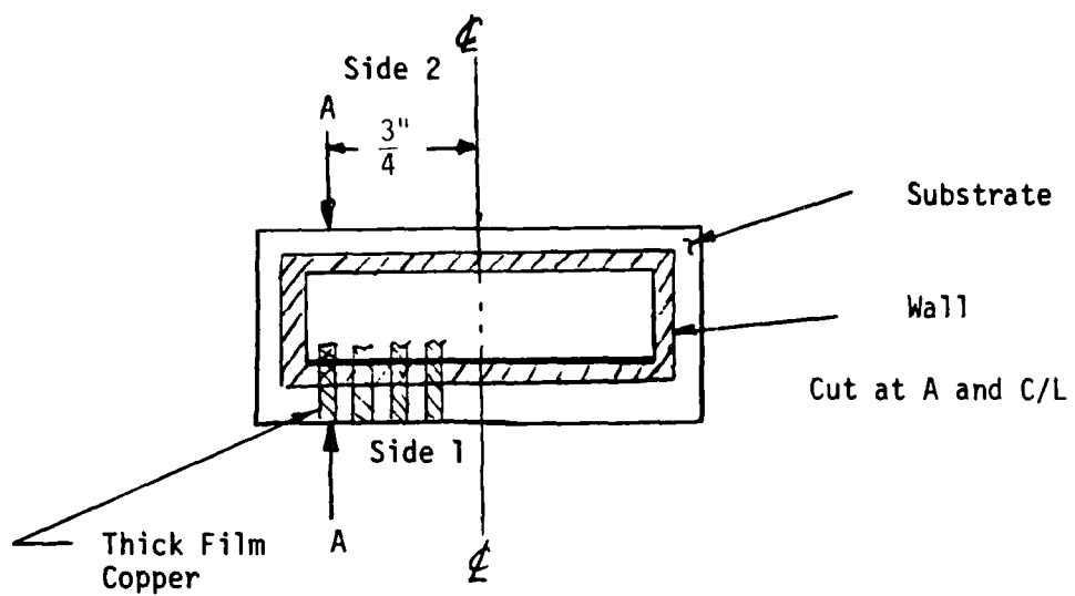
Figure 7. Shear Test Specimen
