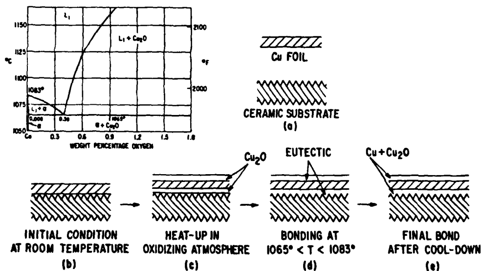
Fig. 2 Eutectic phase diagram and schematic of bonding process.
