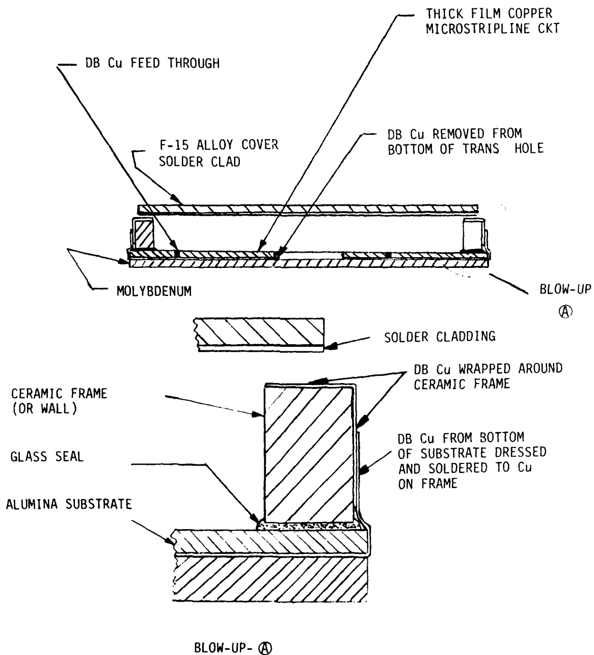
Figure 2. Cross-Section RF 100 W Power Module
