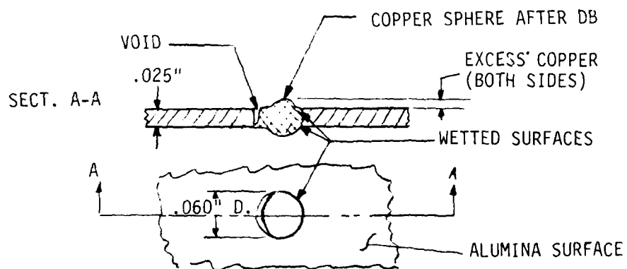
Figure 5. 0.055 In. Diam. Copper Sphere - Void Free Fill
