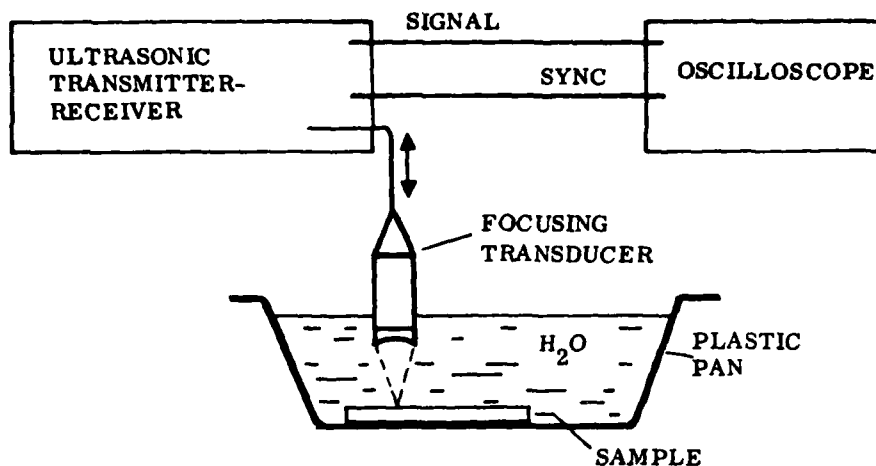
Figure 2. Test Equipment Schematic
