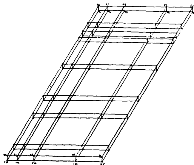
Figure 12. Finite Element Model (Solder)
