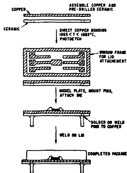
Fig. 6 Process steps to fabricate electronic package by direct copper bonding process.
