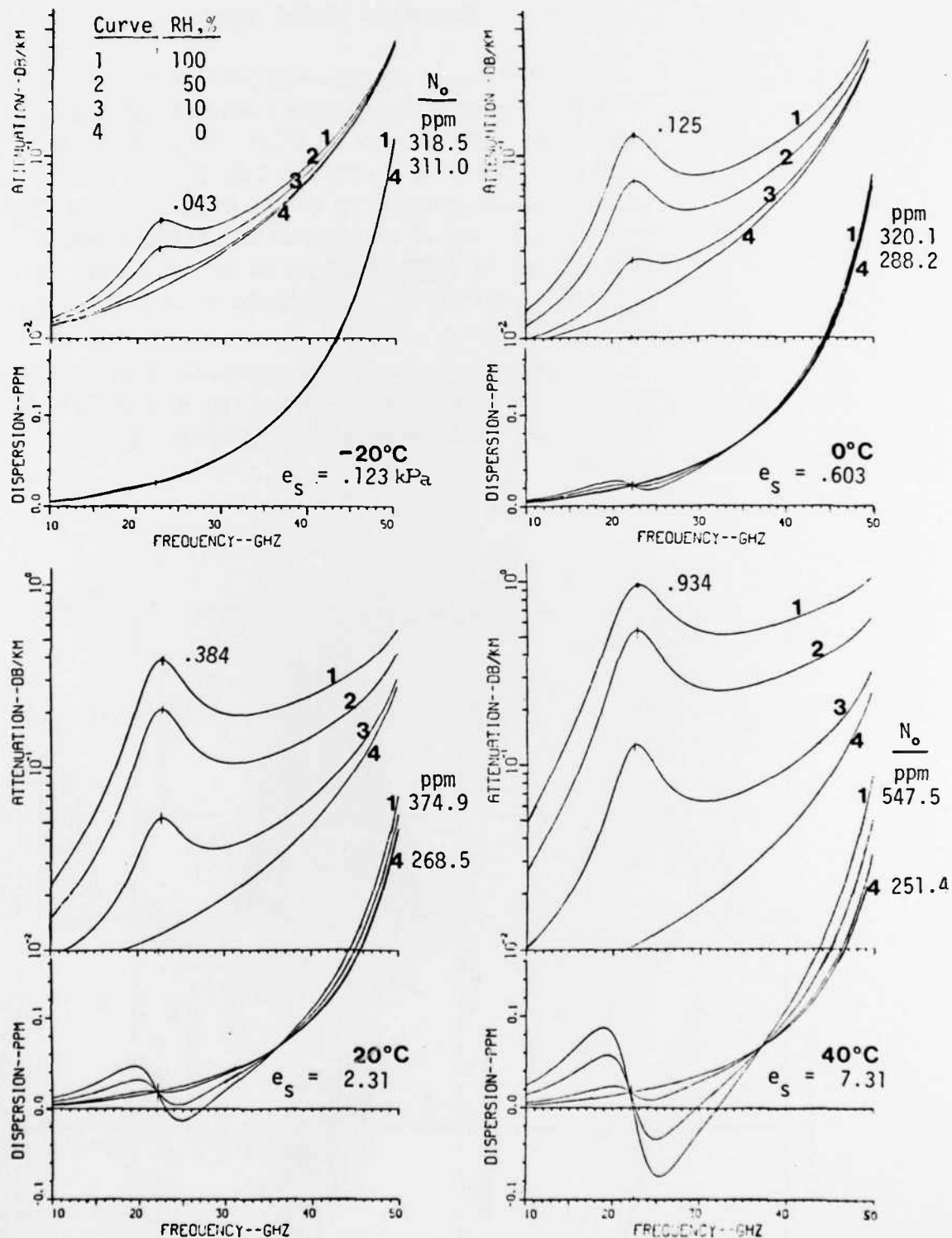
FIG. 3. ATTENUATION \alpha IN DB/KM, REFRACTIVITY N_0 , AND REFRACTIVE DISPERSION D IN PPM FOR DRY ( RH = 0\% ) TO SATURATED ( RH = 100\% ) AIR AT SEA LEVEL, h = 0 \text{ KM} AND TEMPERATURES, T = -20^\circ\text{C} TO +40^\circ\text{C} OVER THE FREQUENCY RANGE 10 TO 50 GHz.
