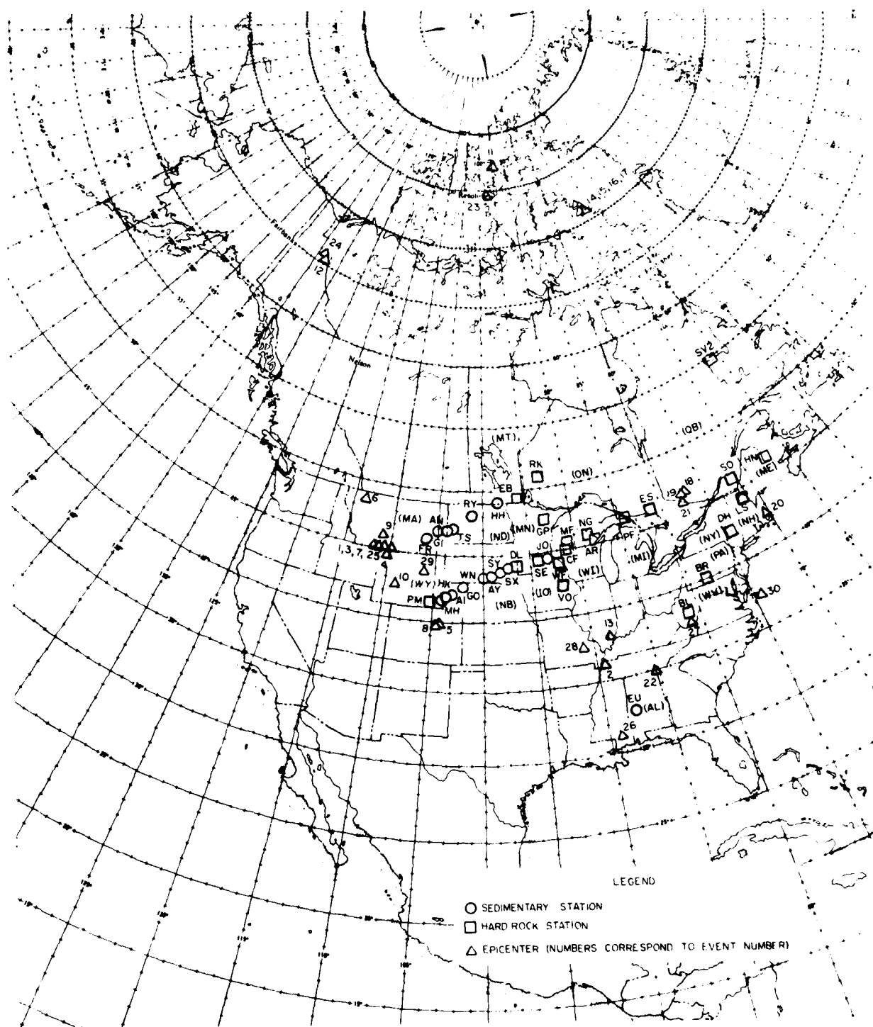
Figure 1 Stations used to investigate amplification of regional phases at sedimentary sites (circles) relative to hard rock sites (squares) located on the shield or stable platform region of North America. Triangles denote the locations of events studied.
