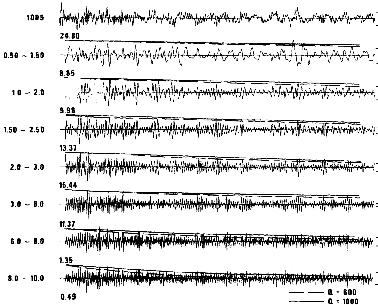
Figure 27b Band pass filtered codas of L at RKON with the theoretical coda shapes for Q = 600 and Q^g = 1000 . Bars show background noise levels.
