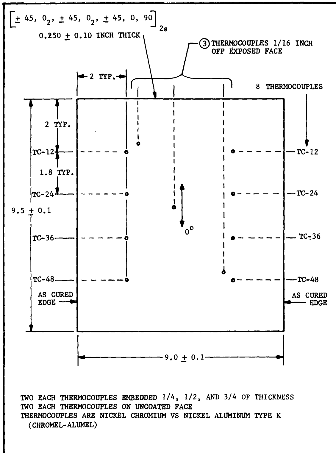
Figure 1. Thermocouple Arrangement for Transit Measurements
