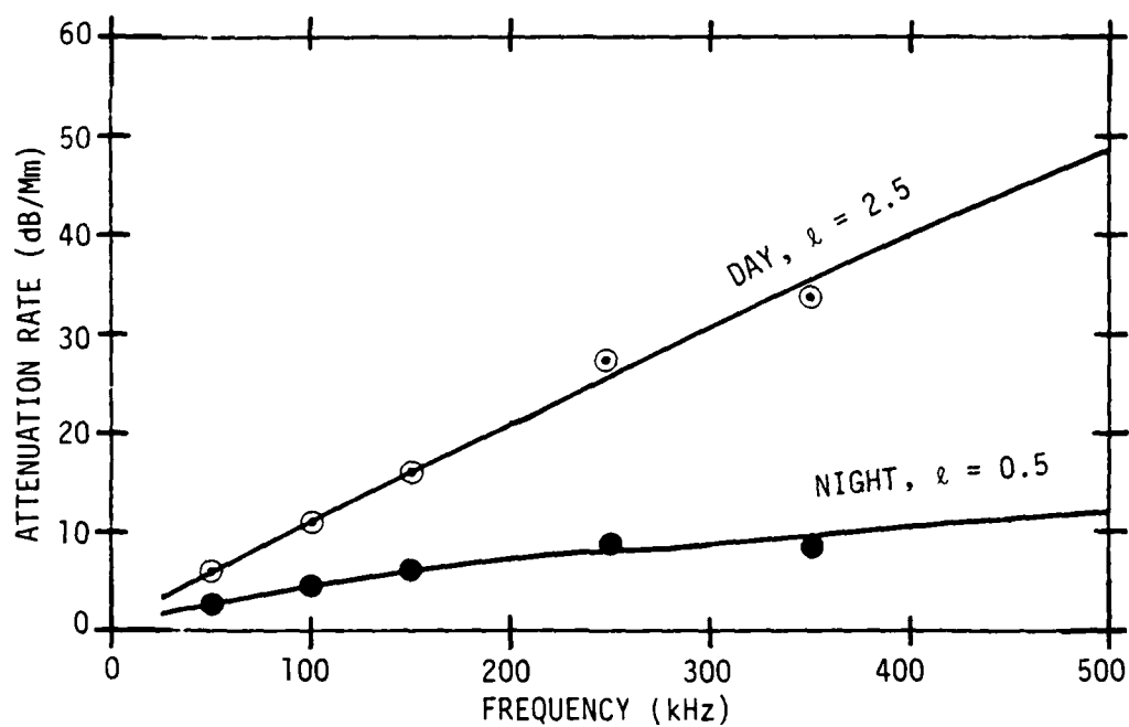
Figure 7. Comparison of Attenuation Rate Versus Frequency (Daytime \ell = 2.5 km and Nighttime \ell = 0.5 km)
