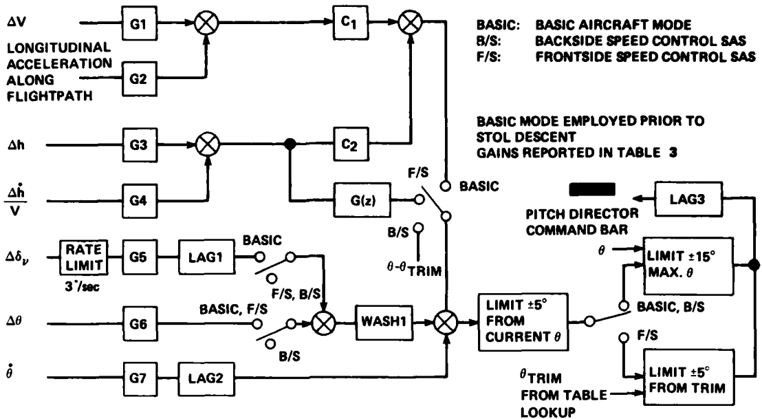
Figure 22. - Pitch flight director.
