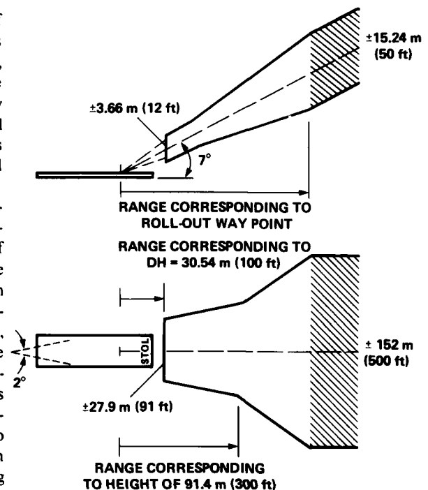
Figure 17.— Scheduled dimensions of path deviation window.
