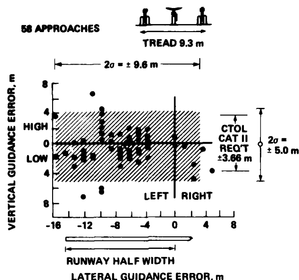
Figure 43.— Guidance errors at pilot's decision height.
