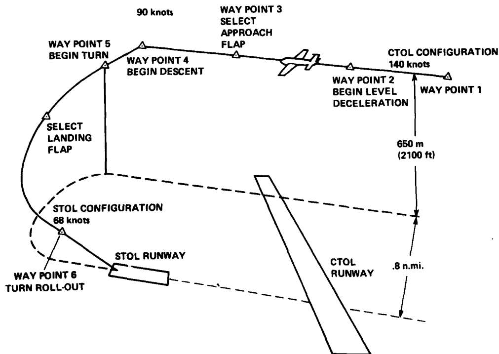
Figure 1.— STOL approach profile.
