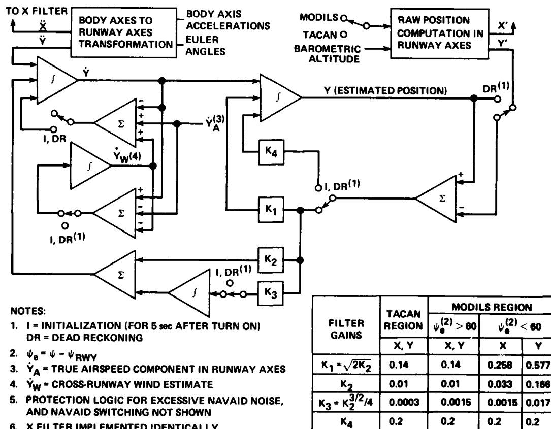
Figure 12. — X and Y complementary filters.
