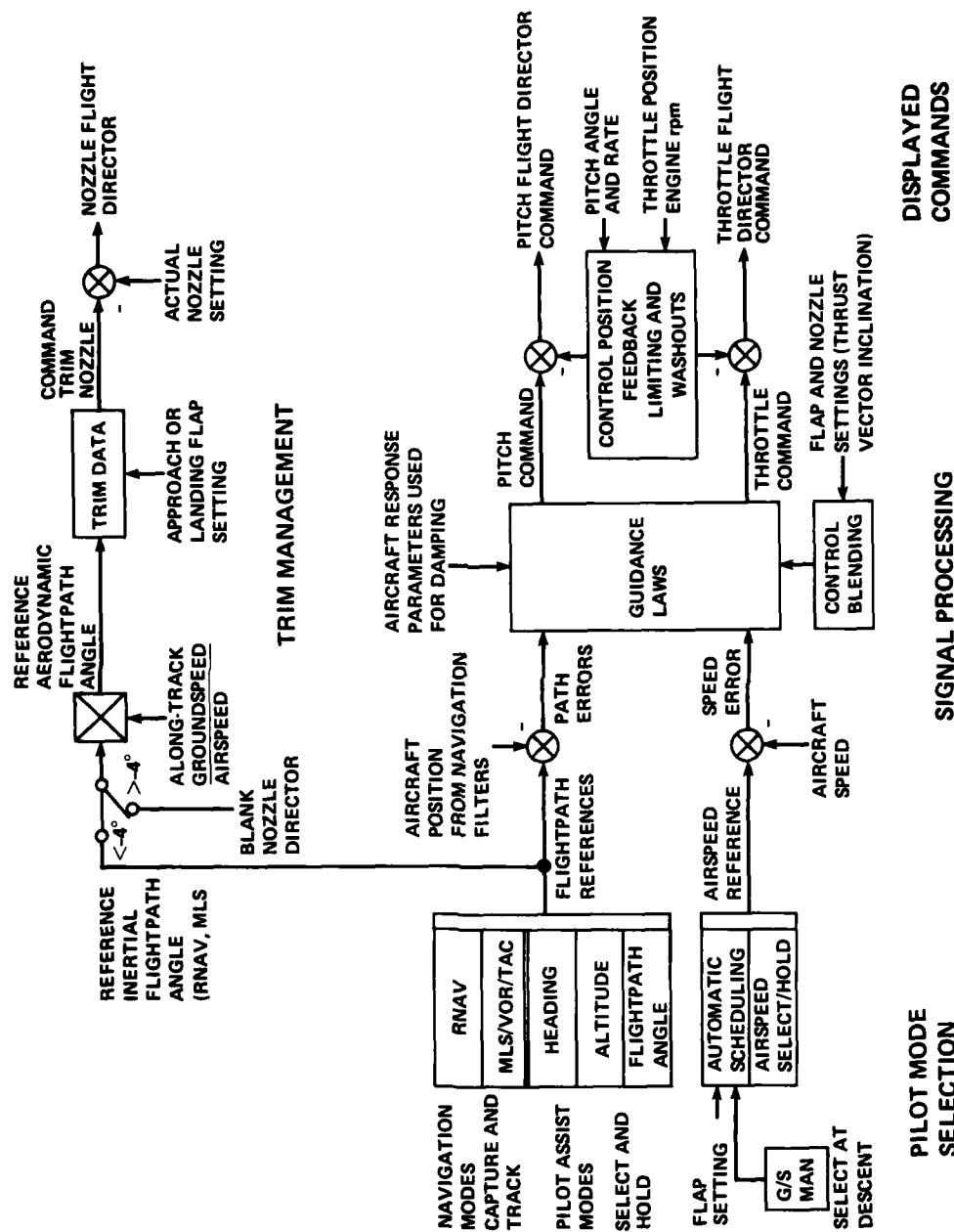
Figure 19. Flight director functional design.
