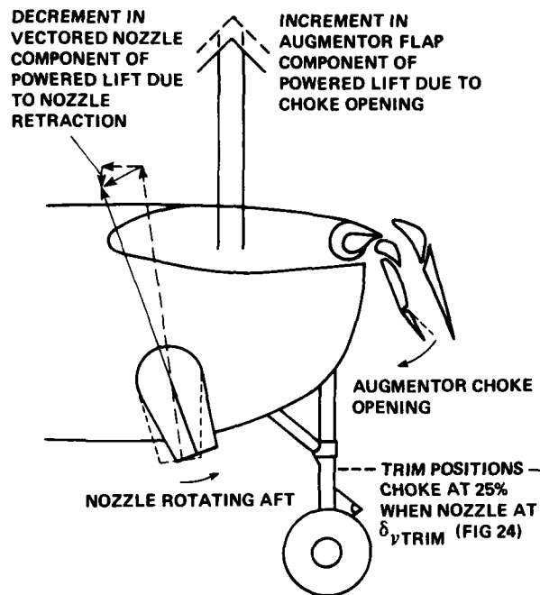
Figure 9.— Nozzle-choke gearing.
