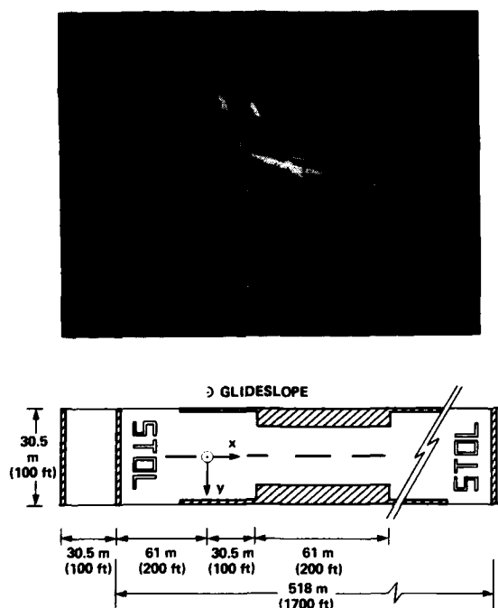
Figure 26. -- Crows Landing Test Facility, STOL runway and coordinate system.
