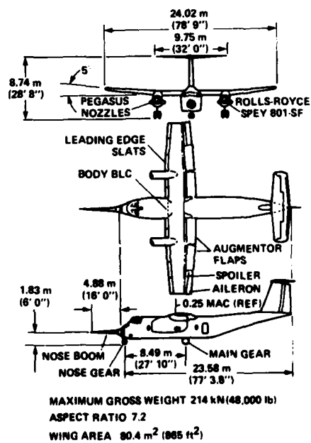
Figure 2. – Augmentor Wing Jet STOL Research Aircraft.
