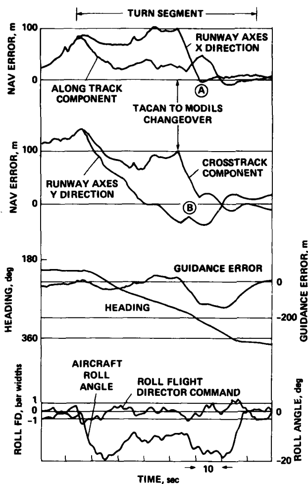
Figure 36.— Typical lateral transient due to NAVAID switching.
