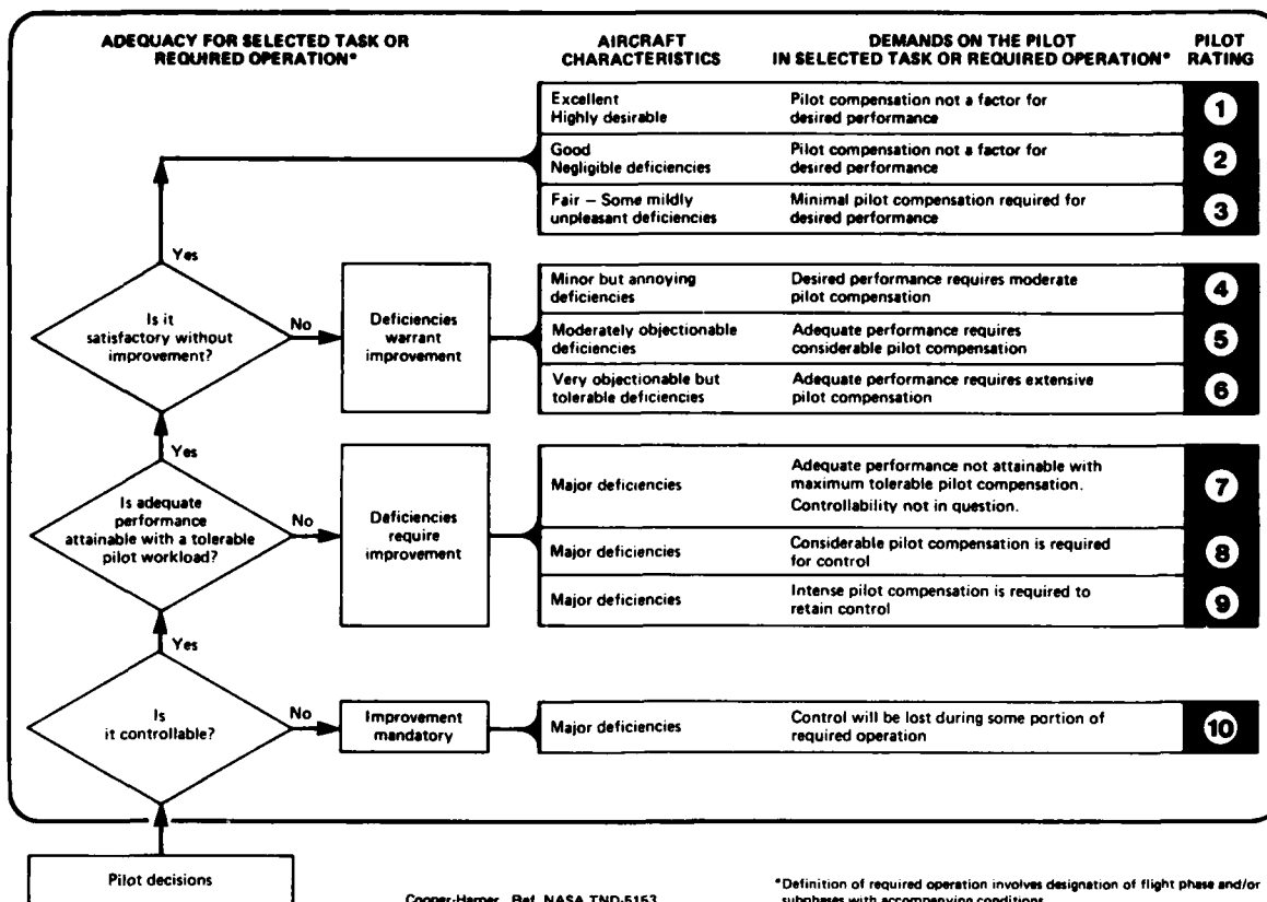
Figure 54.— Handling qualities rating scale.
