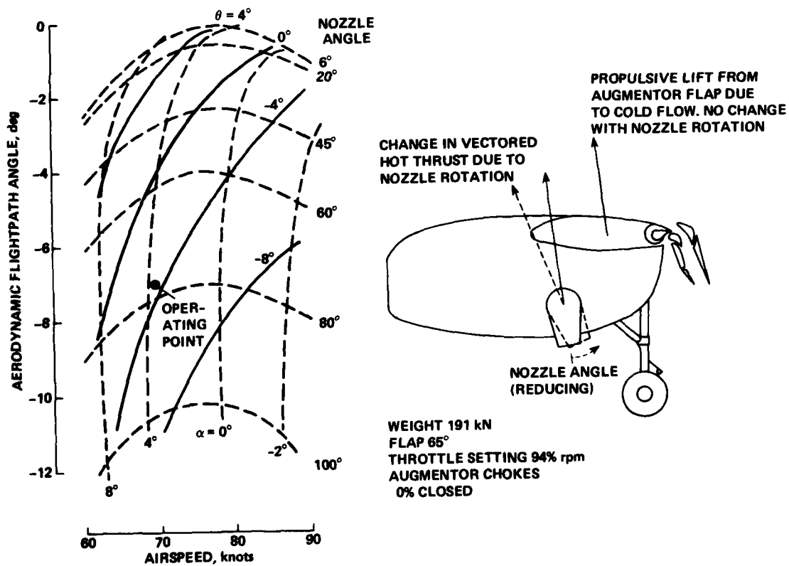
Figure 6.— Descent trim conditions, throttle fixed.
