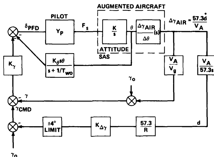
Figure 61.— Closed-loop glidepath tracking system using pitch attitude control.
