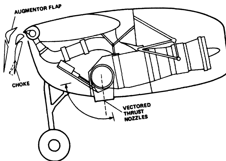
Figure 3.— Augmentor wing propulsive lift system.
