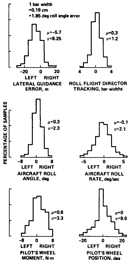
Figure 46.— Lateral performance and control parameters during final 30 sec of approach.
