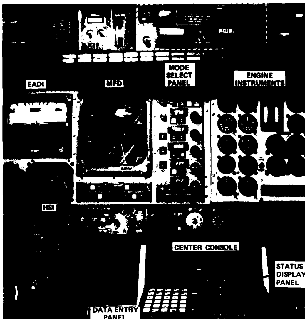
Figure 14.-- Cockpit displays.
