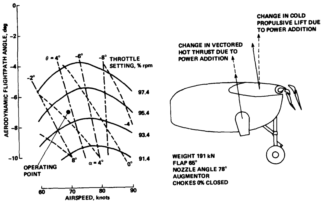
Figure 5.— Descent trim conditions, nozzles fixed.
