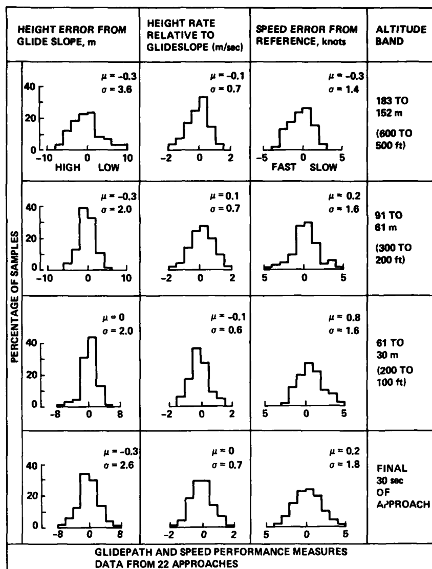
Figure 64. — Glidepath and speed performance measures using the improved throttle flight director control laws.
