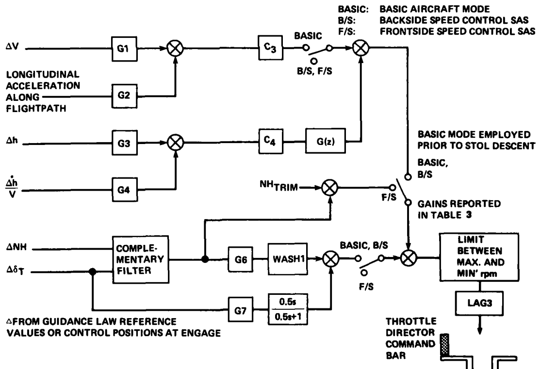
Figure 23. - Throttle flight director.
