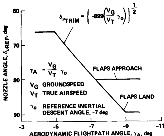
Figure 24.— Trim nozzle calculation.
