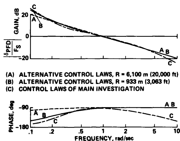
Figure 62.— Controlled element dynamics for pitch flight director.
