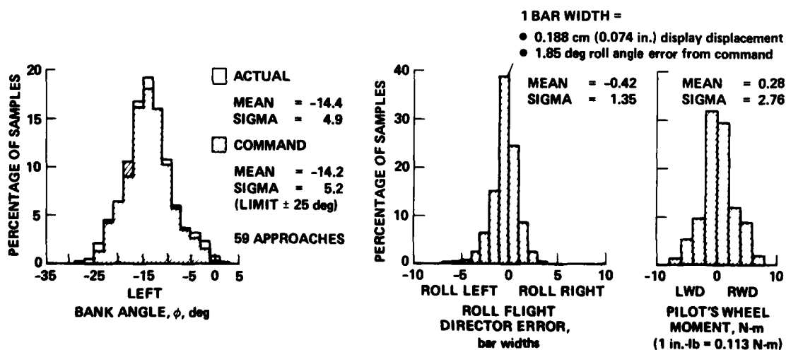
Figure 37.— Roll control utilization during turn segment.
