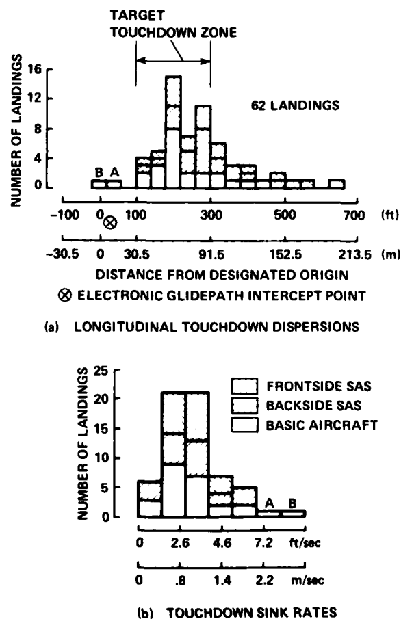
Figure 51.— Longitudinal touchdown performance.
