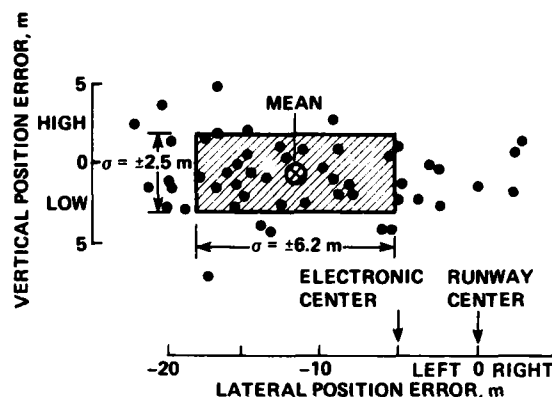
Figure 48.— Net position errors at pilot's decision height.
