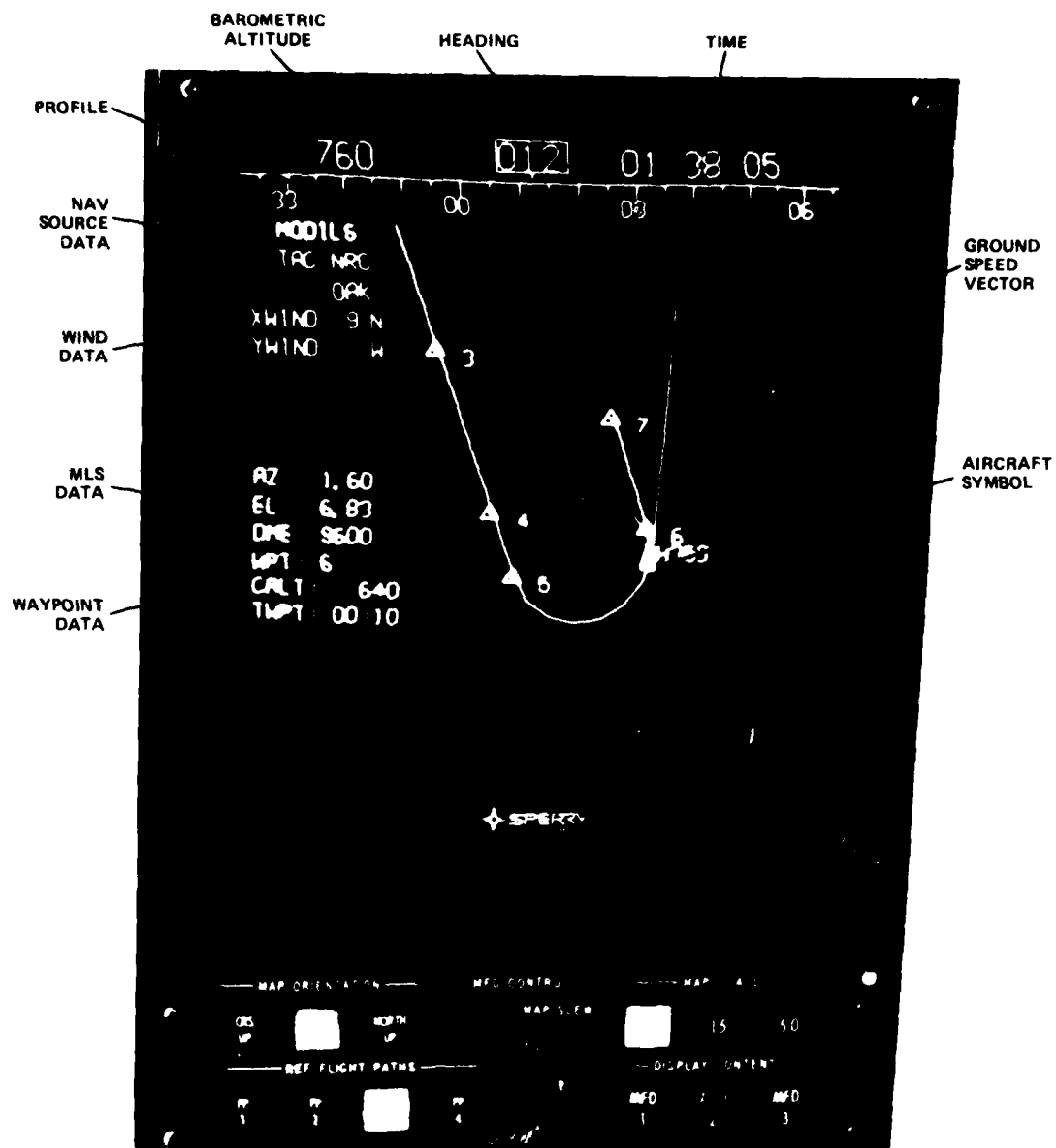
Figure 15.— Multifunction display.
