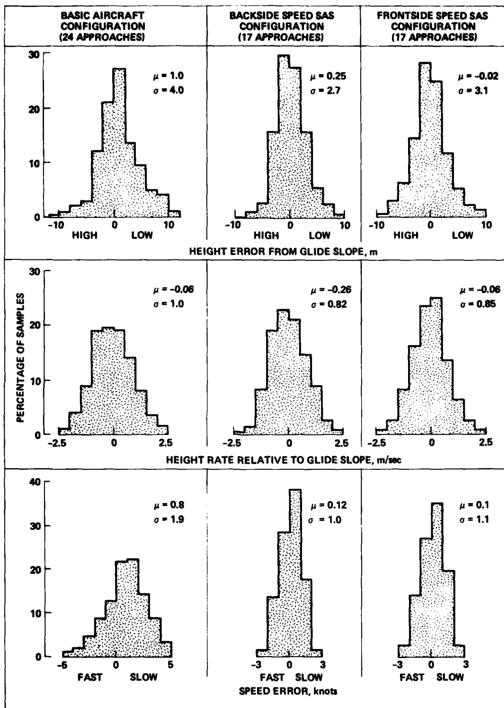
Figure 44.— Longitudinal performance measures during final straight segment.
