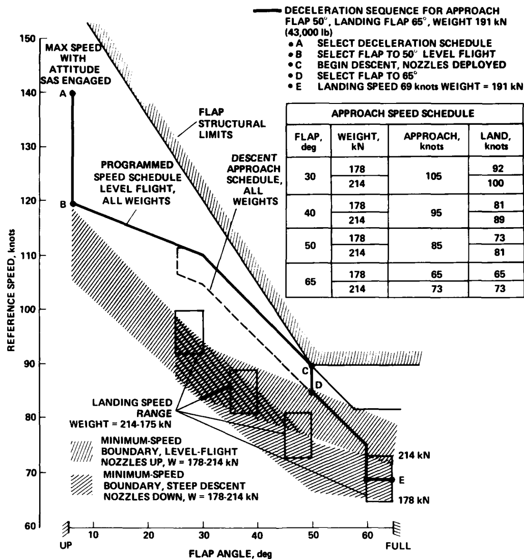
Figure 20. — Scheduling of the decelerating speed reference with flap and nozzle angles.
