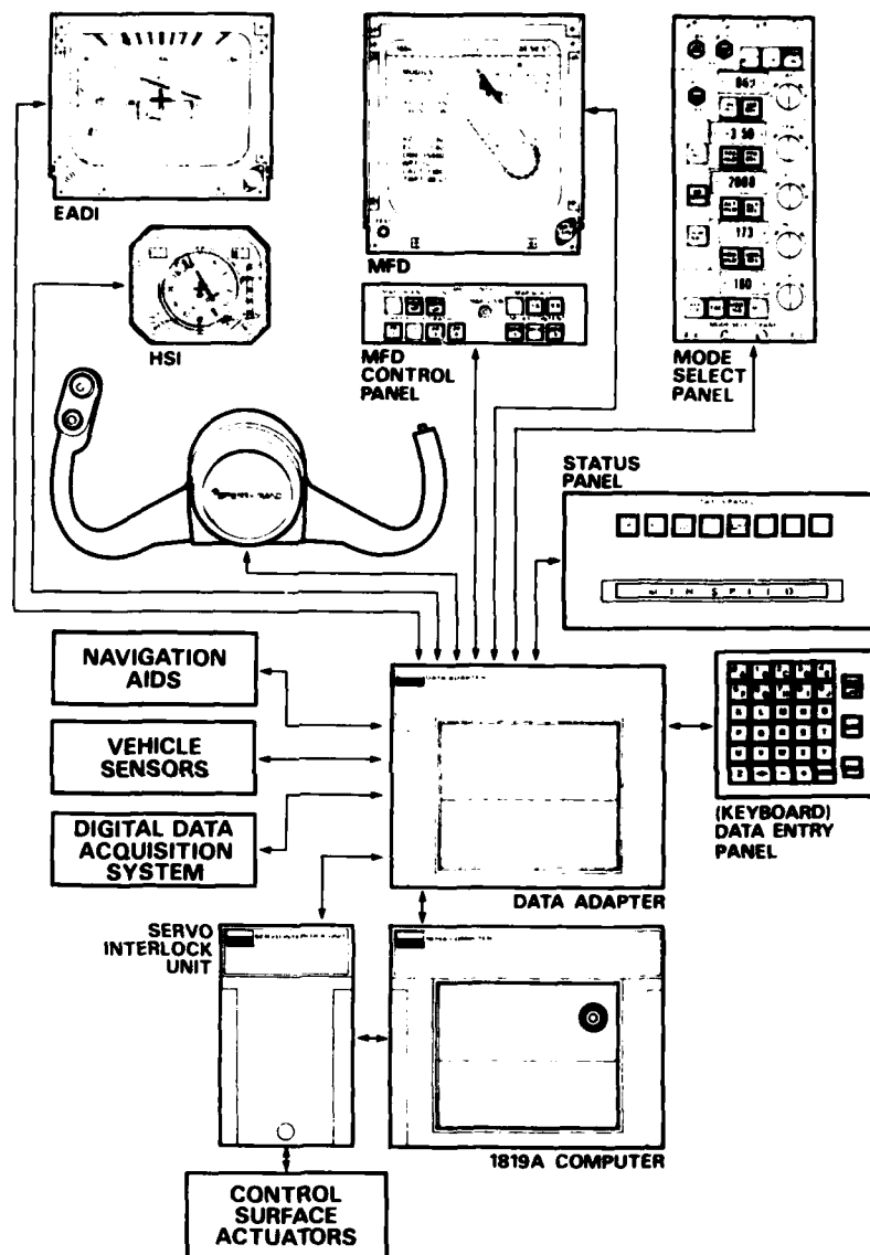
Figure 11.— STOLAND research avionics system.
