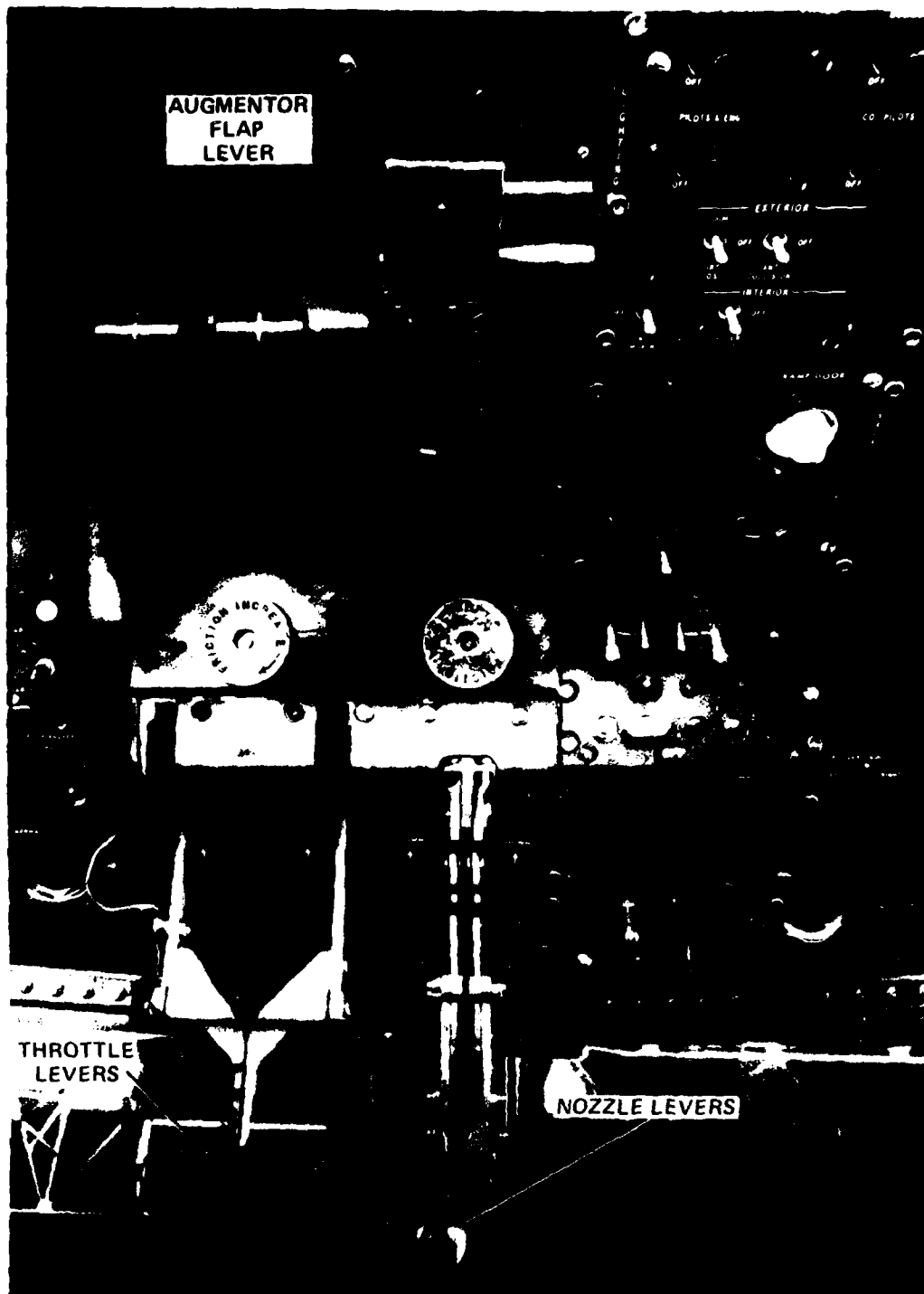
Figure 4. Overhead propulsion system controls.
