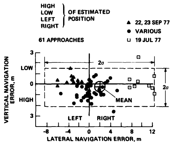
Figure 41. — Navigation errors at decision range plane.
