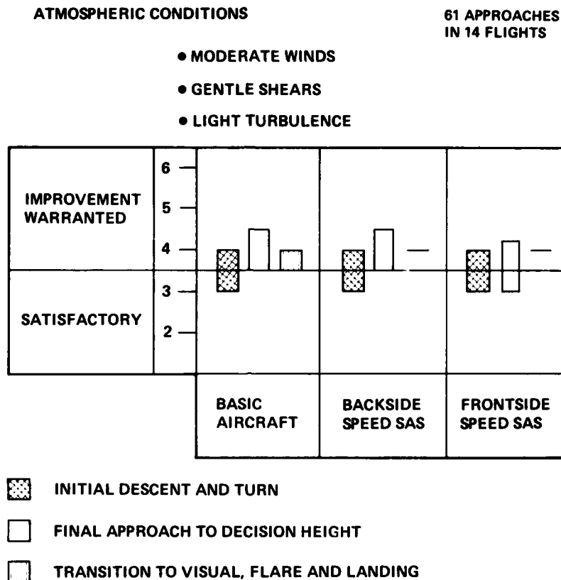
Figure 55. — Range of pilot ratings assigned to three segments of the decelerating curved approach task.
