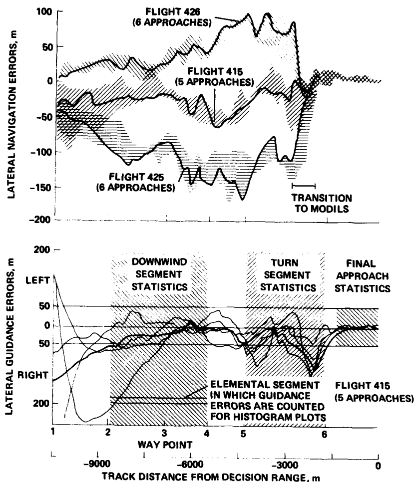
Figure 30.— Typical crosstrack navigation and guidance errors.
