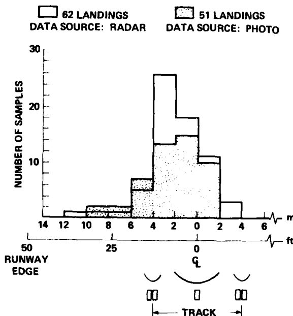
Figure 53.— Lateral touchdown dispersion.
