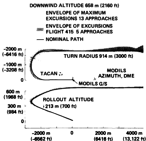
Figure 29.— Envelope of approach performance, flightpath 2.
