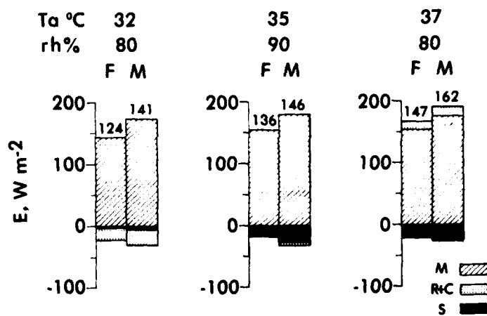
Figure 2. Comparison of mean evaporative heat loss ( E ), ( E = M + (R + C) - S ) between males (M) and females (F) in three hot-wet conditions (32 °C, 80% rh; 35 °C, 90% rh; 37 °C, 80% rh). The numbers at the top of each column represent the E values. The areas ( R + C and S ) above and below the zero point represent whether these values are to be added or subtracted from M .
