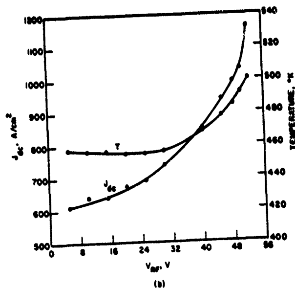
FIG. 50 LARGE-SIGNAL RESULTS FOR THE DIODE OF FIG. 15a WITH f = 10 \text{ GHz} , V_{dc} = 66.1 \text{ V} AND R_{TH} = 3.963 \times 10^{-3} \text{ (}^\circ\text{K-cm}^2/\text{W)} .
