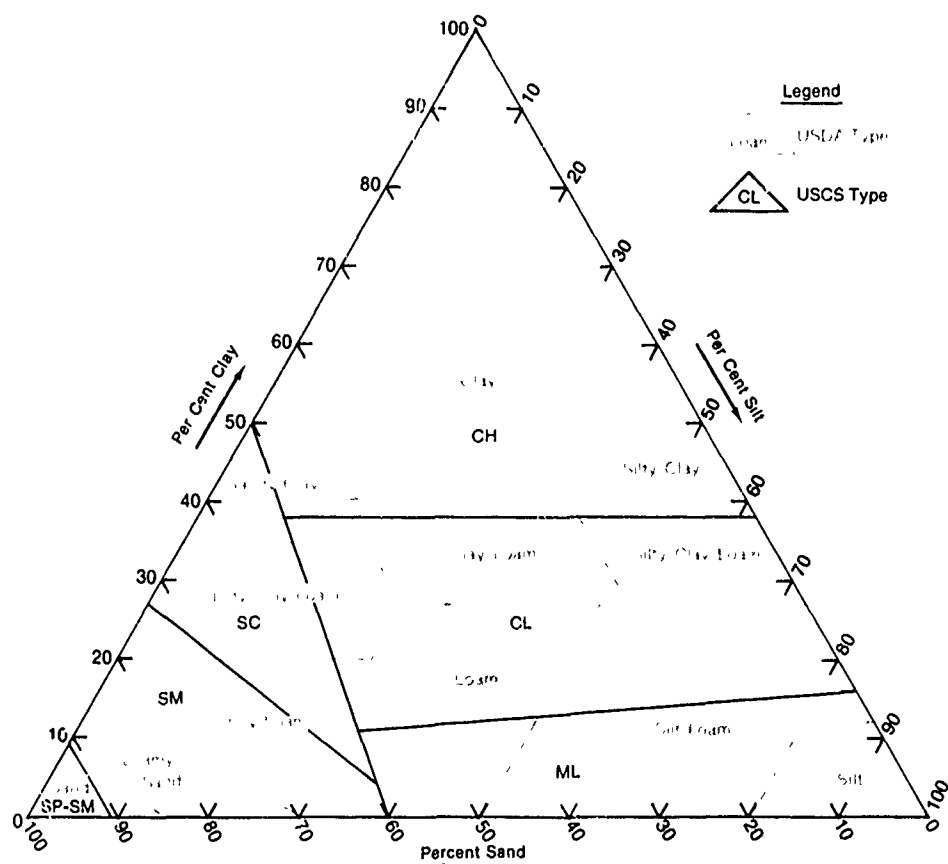
Figure 16. Guide for Comparing USDA and USCS Soil Types (Source: Trafficability of Soils, Soil Classification: TM 3-240; Waterways Experiment Station; 1961.)
