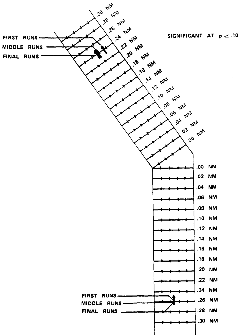
FIGURE 12. TRACKKEEPING BY ORDER OF RUN 0.25 NM BEFORE AND BEYOND BEND
