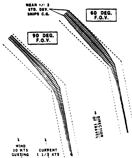
FIGURE 2. SUMMARY OF TRACKKEEPING BETWEEN PERSPECTIVE DISPLAYS
