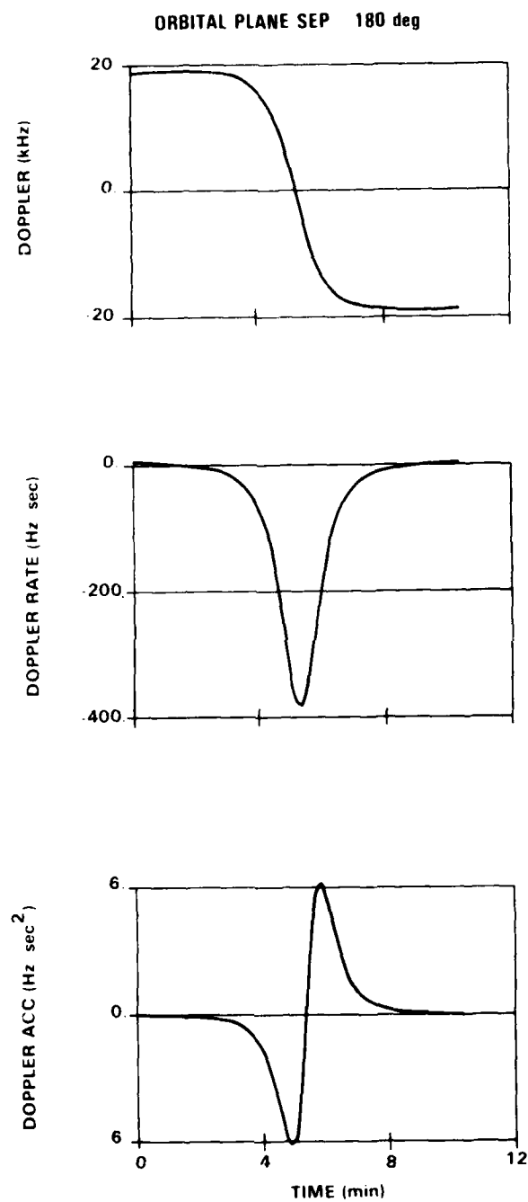
Figure 1. Worst-case Signal Dynamics
