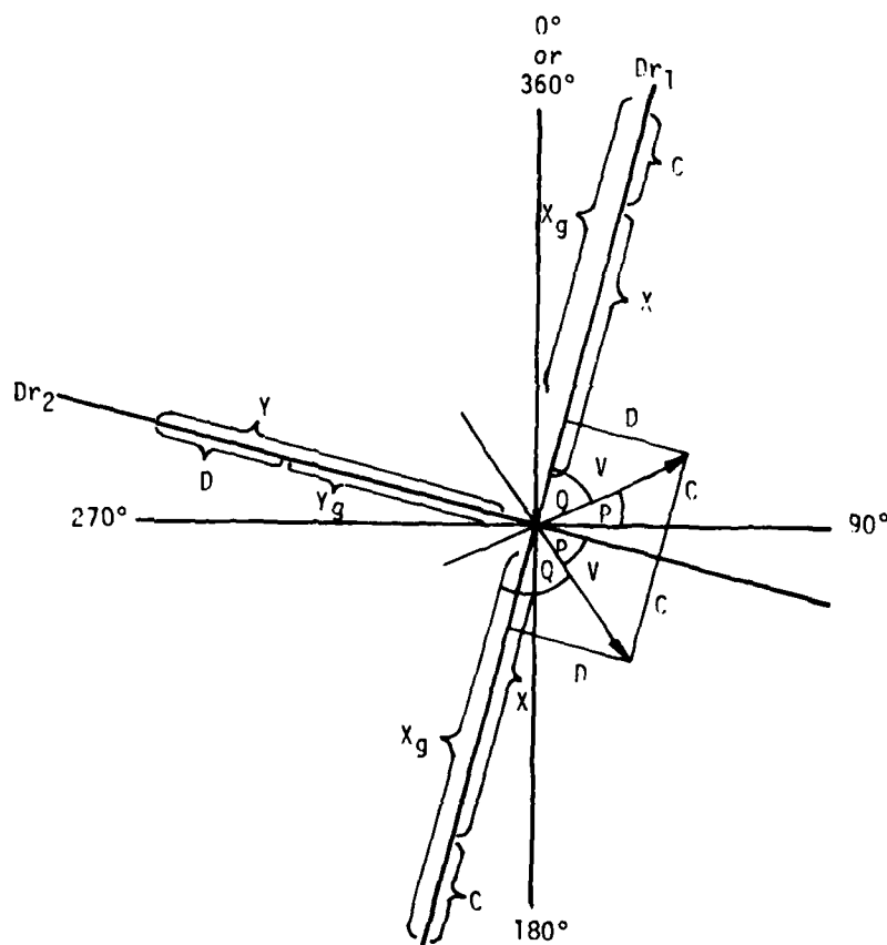
Figure 12. Use of method 1 to compute wind velocity. Variables are explained in figure 2 and first technique. Only Dr_2 is known, and C > 0 and D < 0 . Two values of Dr_1 , X , X_g , V , P , Q , C , and D are shown because Dr_1 may be 15^\circ or 195^\circ . Two wind velocities ( V ) are computed.
