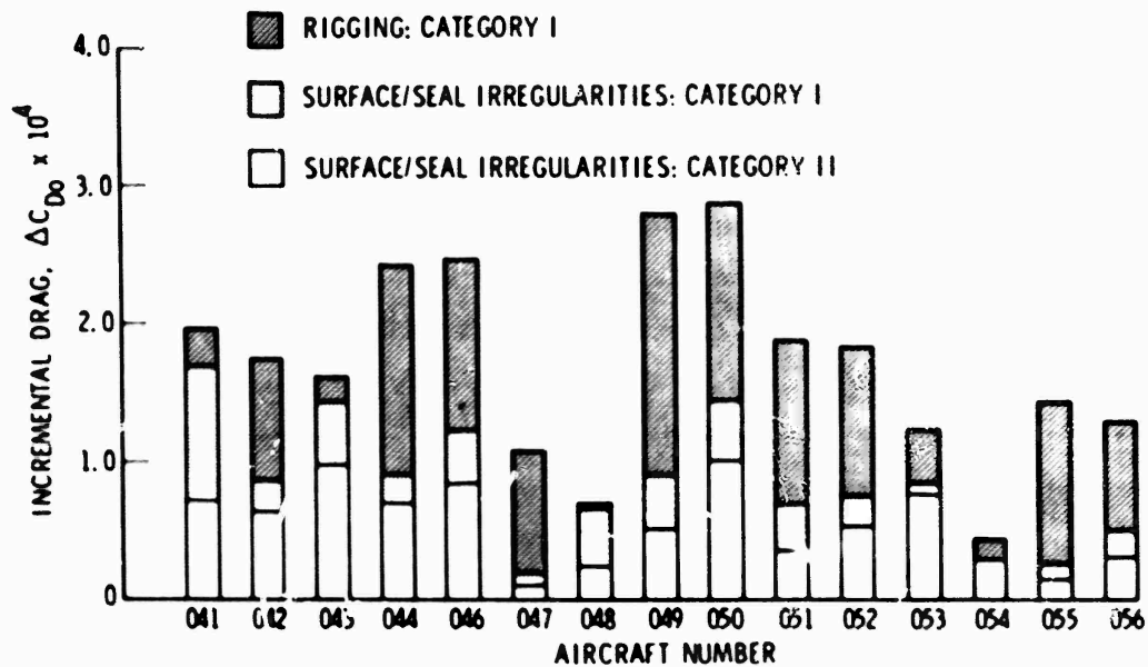
Figure 5. DC-10-10 Incremental Drag Summary
