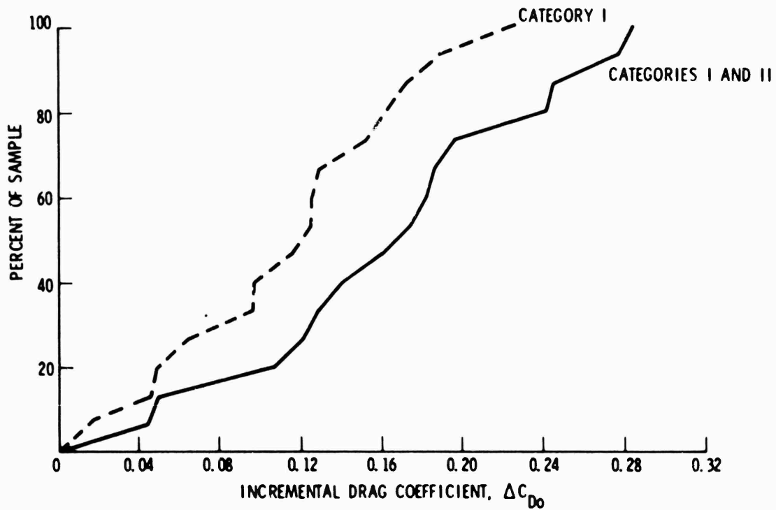
Figure 8. DC-10-10 Cumulative Distribution of \Delta C_{Do}
