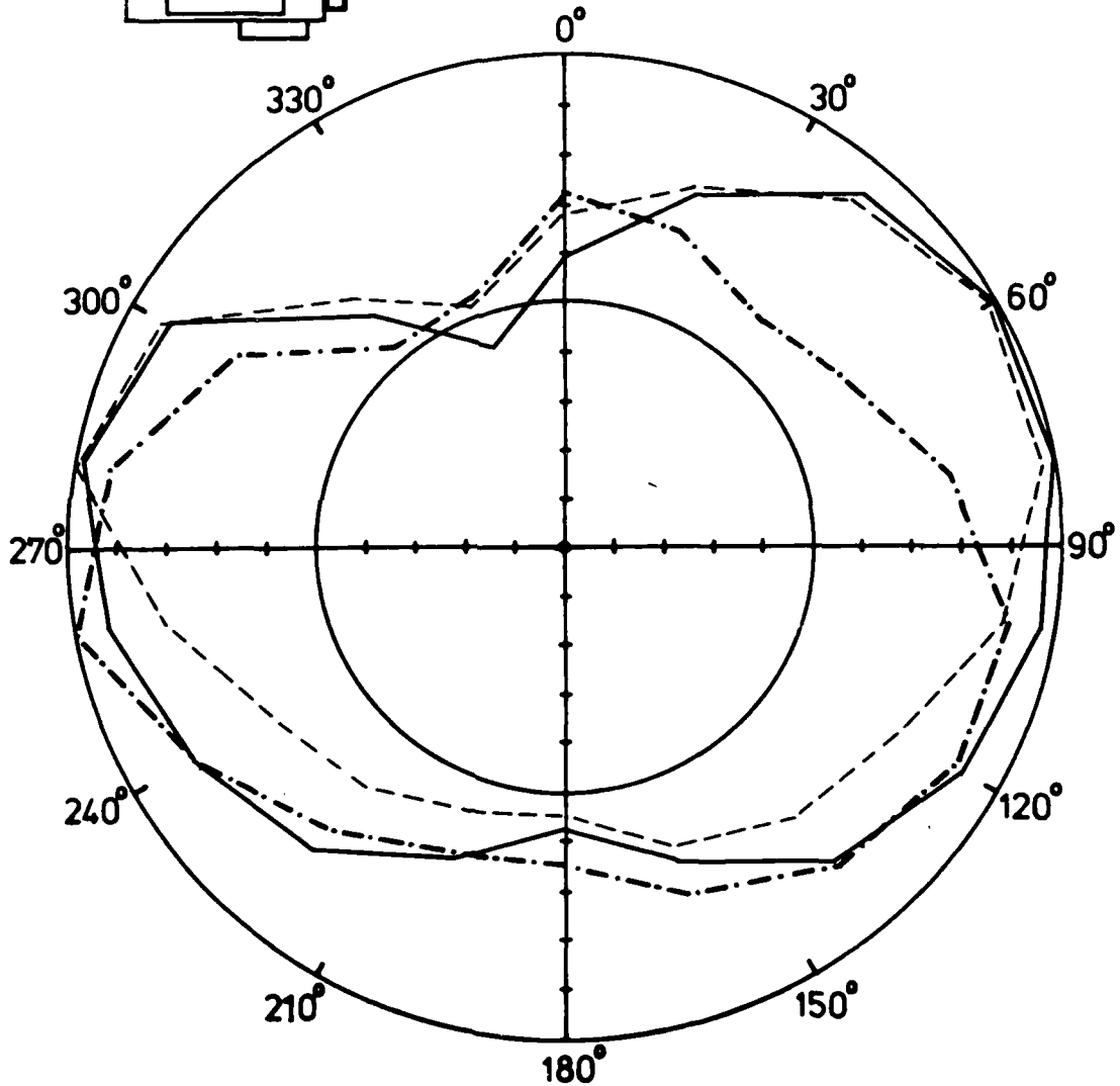
Fig. 19: Receiving pattern of antenna 2 for f = 70/75/80 MHz. Roof not mounted. (Antenna configuration as in Fig. 10)
