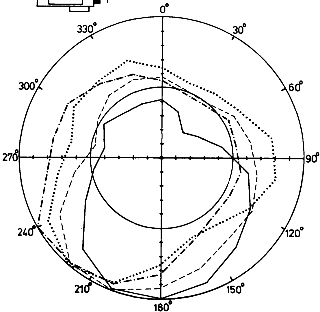
Fig. 37: Receiving pattern of antenna 1 for f = 30/34/40/44 MHz. Roof not mounted. (Antenna configuration as in Fig. 36)
