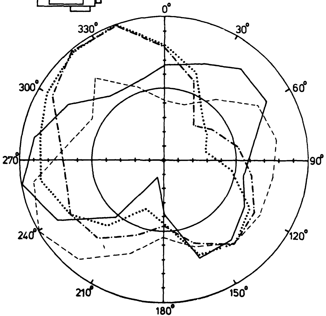
Fig. 20: Receiving pattern of antenna 6 for f = 30/35/40/45 MHz. Roof not mounted. (Antenna configuration as in Fig. 10)
