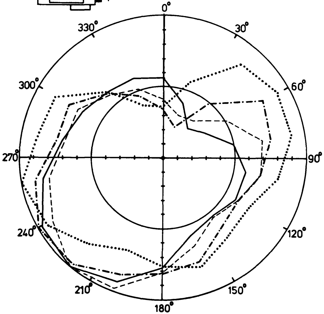
Fig. 12: Receiving pattern of antenna 1 for f = 50/55/60/65 MHz. Roof not mounted. (Antenna configuration as in Fig. 10)
