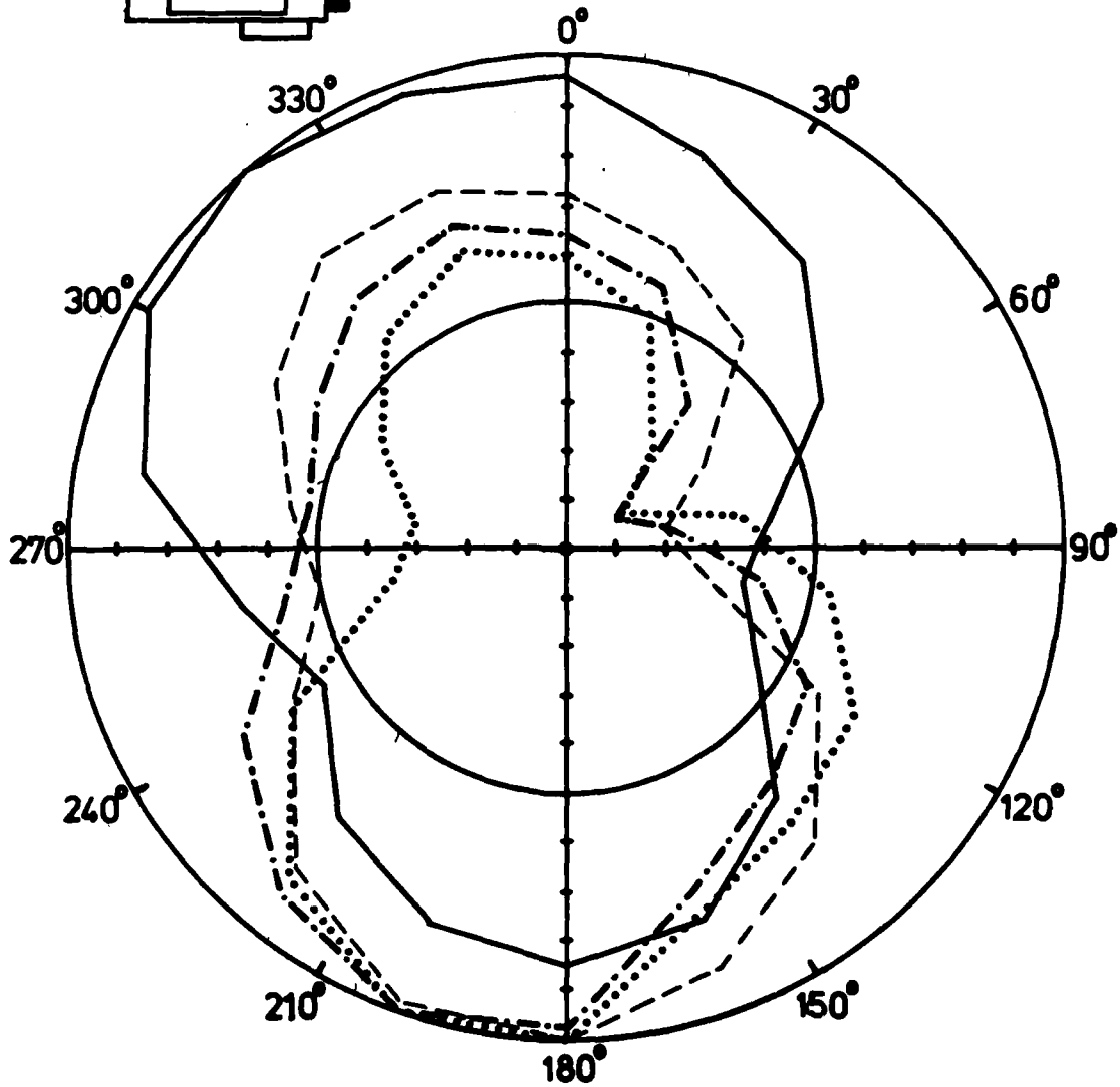
Fig. 56: Receiving pattern of a bent-down rod antenna. f = 30/35/40/45 MHz.
