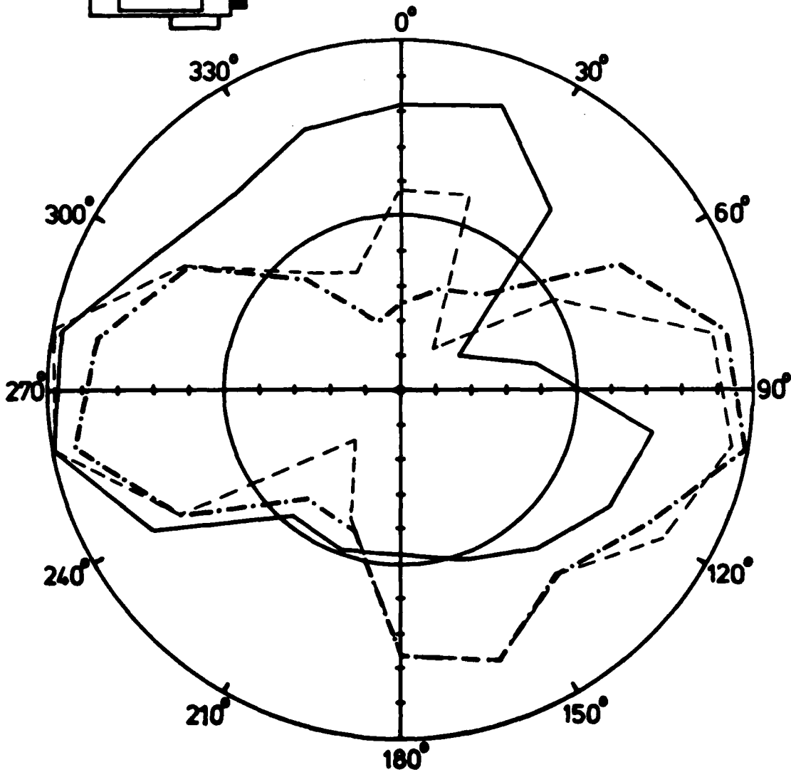
Fig. 58: Receiving pattern of a bent-down rod antenna. f = 70/75/80 MHz.
