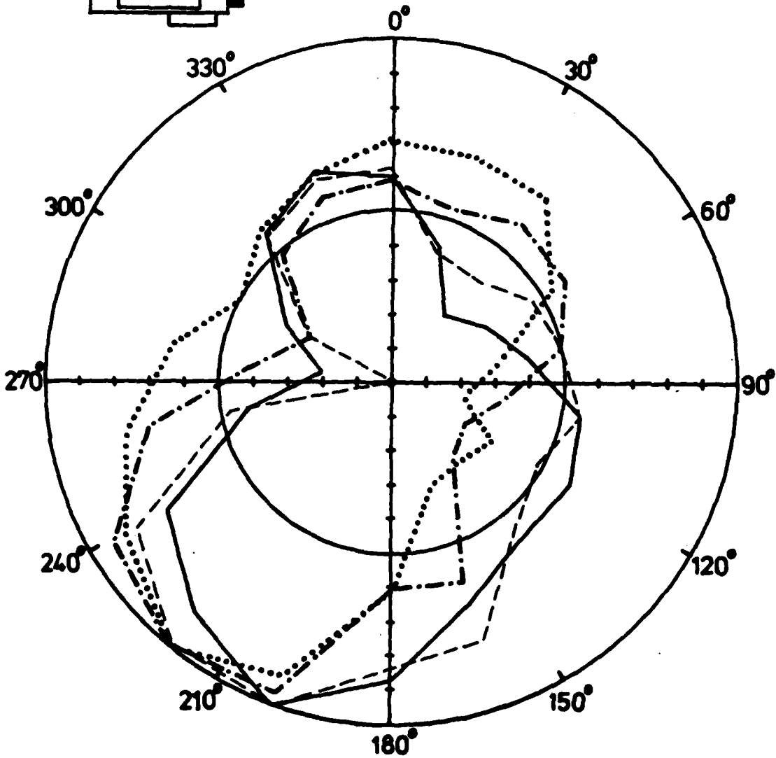
Fig. 57: Receiving pattern of a bent-down rod antenna. f = 50/55/60/65 MHz.
