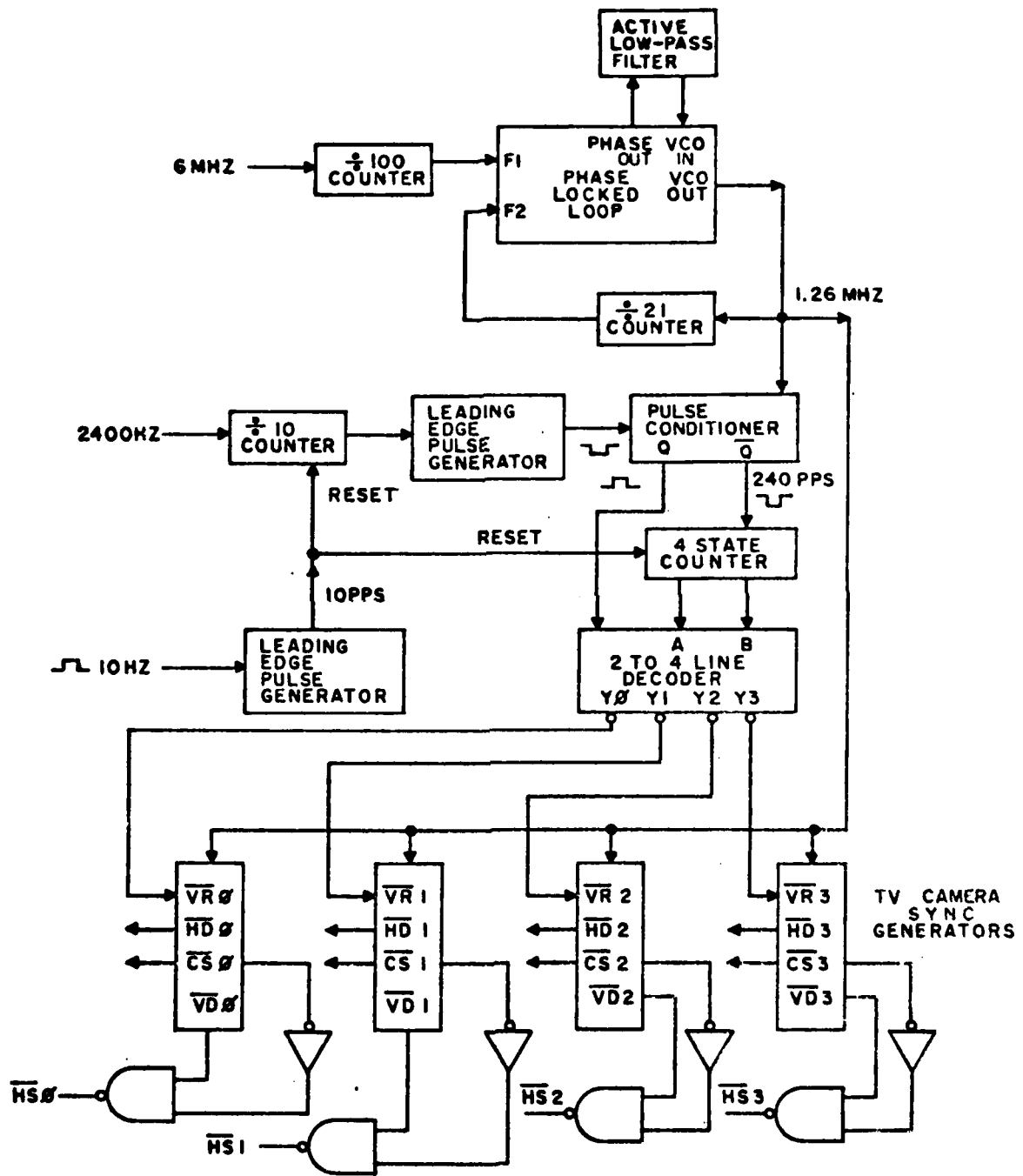
Figure 3. Video synchronizer.
