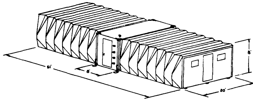
Figure 16. Expandable 50-ft ISO shelter tested at CRTC 1974-1975.
