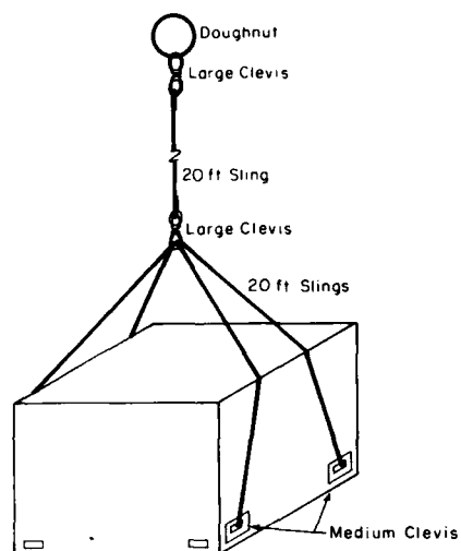
Figure 5. Sling rigging for the helicopter lift.
