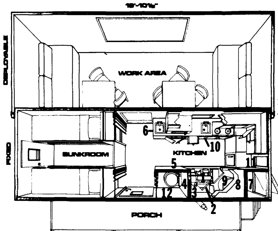
Figure 2. Equipment location.
