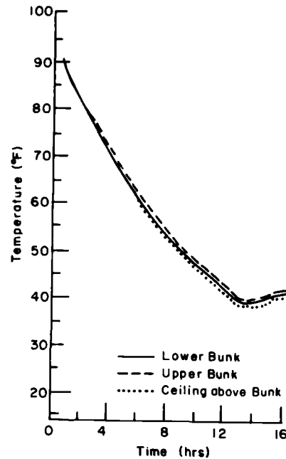
Figure 13. Rate of cooling inside the shelter with no heat input.
